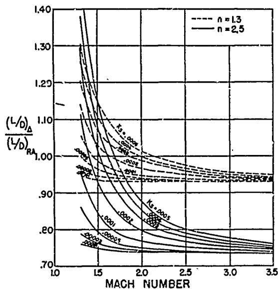
Fig. 7 RATIO OF MAXIMUM LIFT-DRAG RATIOS OF DELTA AND REVERSE ARROW WINGS
