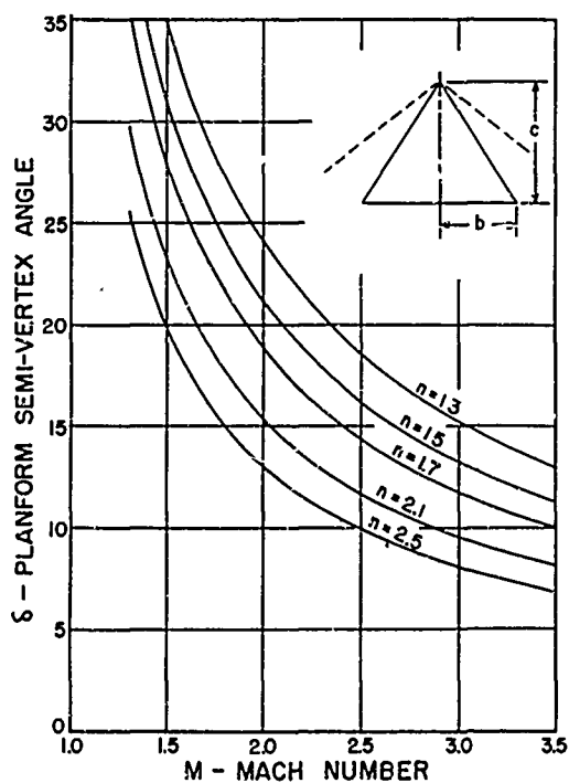
Fig. 9 PLANFORM SEMI-VERTEX ANGLE OF DELTA WINGS
