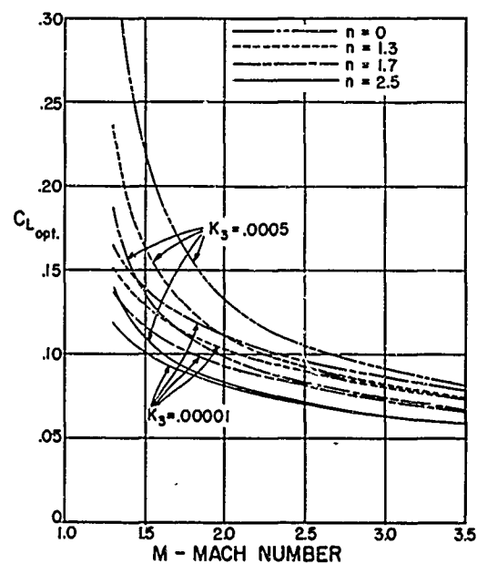
Fig. 10 OPTIMUM LIFT COEFFICIENT - DELTA WINGS
