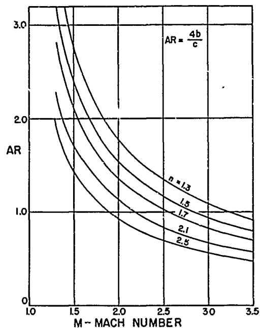
Fig. 8 ASPECT RATIO OF DELTA WINGS
