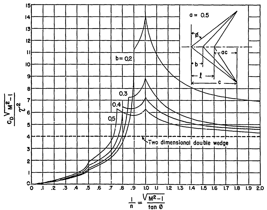
Fig. 16 Δ-WING DRAG-SWEPT TRAILING EDGE
