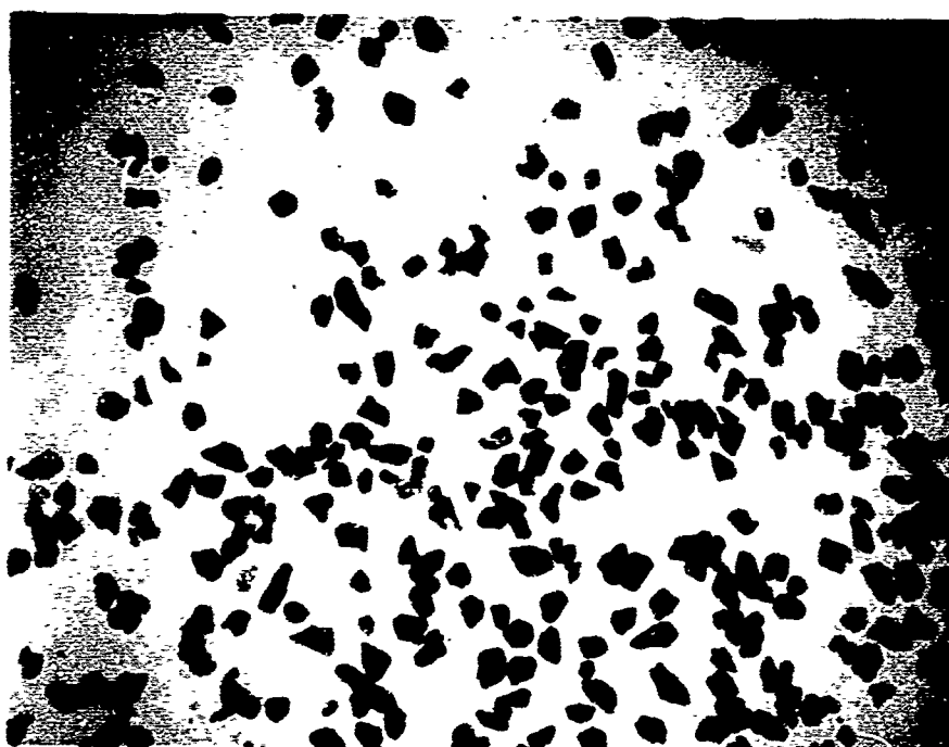
FALLOUT PARTICLES FROM AN ERUPTION OF VOLCANO IRAZU
