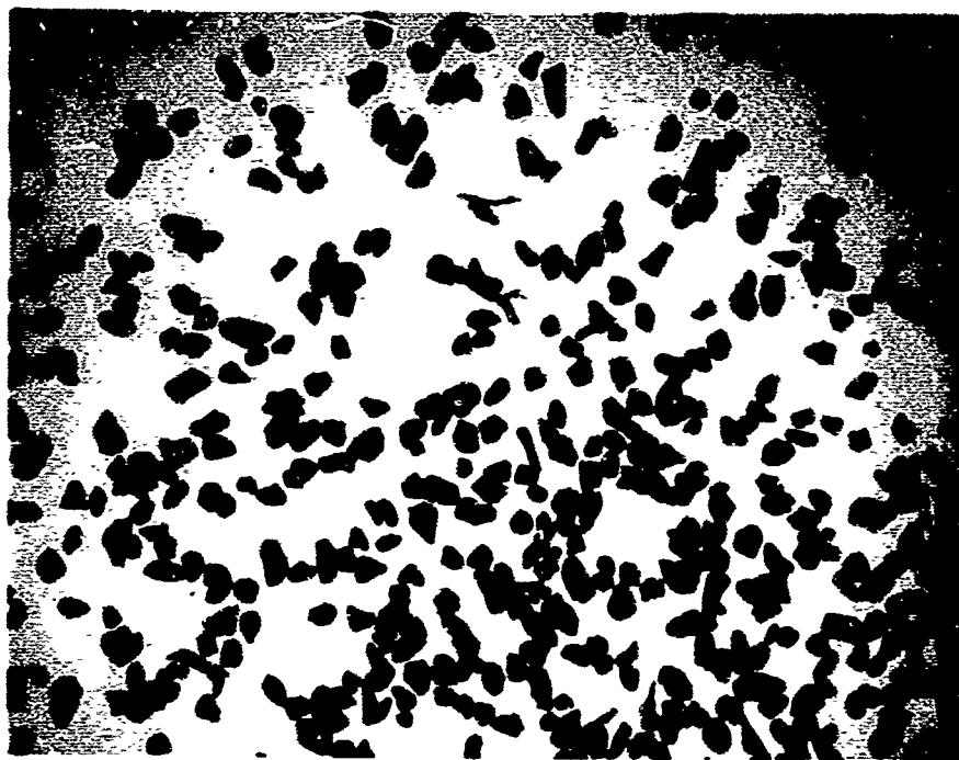
FALLOUT PARTICLES FROM A LOW-YIELD NEAR-SURFACE NUCLEAR DETONATION
