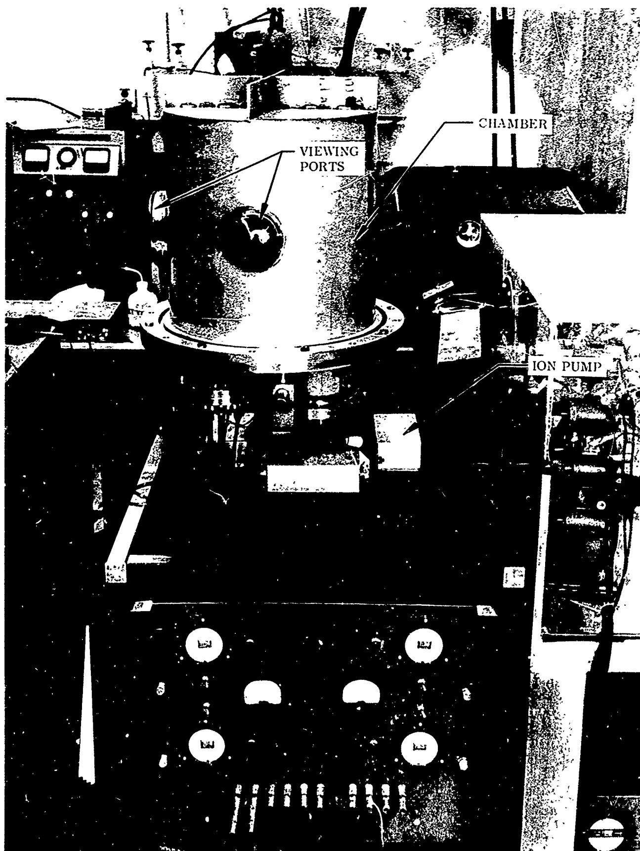
Fig. 1-7 Test Chamber With Ion Pump
