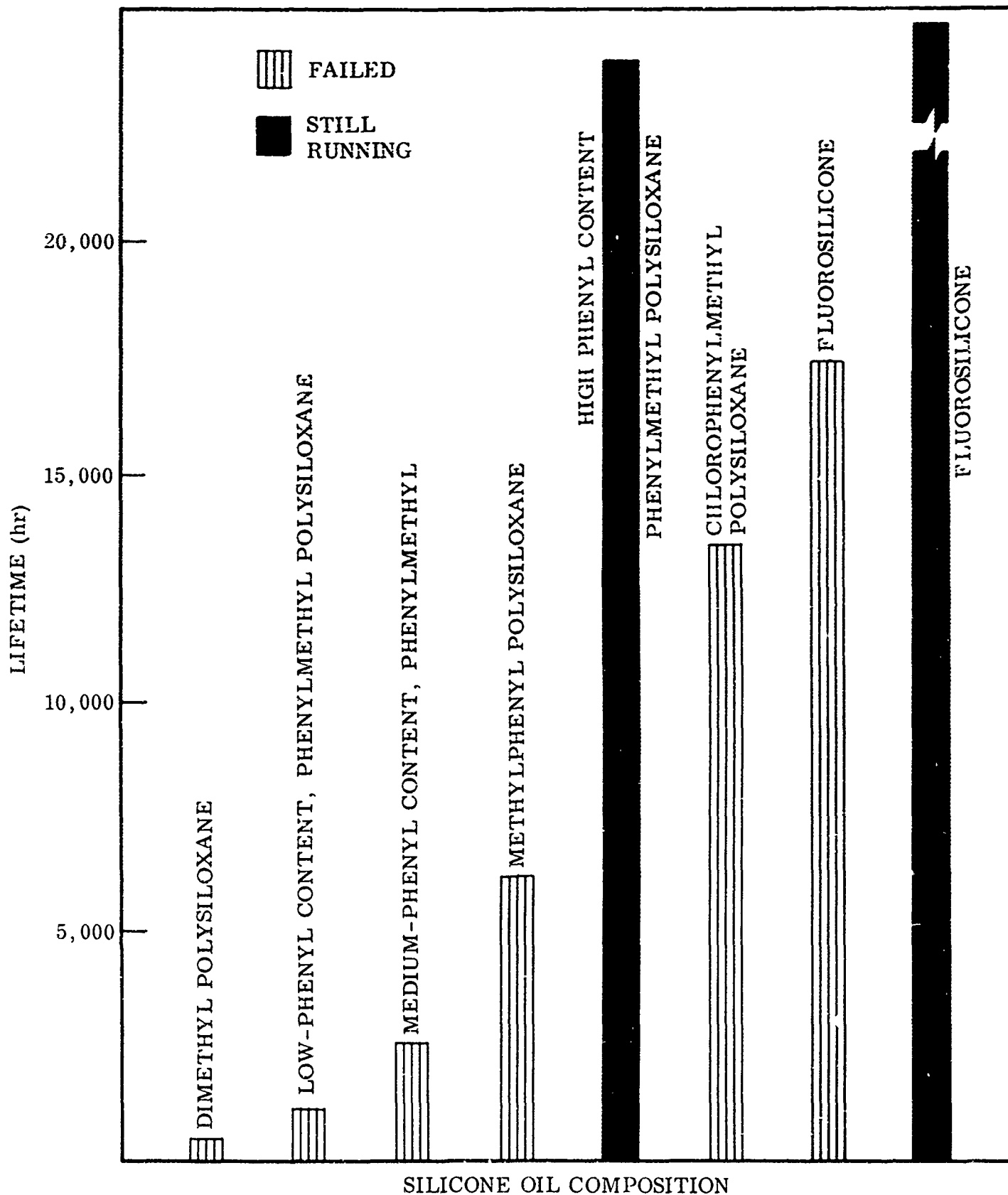
Fig. 1-15 Effect of Silicone Oil Composition on Bearing Lifetime in Vacuum
