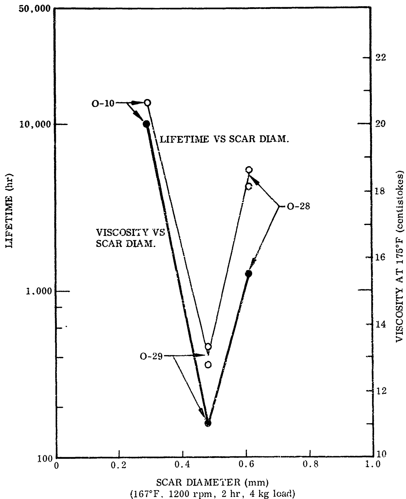
Fig. 1-16 Relationships Between Oil Lubricity (as Measured by Scar Diameter), Lifetime, and Viscosity
