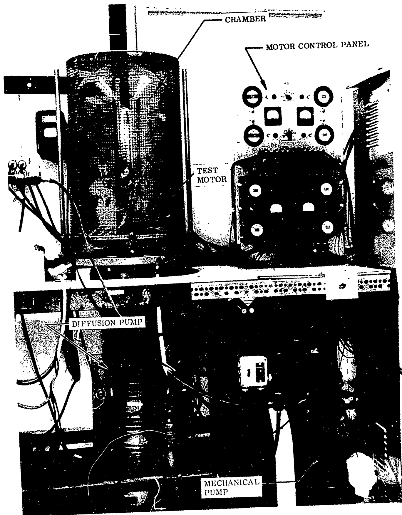
Fig. 1-6 Test Chamber With Oil Diffusion Pump
