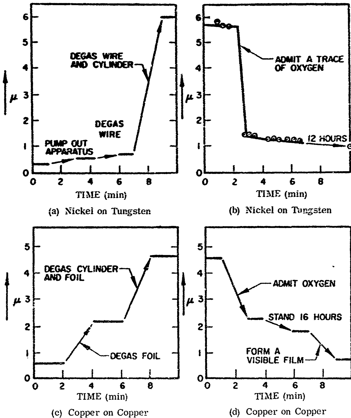
(a), (c) Effect of Removing Adsorbed Film of Oxygen and Other Contaminants From Metal Surfaces (b), (d) Effect of Adding a Trace of Oxygen to Clean Outgassed Metals
