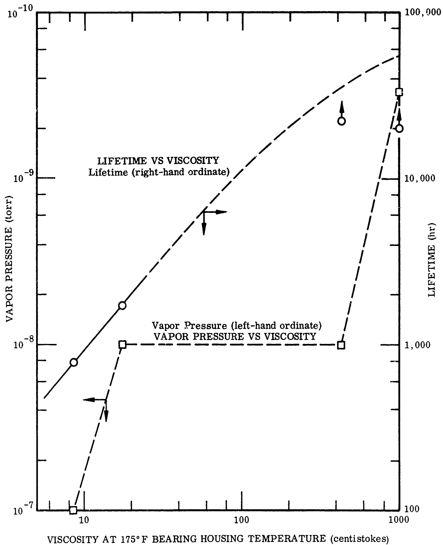
Fig. 1-14 Variation of Vapor Pressure and Lubricating Lifetime With Viscosity of Selected Mineral Oils
