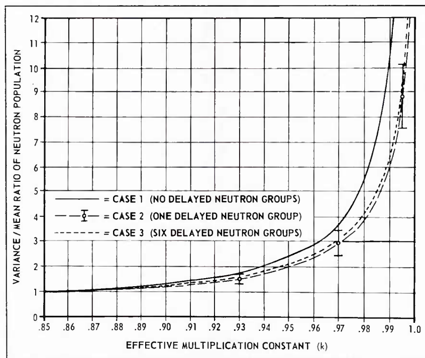
Figure 2. Theoretical variance/mean ratio of the neutron population in the subcritical condition of the AFRRI-TRIGA Reactor.
