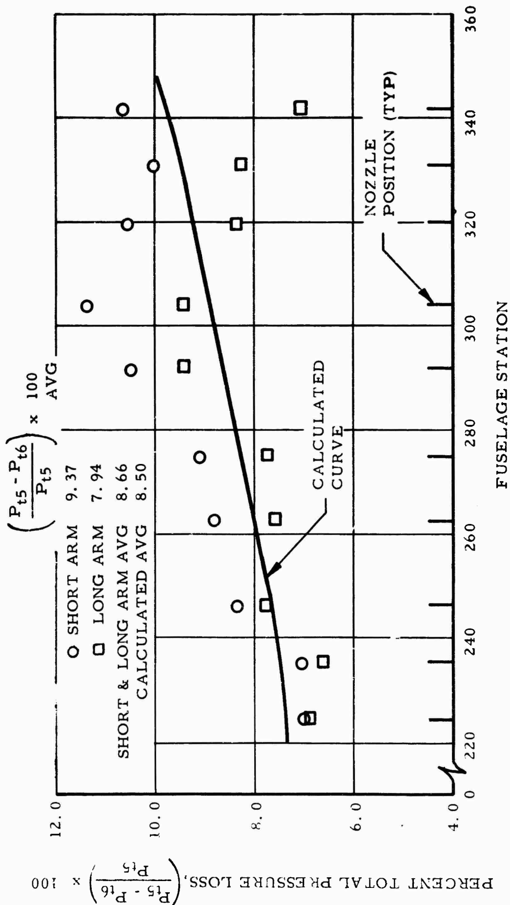
Figure 67. Engine Exit to F Manifold Nozzle Exit Total Pressure Loss Performance.
