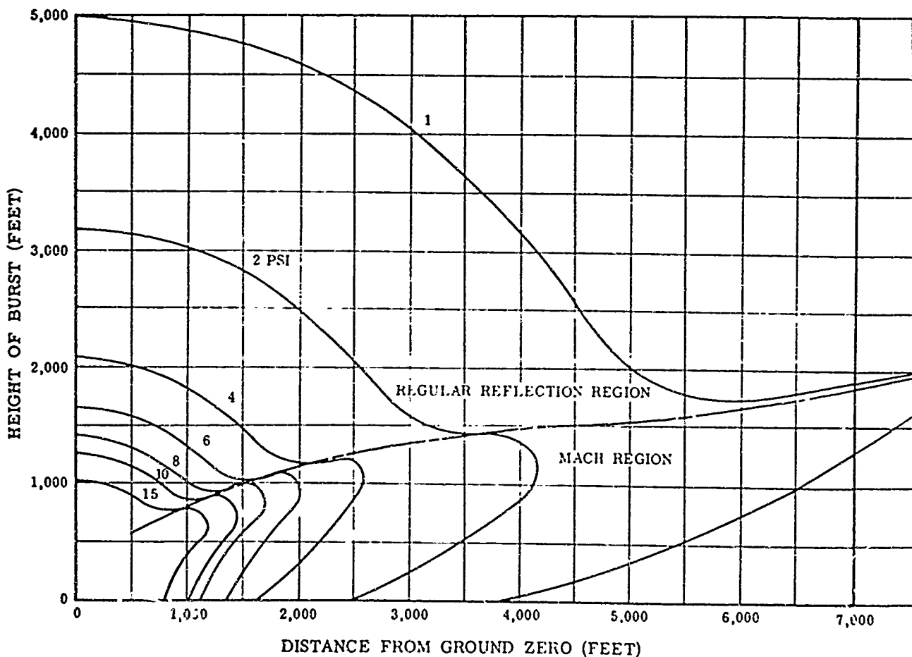
Fig. A-17. Peak Overpressures on the Ground for a 1-kt Burst
