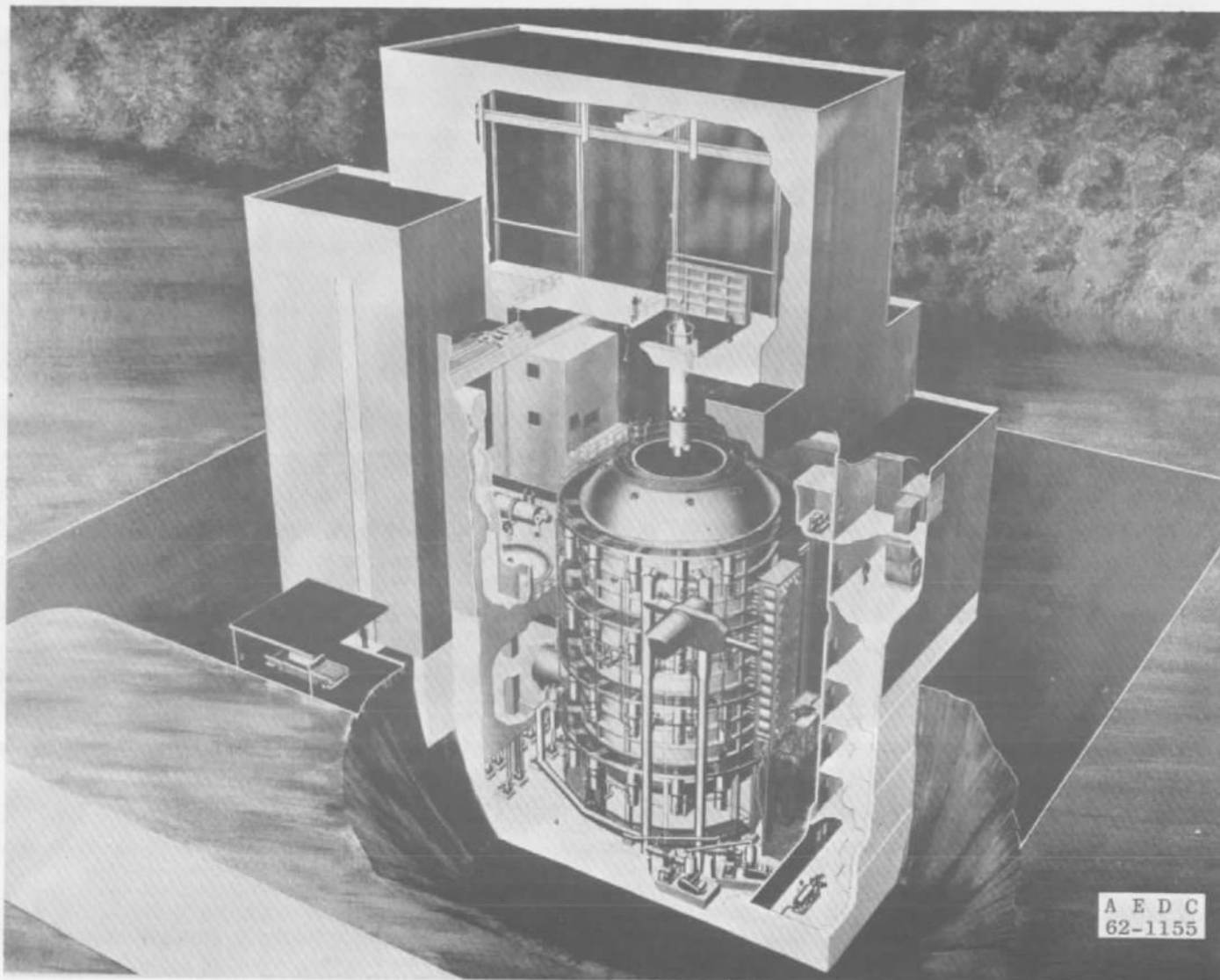
Fig. 2 Mark I Facility Arrangement
