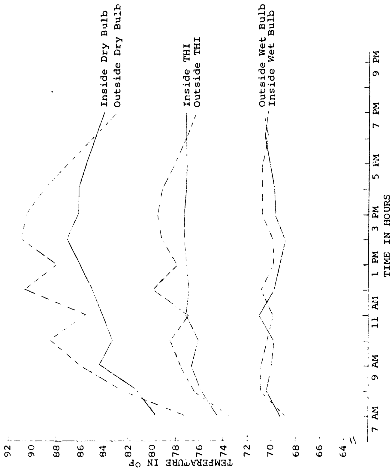
Figure D-5. Inside dry bulb, outside dry bulb, and THI temperatures by hour for June 23, 1968 (ES VII).
