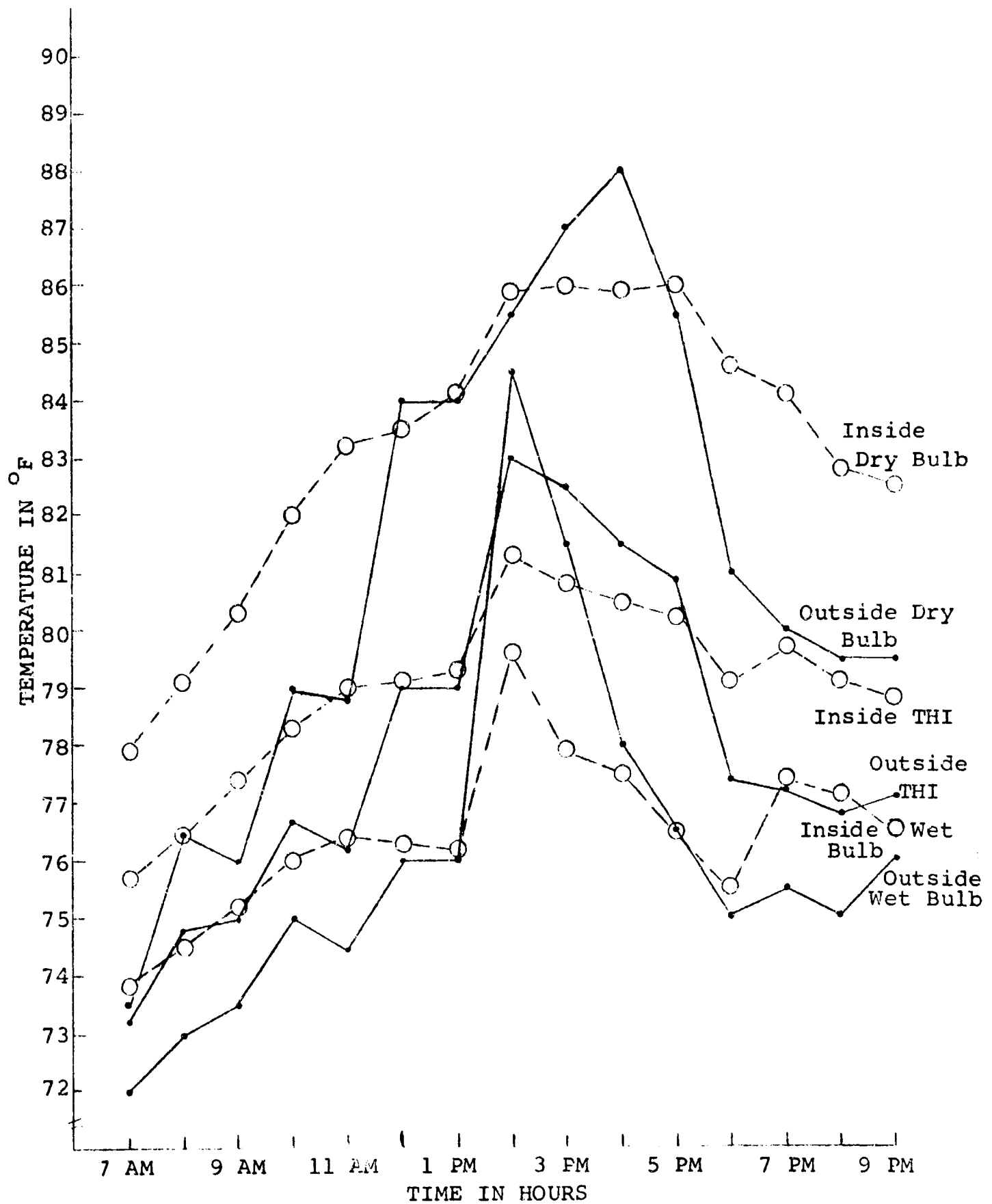
Figure D-9. Dry bulb, wet bulb, and THI temperatures by hour for September 11, 1965 (ES VIII).
