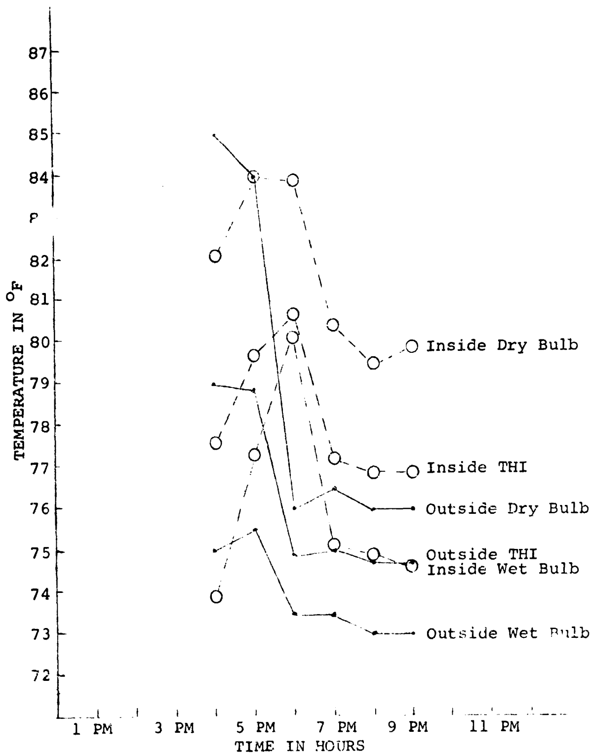
Figure D-8. Dry bulb, wet bulb, and THI temperatures by hour for September 10, 1965 (ES VIII).
