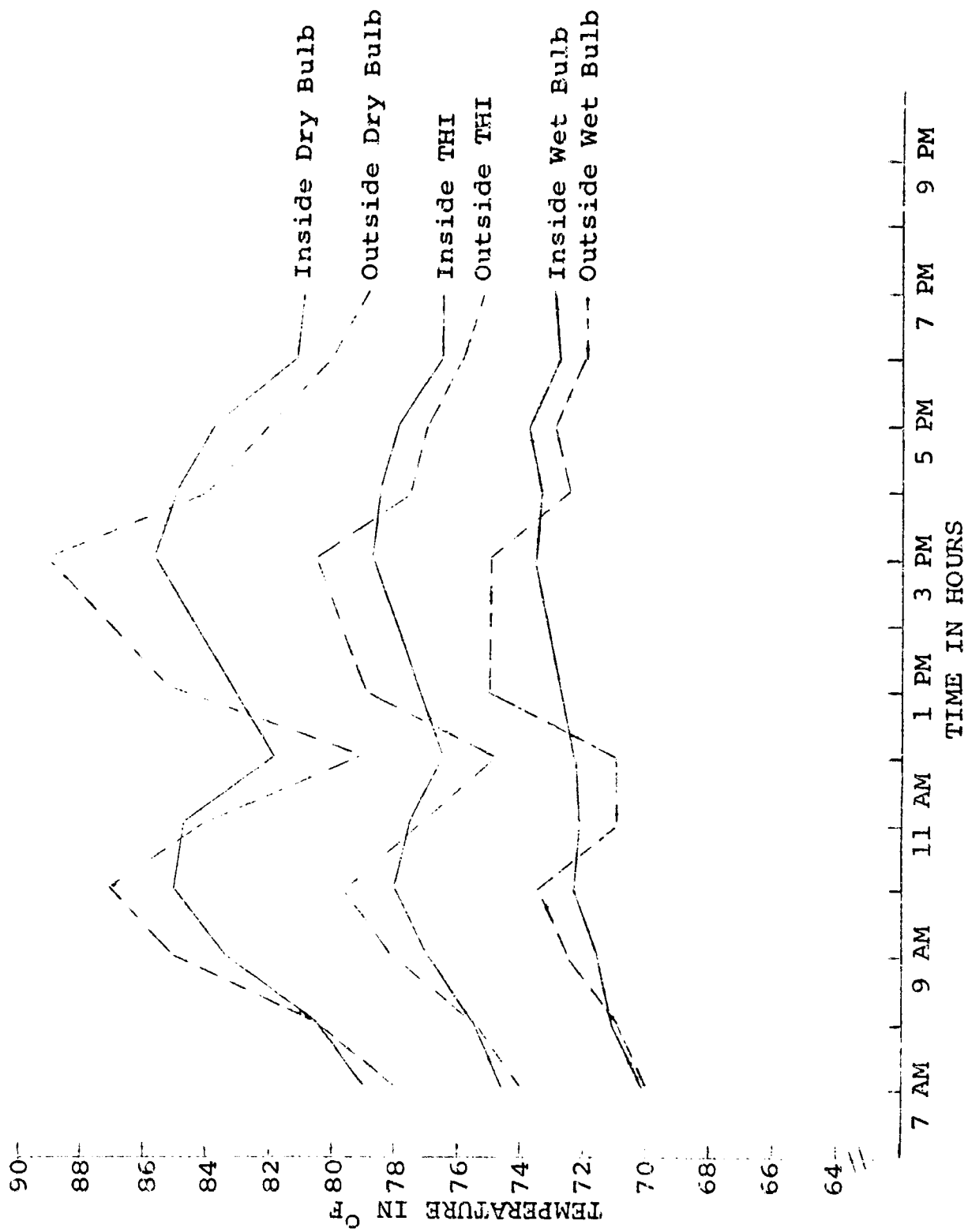
Figure D-6. Dry bulb, wet bulb, and THI temperatures by hour for June 24, 1965 (ES VII).
