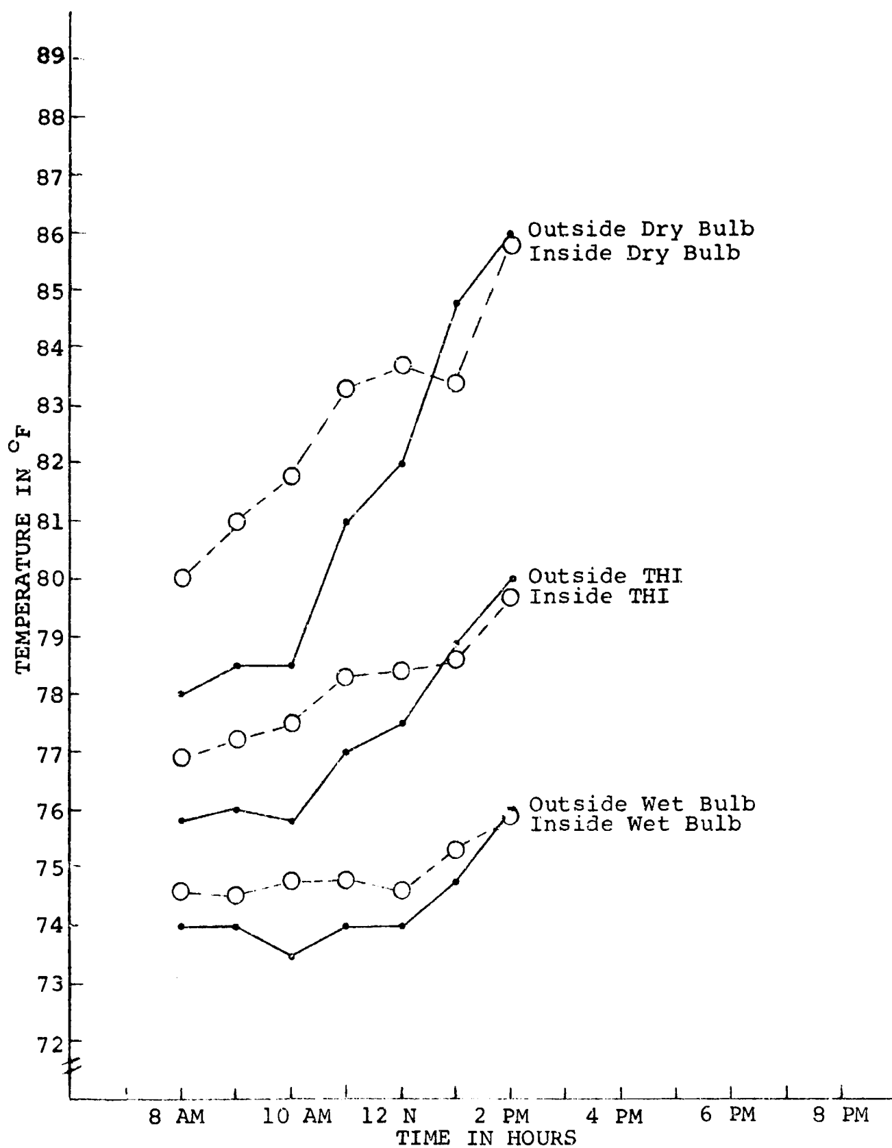
Figure D-10. Dry bulb, wet bulb, and THI temperatures by hour for September 12, 1965 (ES VIII).
