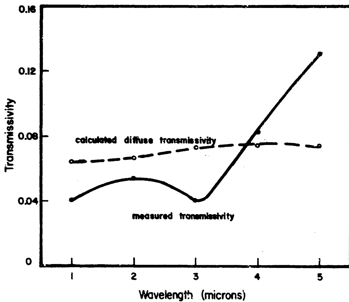
Figure 5.14 Measured and Calculated Transmissivity vs. Wavelength for \text{SrTiO}_3\text{A} .
