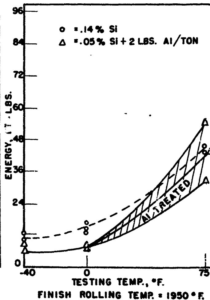
FIGURE 4. NOTCH TOUGHNESS CURVES ON HIGH-SILICON HULL PLATE STEEL HOT-ROLLED AT DIFFERENT TEMPERATURES
