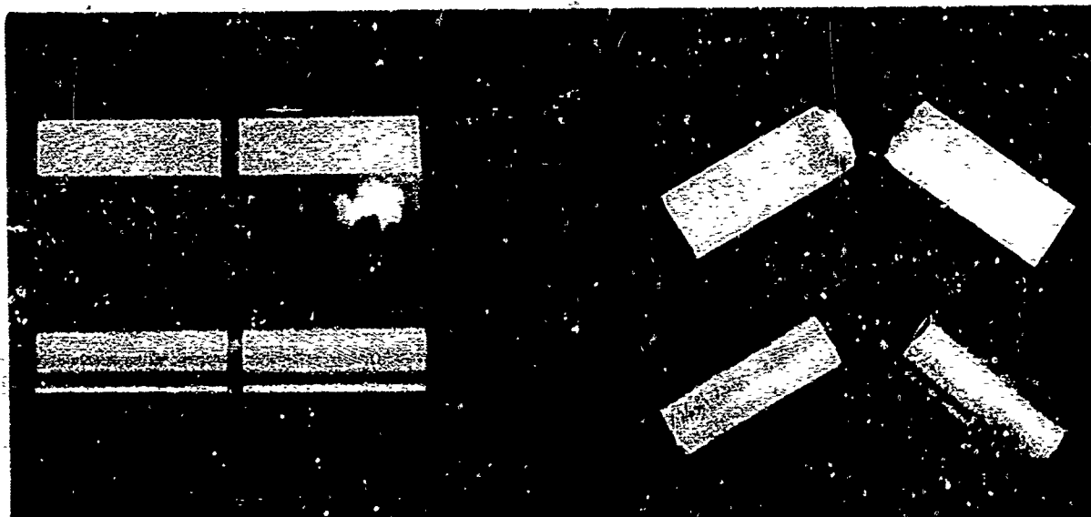
Figure 2. Photograph of V-Notch Charpy and round Charpy specimens before and after breaking.
