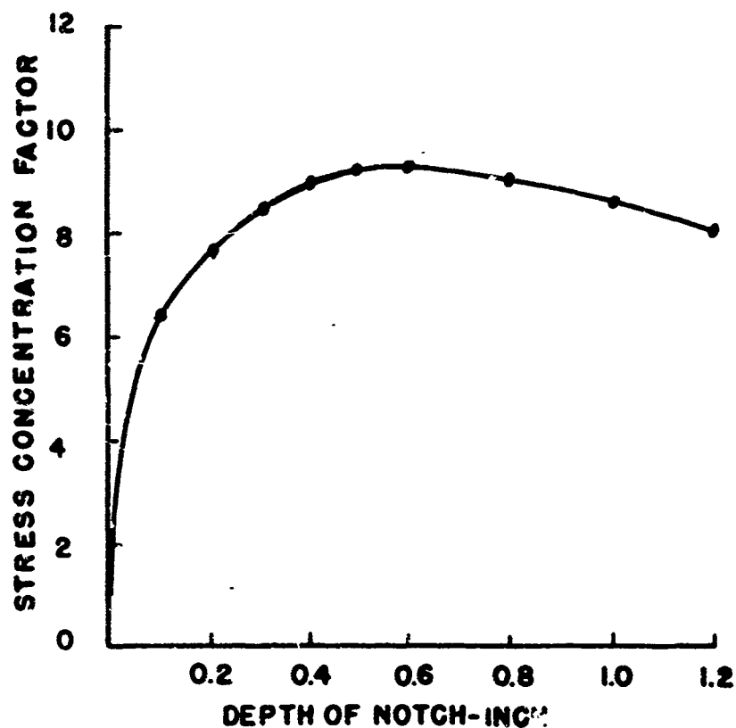
Figure 11. Variation in stress concentration as a function of notch depth for bar of indicated dimensions. (Calculation by L. R. Jackson, Applied Physics Division, Battelle Memorial Institute.)
