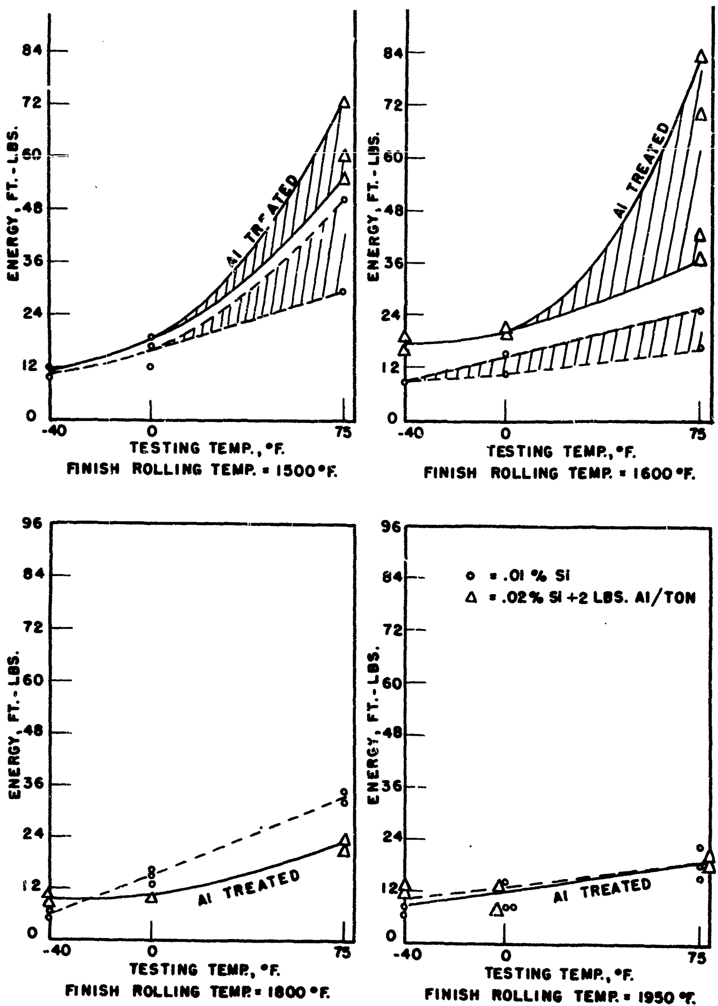
FIGURE 5 . NOTCH TOUGHNESS CURVES LOW-SILICON HULL PLATE STEEL HOT-ROLLED AT DIFFERENT TEMPERATURES
