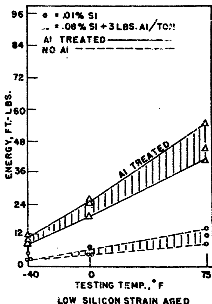
FIGURE 9, EFFECT OF STRAIN AGING UPON THE NOTCH TOUGHNESS OF HULL PLATE STEELS
