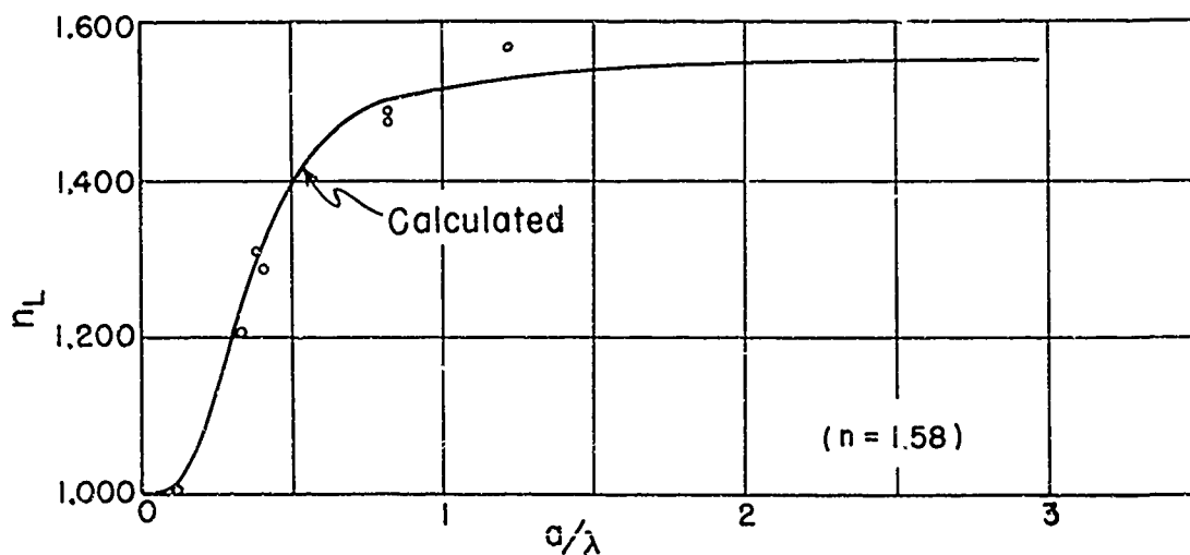
Fig. 8 EXPERIMENTAL VERIFICATION OF n_L - 1 = (n - 1)e^{-\left(\frac{\lambda}{\lambda_c}\right)^2}
