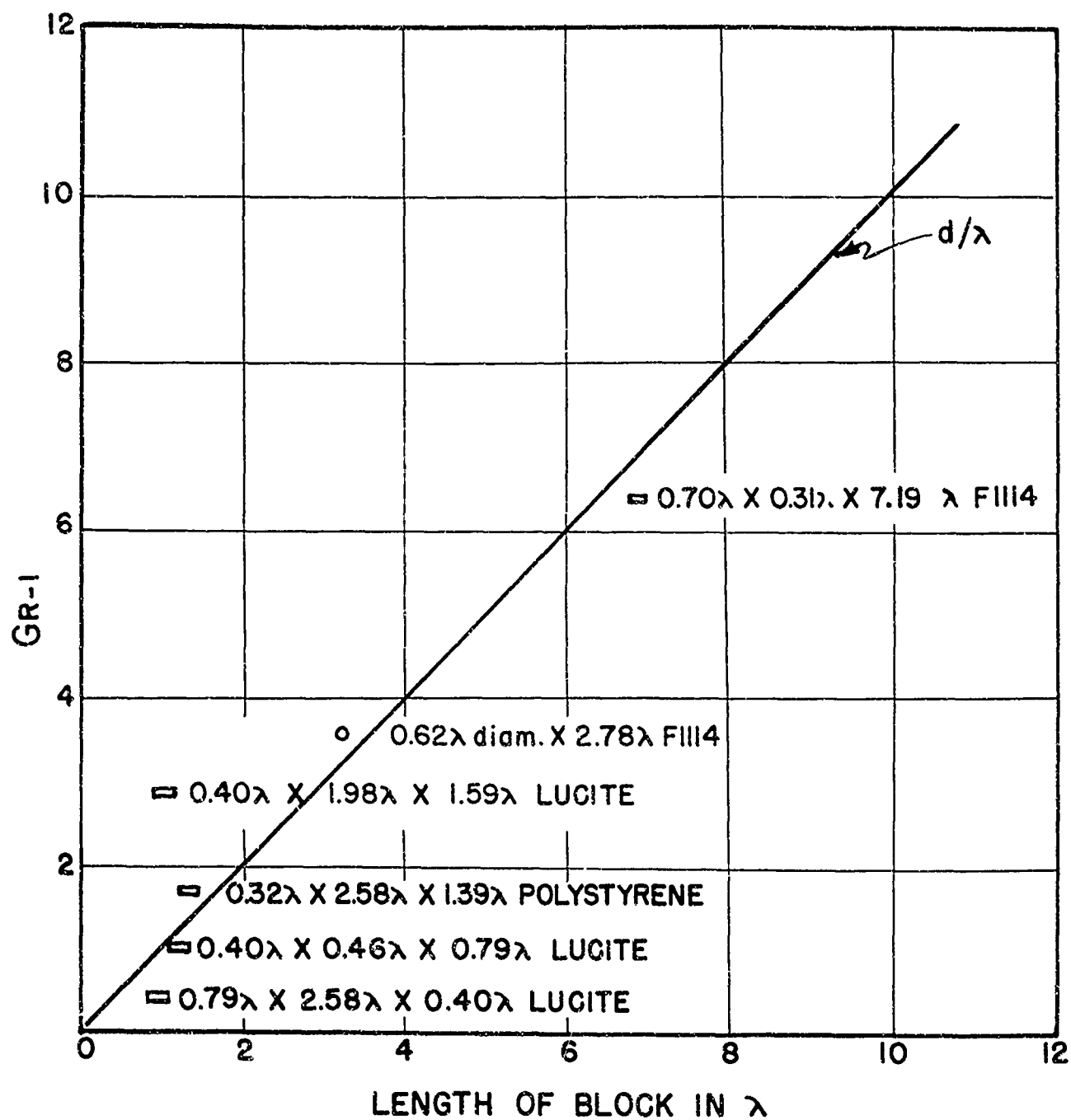
Fig. 5 RELATIVE MAXIMUM GAIN OF A LENS COMPARED TO METALLIC MOUTH
