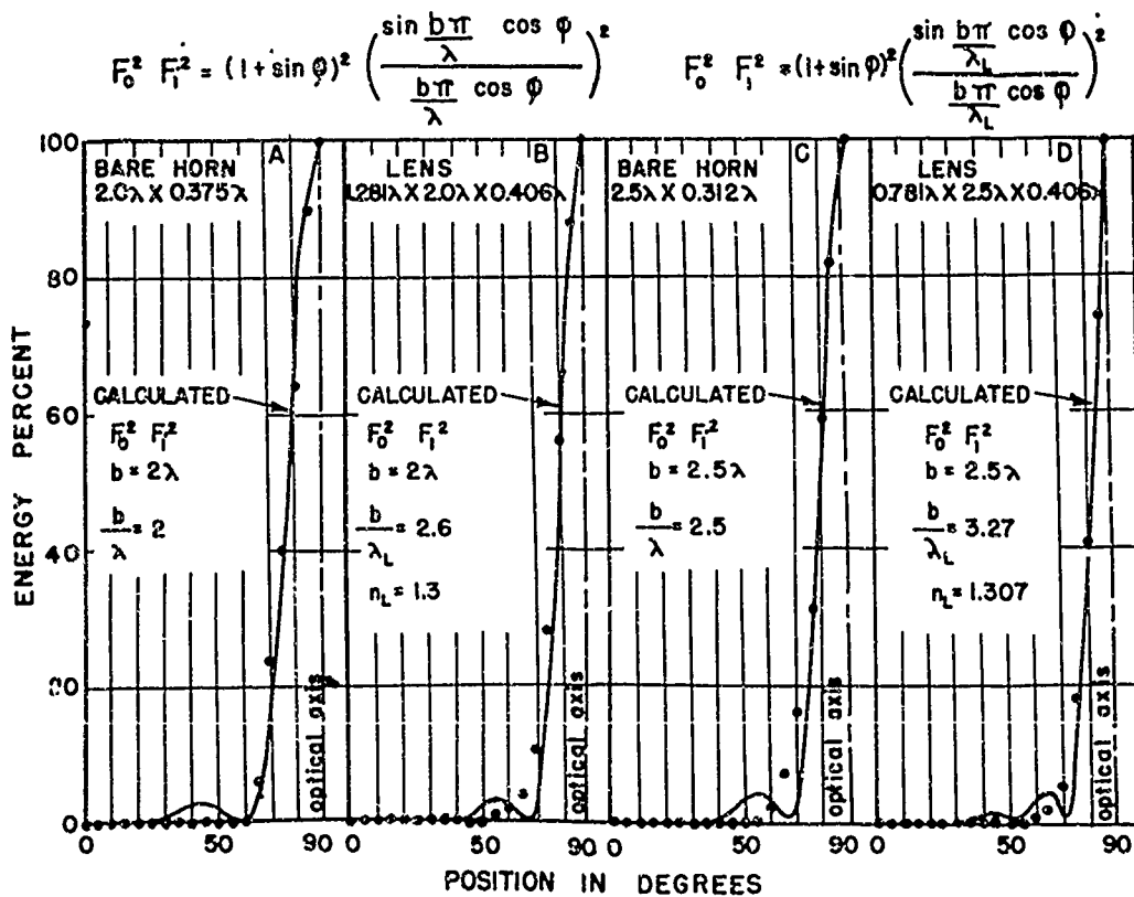
Fig. 11 WIDE RECTANGULAR LUCITE LENS H PATTERNS
