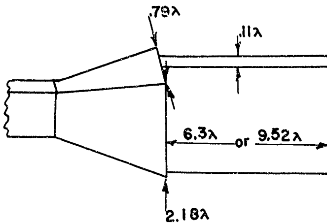
E PLANE .79\lambda \times 2.18\lambda HORN
