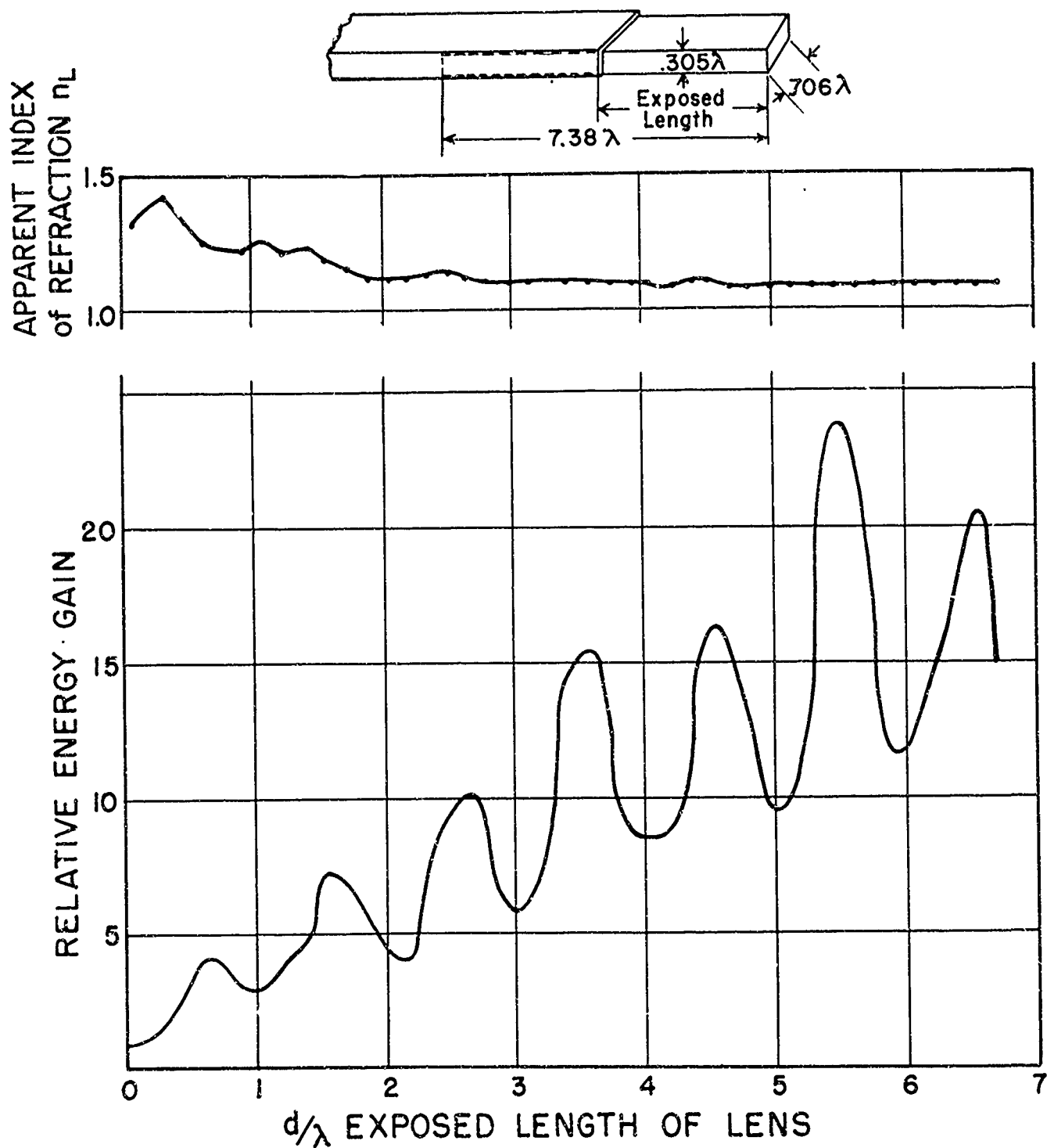
Fig. 2 LENS WITH TRANSFORMER SECTION INSIDE WAVE GUIDE
