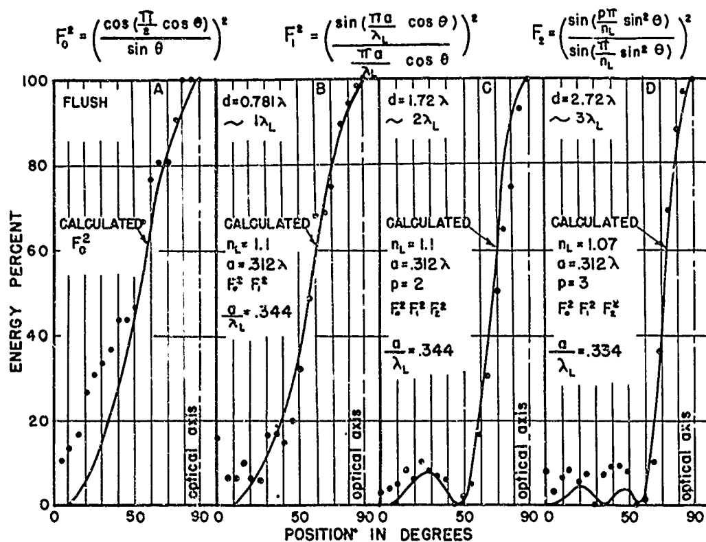
Fig. 10 NARROW RECTANGULAR FIII4 LENS E PATTERNS
