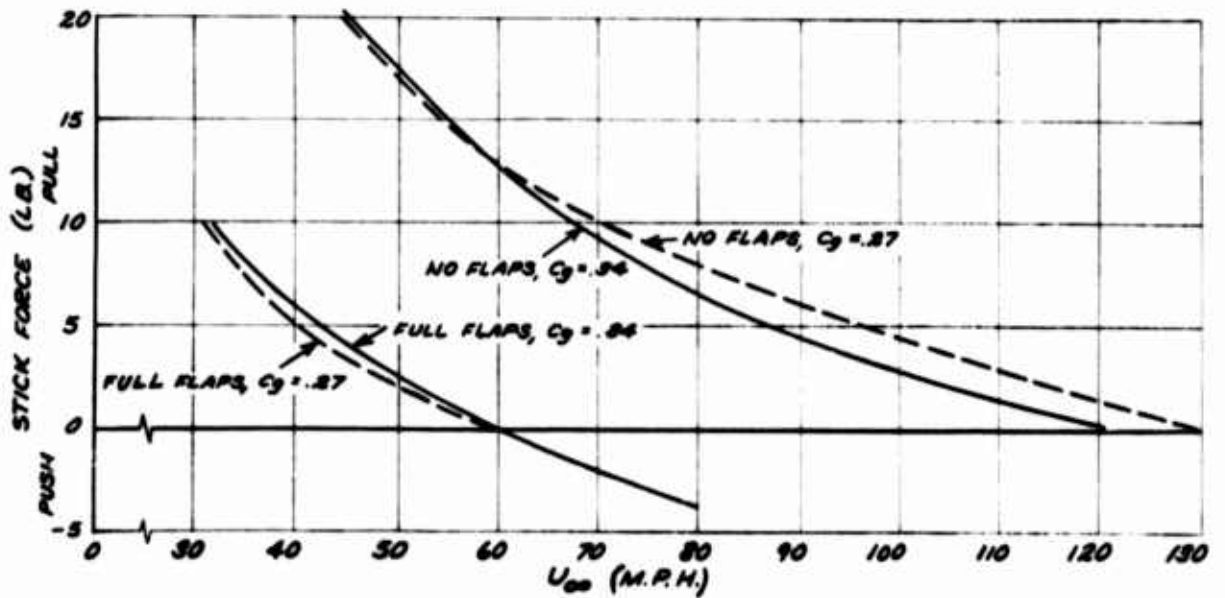
Figure 17. Stick Force Measurements on Modified L-19.
