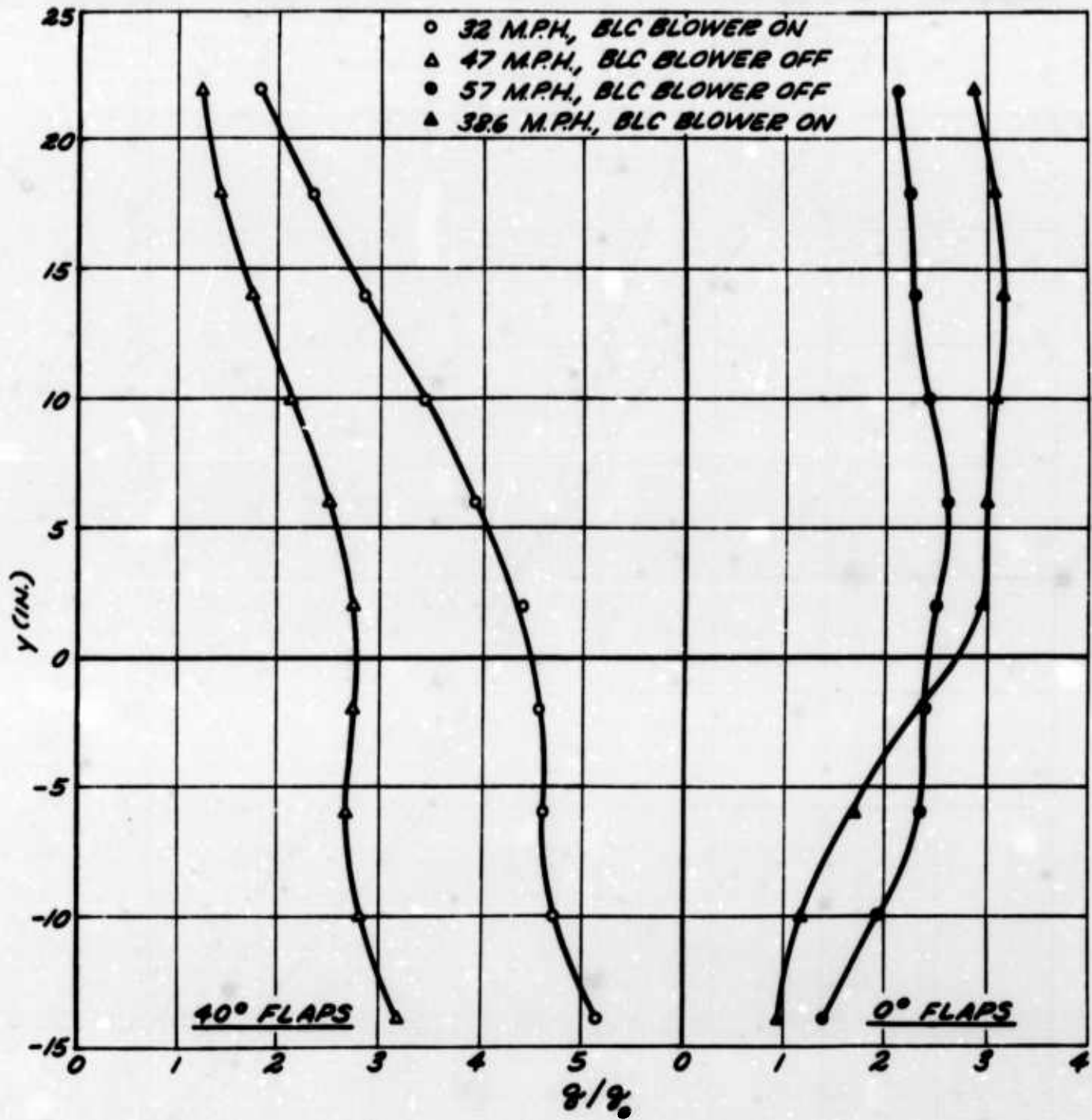
Figure 35. Results of Dynamic Head Survey at Tailplane, Level Flight Power.
