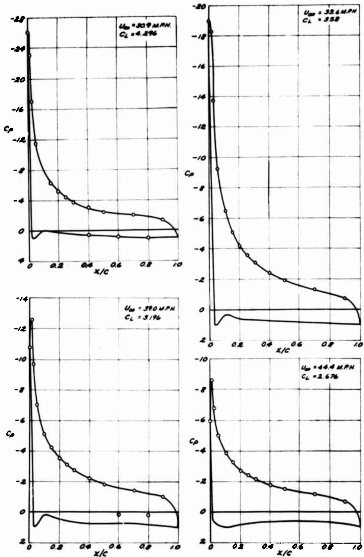
Figure 22. Wing Pressure Distributions at Various Aircraft Airspeeds, Full Flaps, BLC Blowers On.
