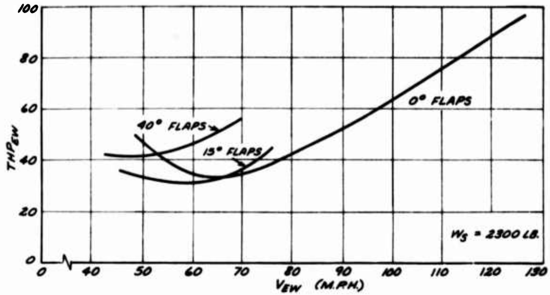
Figure 14. Power Required in Gliding Flight.
