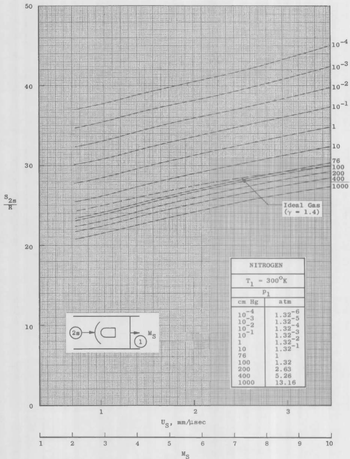
h. S_{2s}/R against Incident Shock Mach Number M_S
