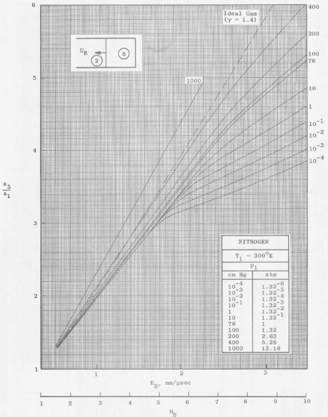
f. a_5/a_1 against Incident Shock Mach Number M_S
