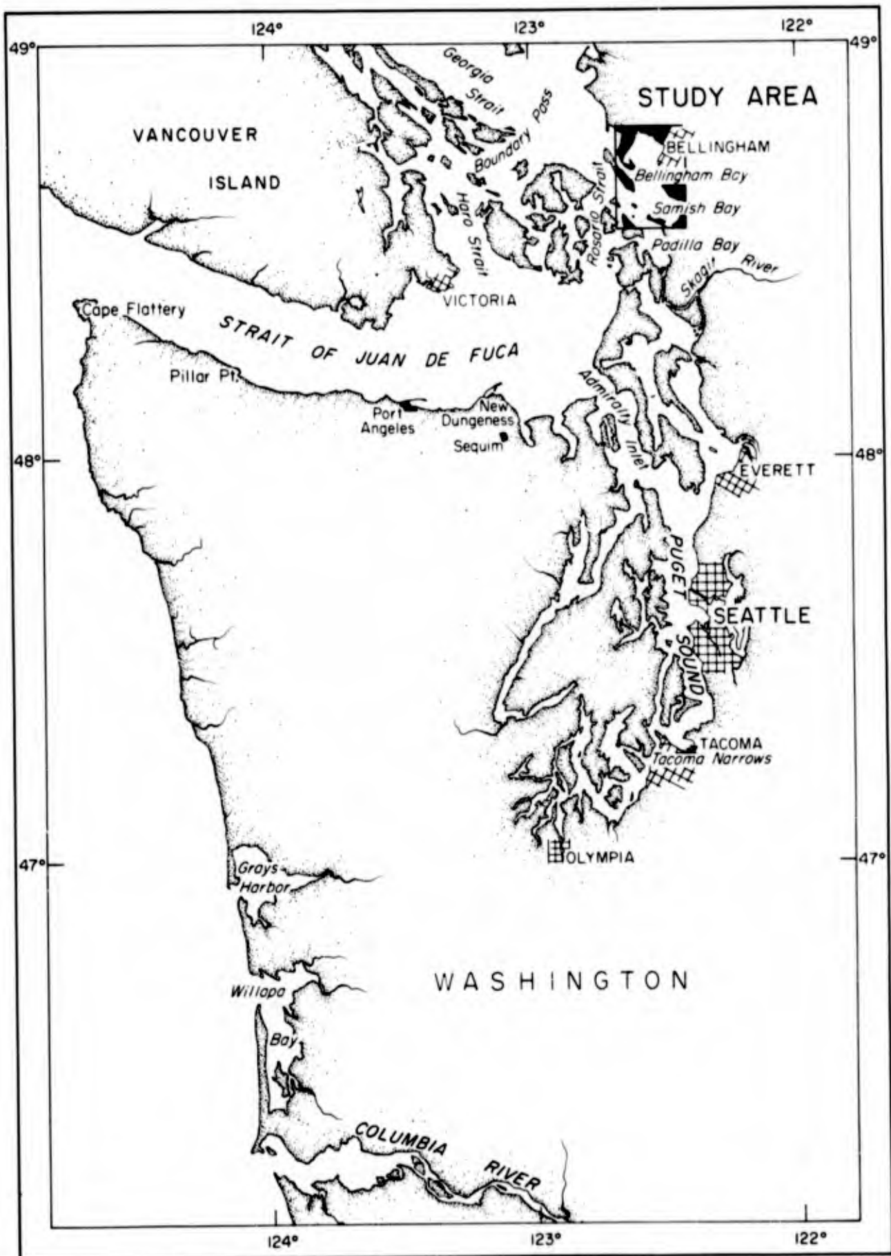
Fig. 1.1. Location of Bellingham and Samish Bays.
