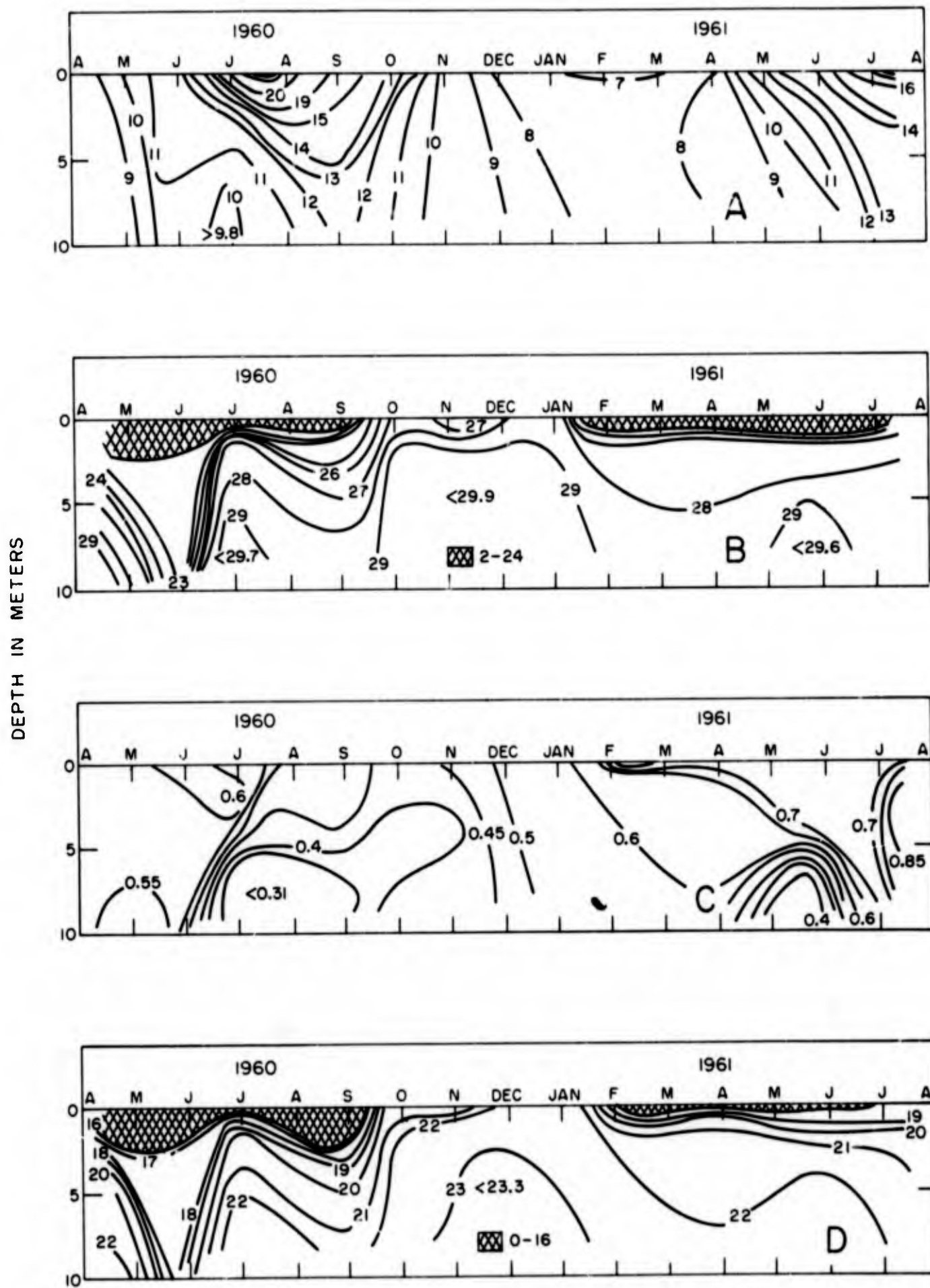
Fig. 2.2. Annual cycles at station A-3. A, temperature ( ^{\circ}\text{C} ); B, salinity (‰); C, oxygen (mg-atom/liter); D, density as \sigma_t .
