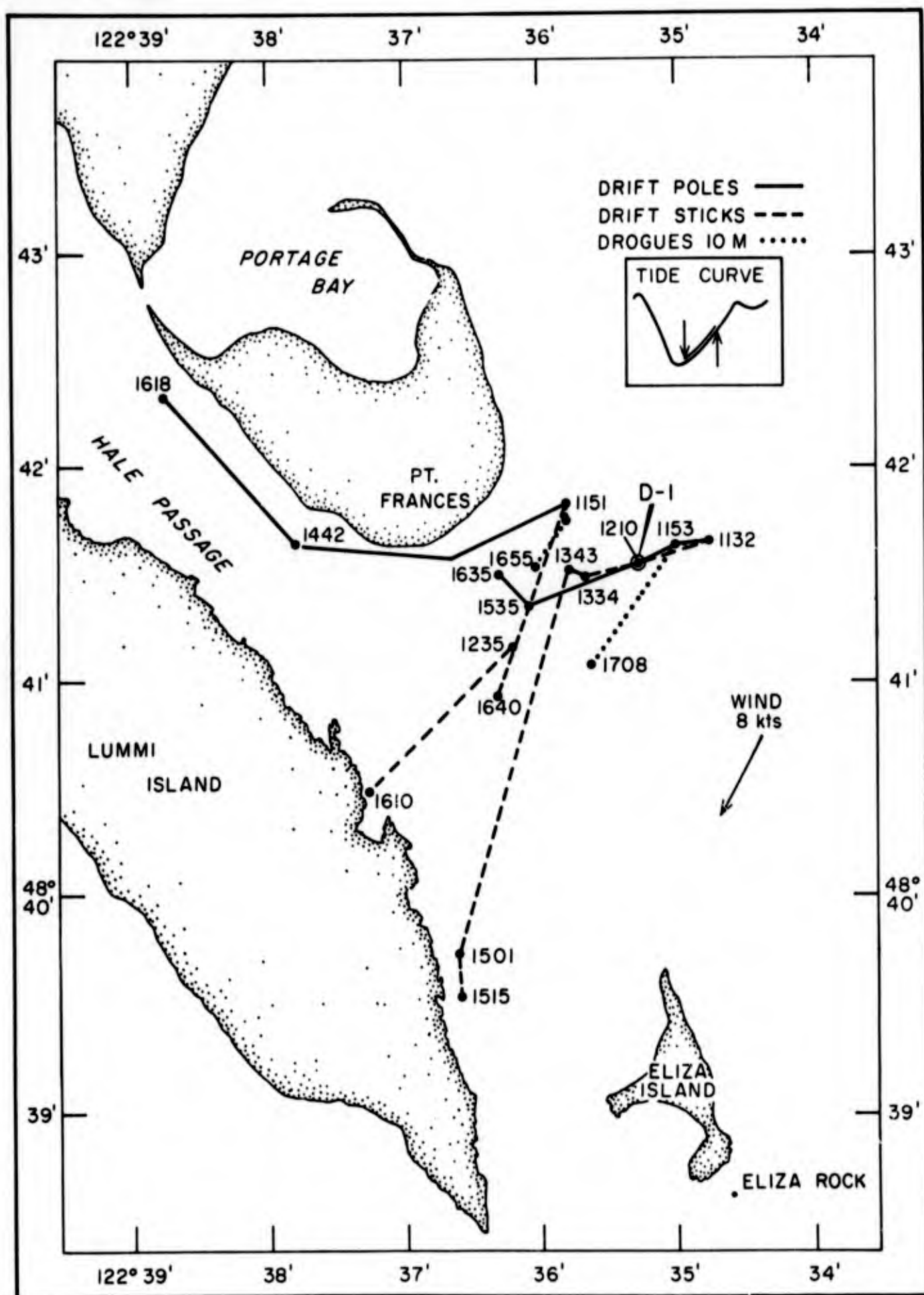
Fig. 3.3. Tracks of drift devices near stations D-1, 19 July 1960.
