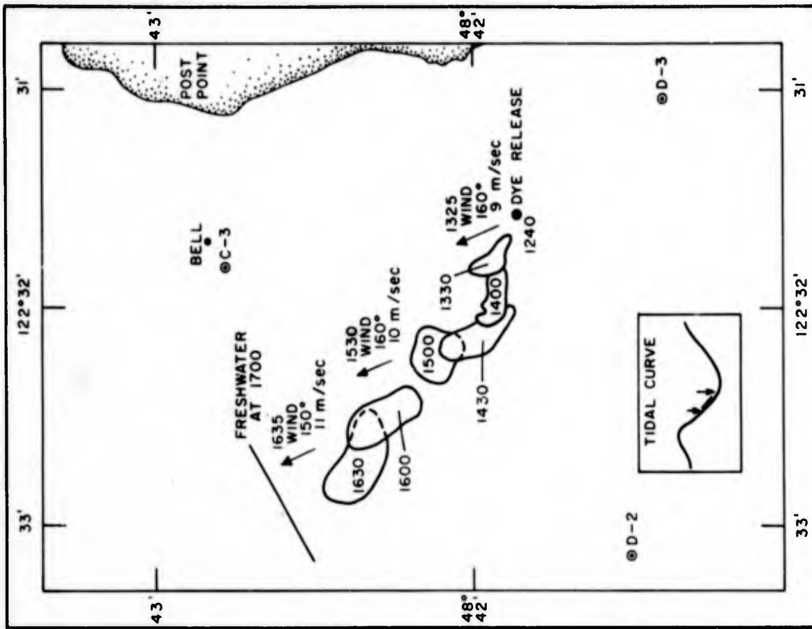
Fig. 4.2. Spread of surface dye injection, 8 February 1961.
