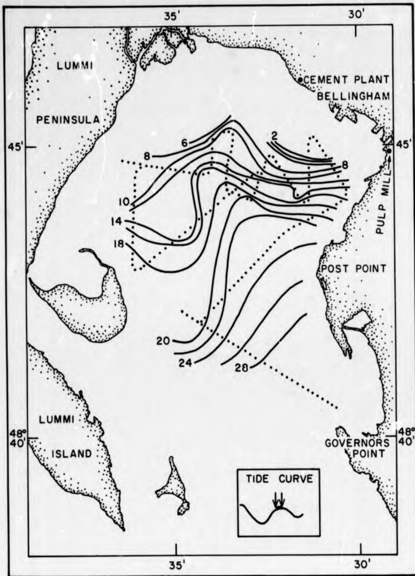
Fig. 2.25. Surface distribution of salinity in upper Bellingham Bay, 21 May 1960, 1410-1632, ebb tide.
