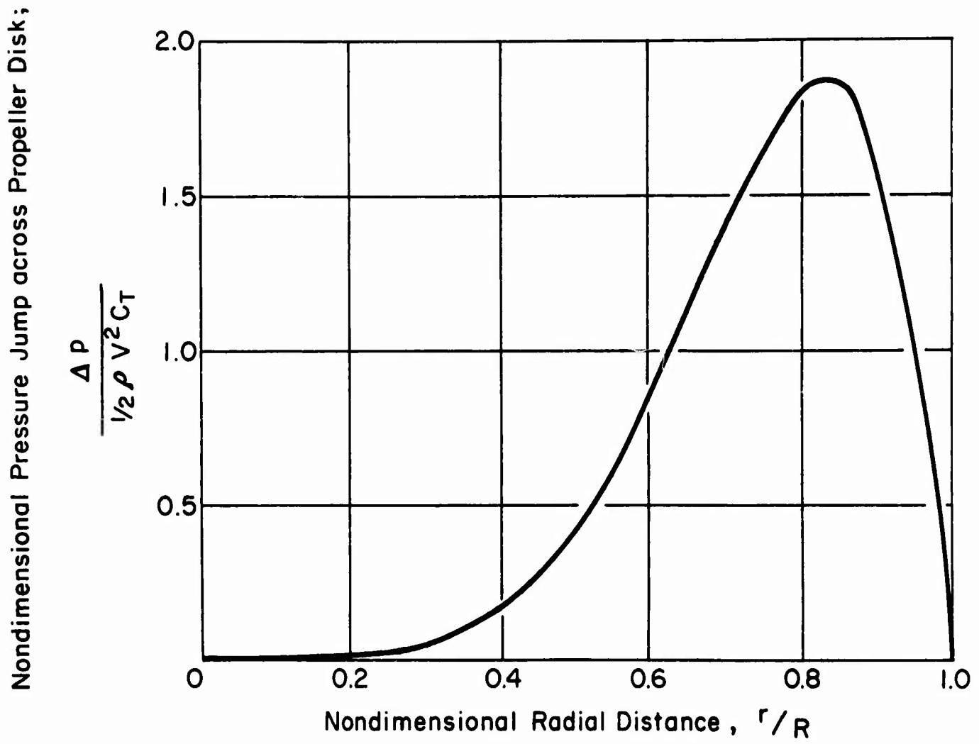
Figure 2 – Assumed Pressure Jump Variation along the Radius of the Propeller
