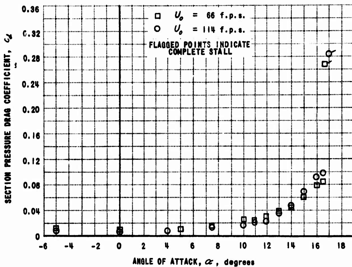
Figure 17. SECTION PRESSURE DRAG COEFFICIENT, c_d , VERSUS ANGLE OF ATTACK, \alpha , IN UNIFORM FLOW WITH LOW SOLIDITY TURBULENCE SCREEN.
