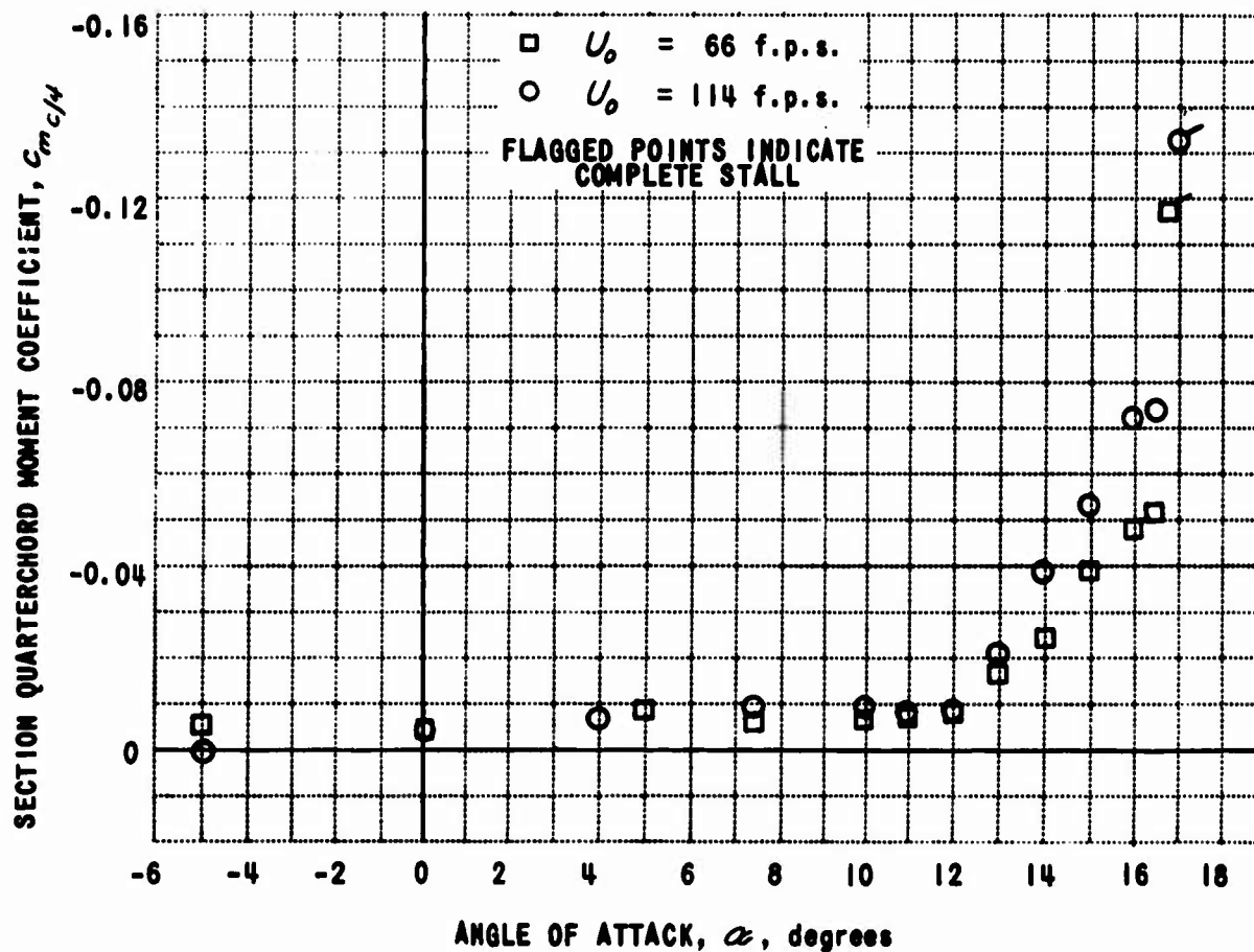
Figure 16. SECTION QUARTERCHORD MOMENT COEFFICIENT, C_{m_{c/4}} , VERSUS ANGLE OF ATTACK, \alpha , IN UNIFORM FLOW WITH LOW SOLIDITY TURBULENCE SCREEN.
