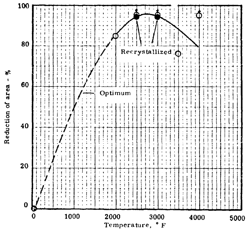
Figure 27. The elongation and reduction of area of 0.100-in. tungsten sheet in the optimum and recrystallized conditions at different temperatures.
