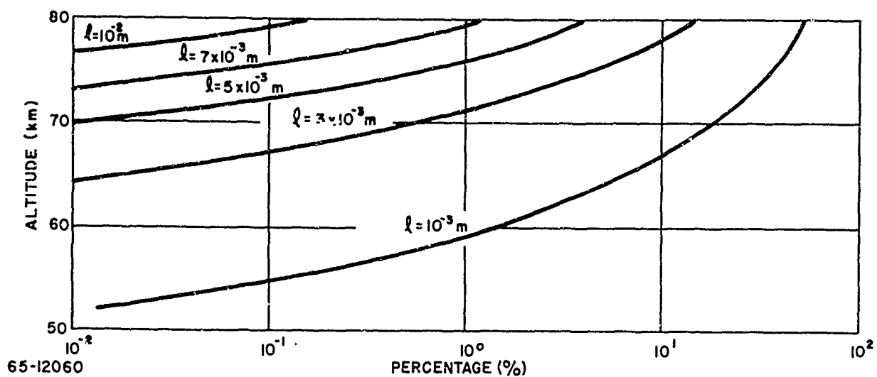
Figure 22 PERCENTAGE OF NEUTRAL PARTICLES IN THE ATMOSPHERE, WHOSE FREE PATH IS LONGER THAN l
