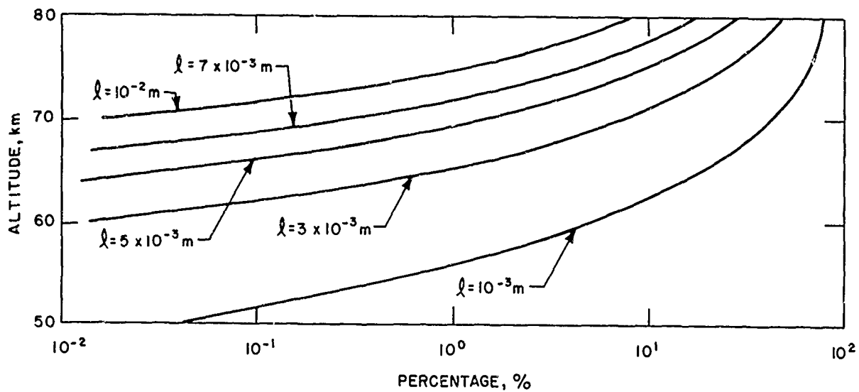
Figure 23 PERCENTAGE OF NEUTRAL PARTICLES IN THE ATMOSPHERE, WHOSE FREE PATH IS LONGER THAN l
