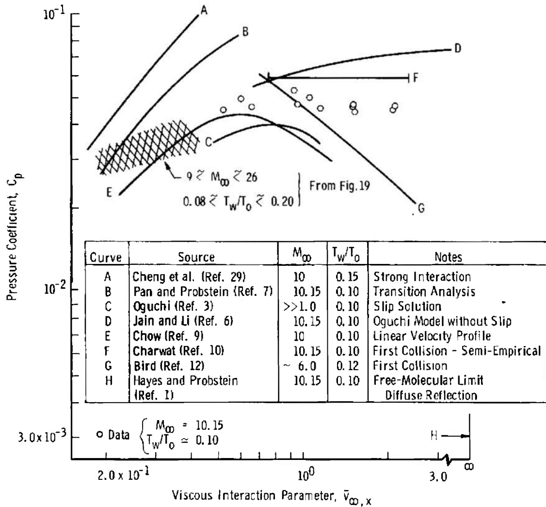
Fig. 21 Comparison of Available Theoretical Results in the Merged-Layer Regime
