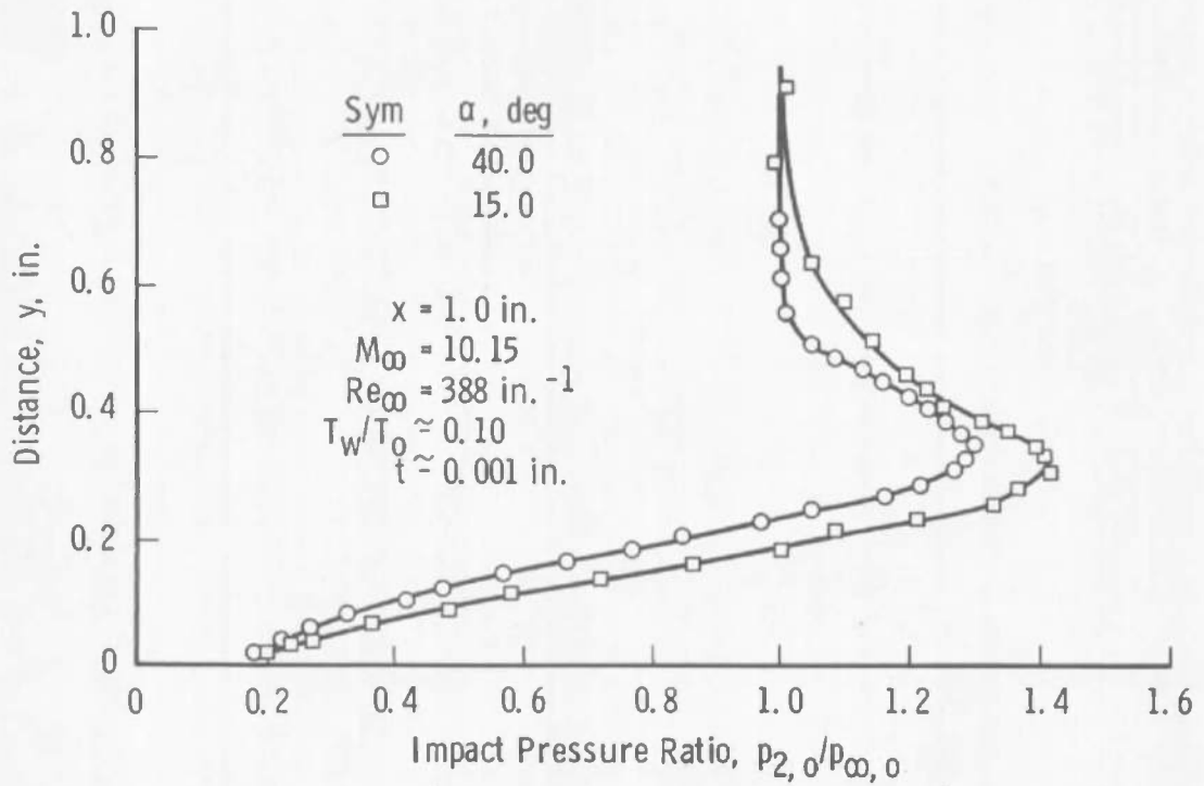
a. Flow Distortion in Shock Layer Caused by Plate Bevel Angle
