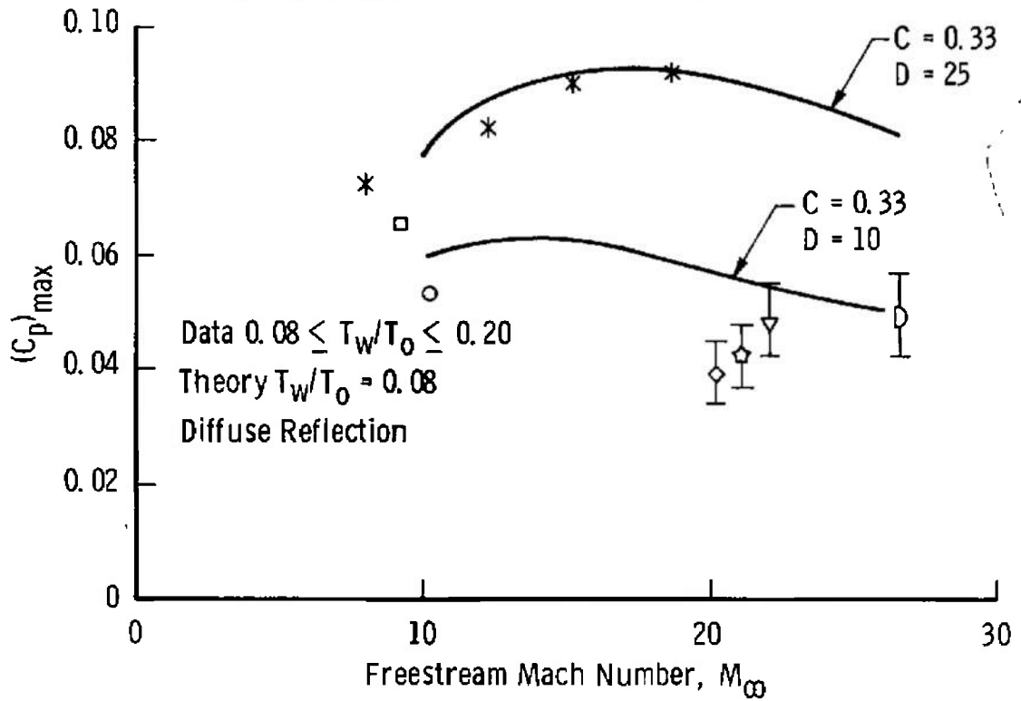
Fig. 23 First Collision Theory of Charwat (Ref. 10) Compared to Available Experimental Results
