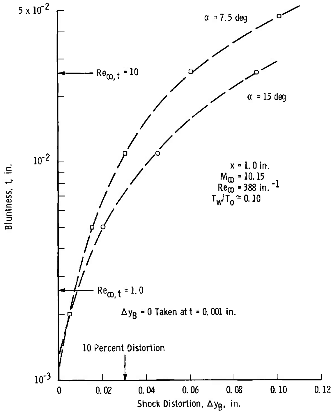
c. Effect of Leading-Edge Bluntness Fig. 7 Concluded
