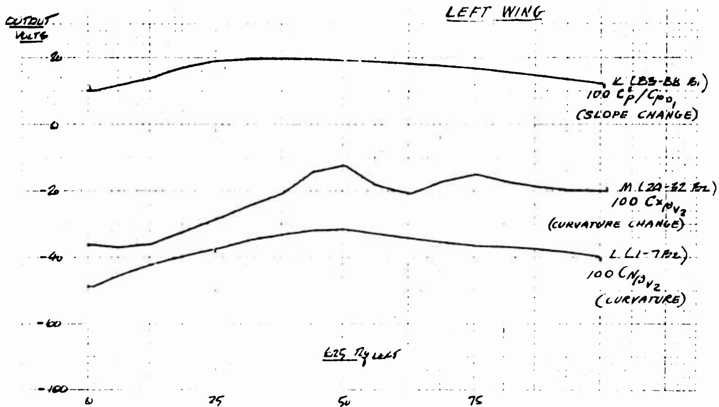
Figure 61 One Hundred Times the Linear Coefficient of the Polynomial Fit to the Fan Power Coefficient Ratio, And One Hundred Times the Second Degree Coefficient Of the Polynomial Fit to C_{X\beta v} and C_{N\beta v} Plotted vs 625 R_q for the Left Wing
