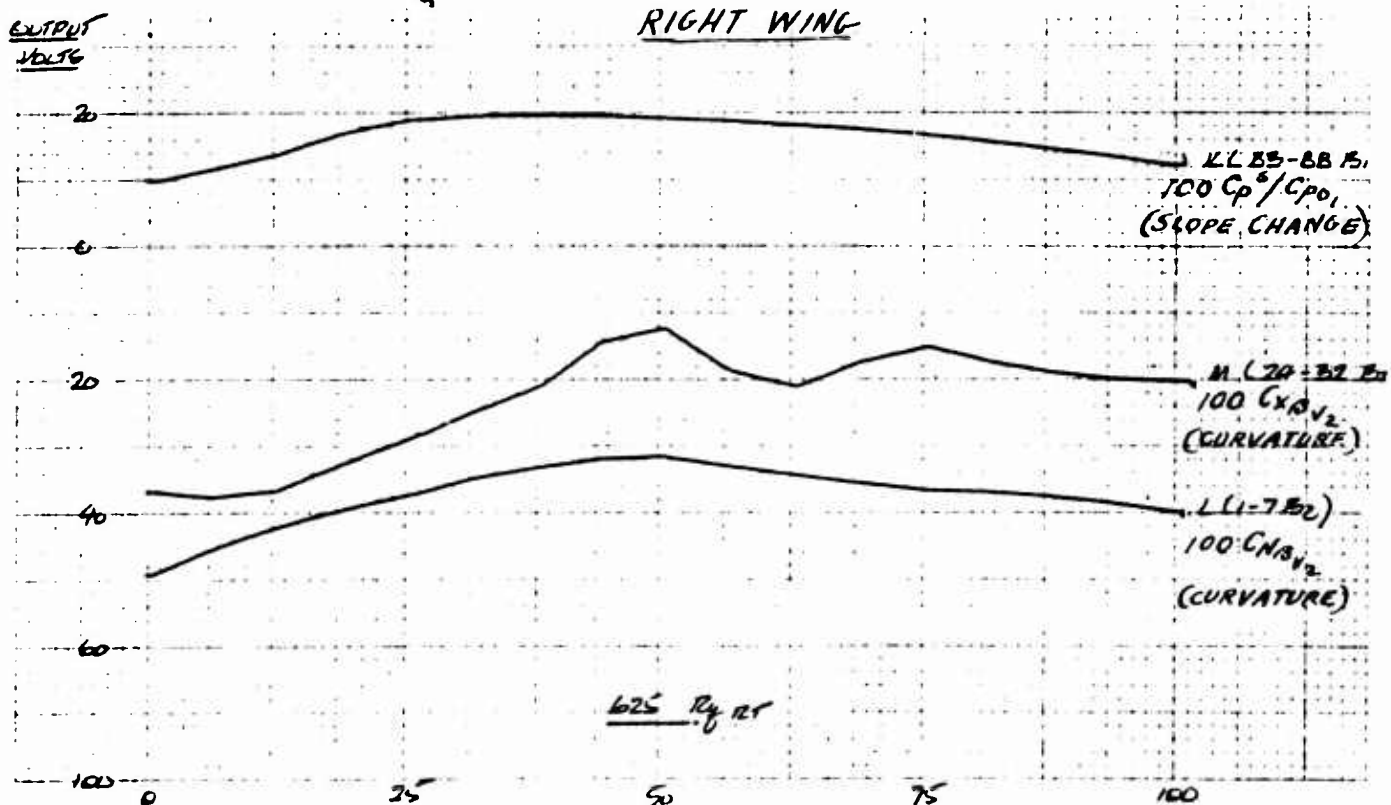
Figure 62 One Hundred Times the Linear Coefficient of the Polynomial Fit to the Fan Power Coefficient Ratio, And One Hundred Times the Second Degree Coefficient Of the Polynomial Fit to C_{X\beta v} and C_{N\beta v} Plotted vs 625 R_q for the Right Wing
