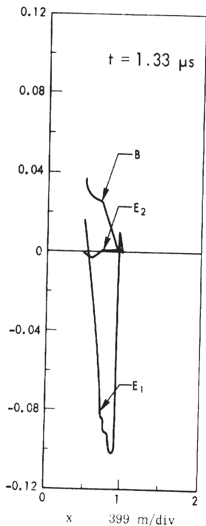
Fig. 3a--The dipole fields as functions of radius for several times for the \Delta = 1/8 case. As before Y = 1 ton and z = 2 km.
