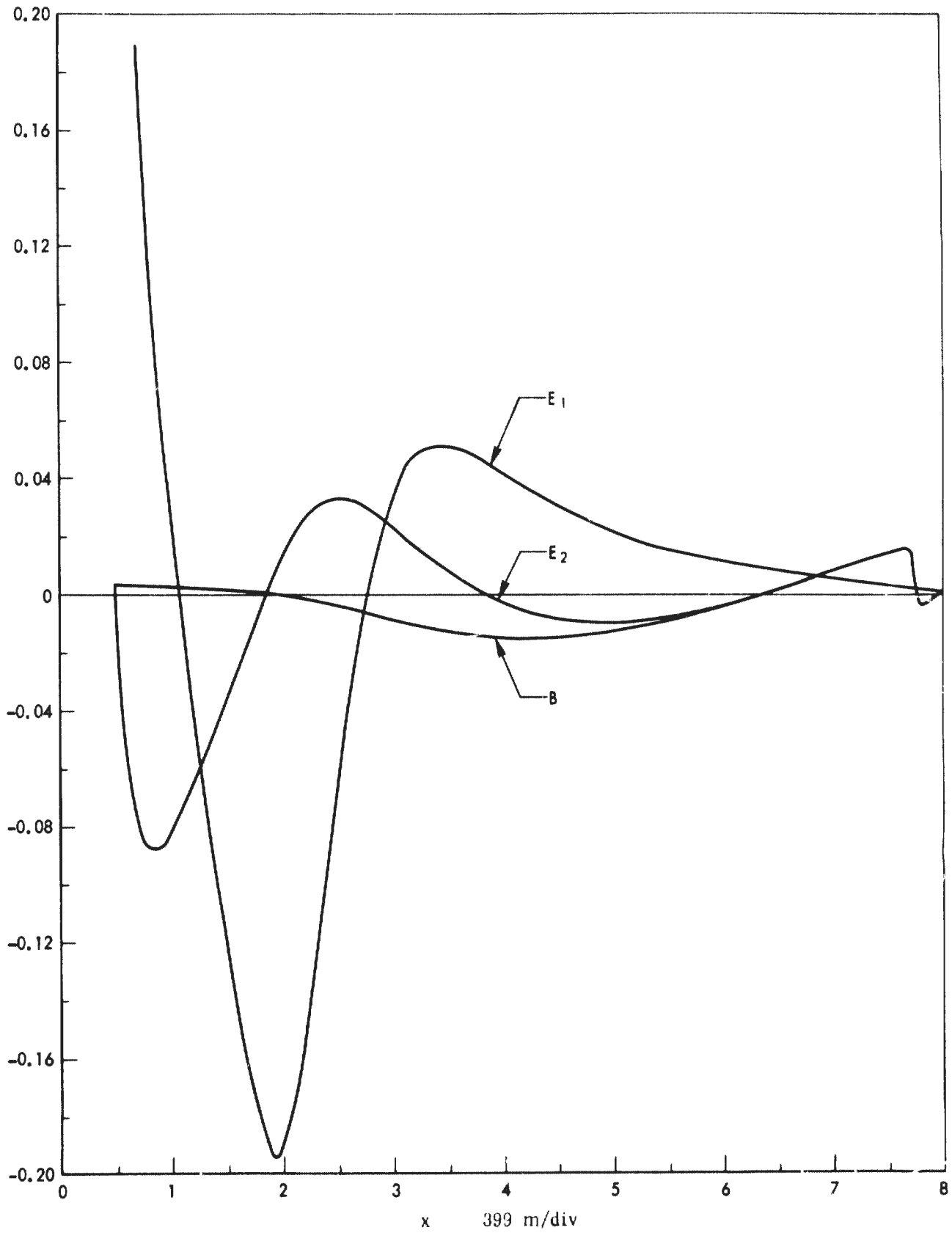
Fig. 3f--The dipole fields at t = 10.64 \mu\text{s} .
