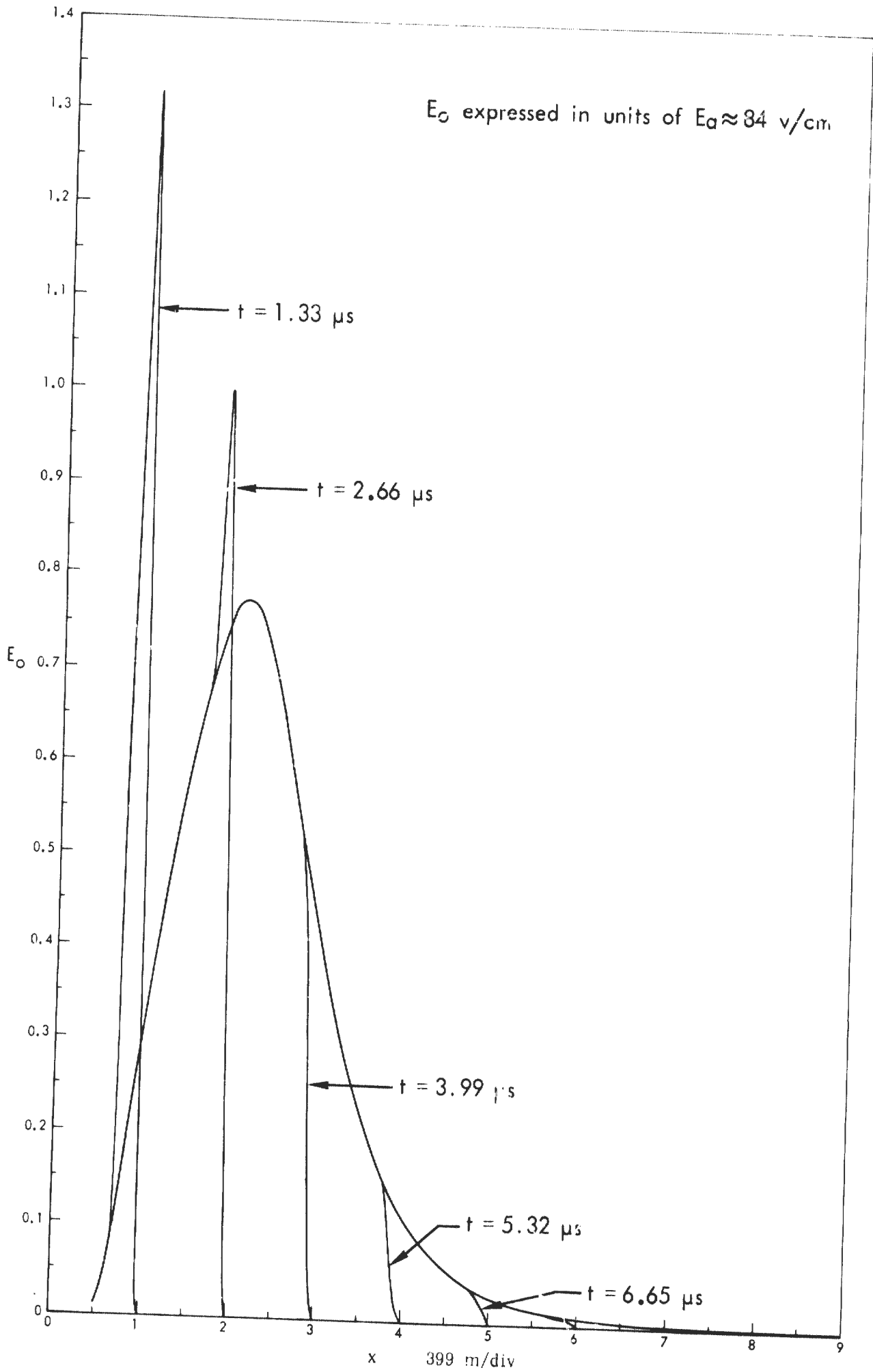
Fig. 2-- E_0 , the spherically symmetric part of the radial field as a function of position for various times for the case \Delta = 1/8 . The field approaches an asymptotic form because ionic conductivity is neglected.
