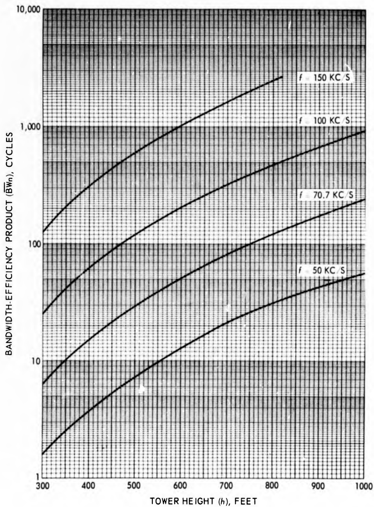
Figure 7. Variation of reference tower bandwidth - efficiency product with tower height ( h/d = 200 ).
