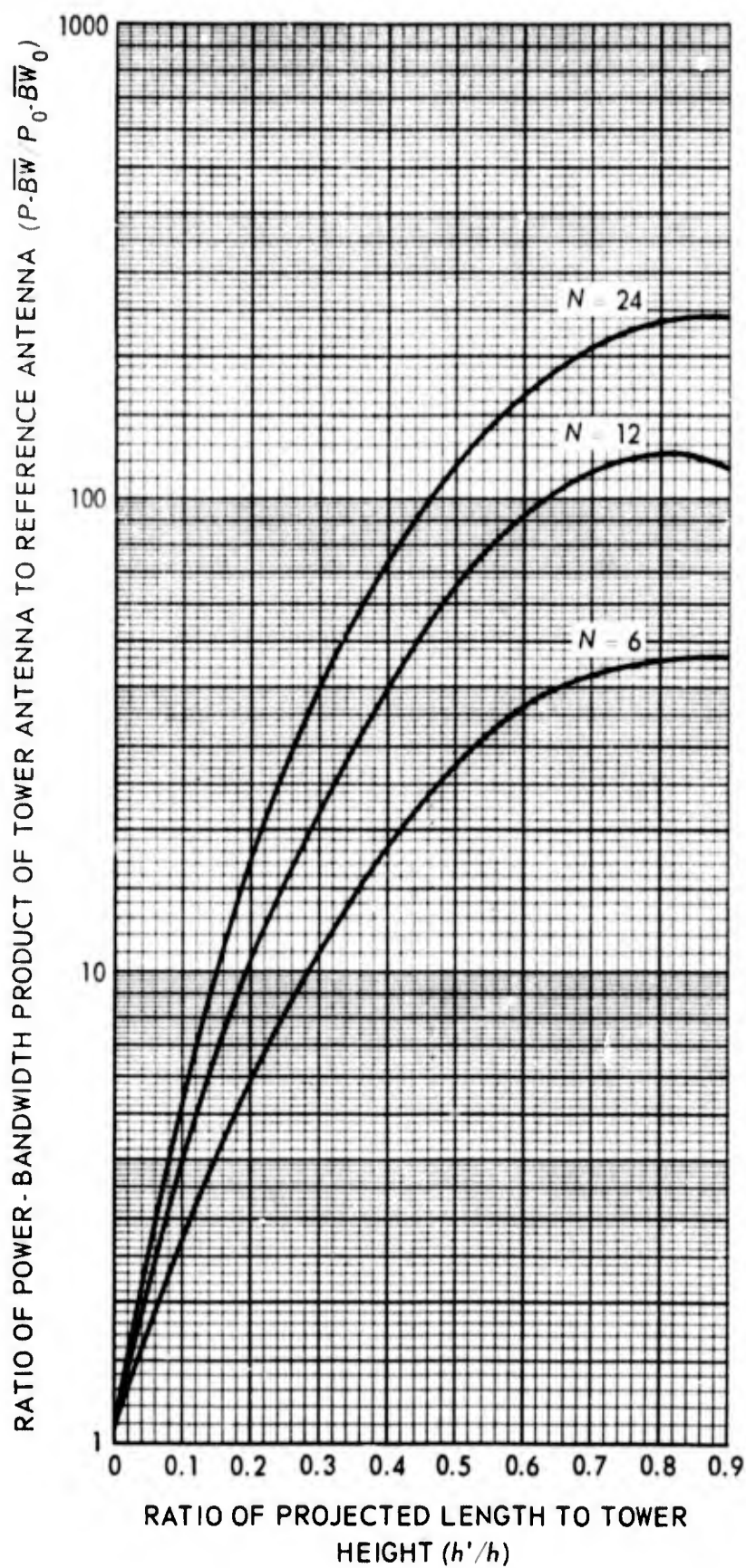
Figure 33. Normalized power-bandwidth product of three top-loaded antennas, \rho = h .
