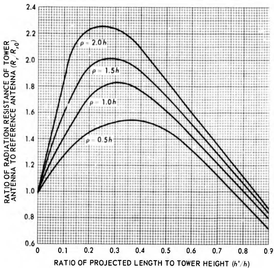
Figure 20. Normalized radiation resistance of top-loaded antenna, N=12 .
