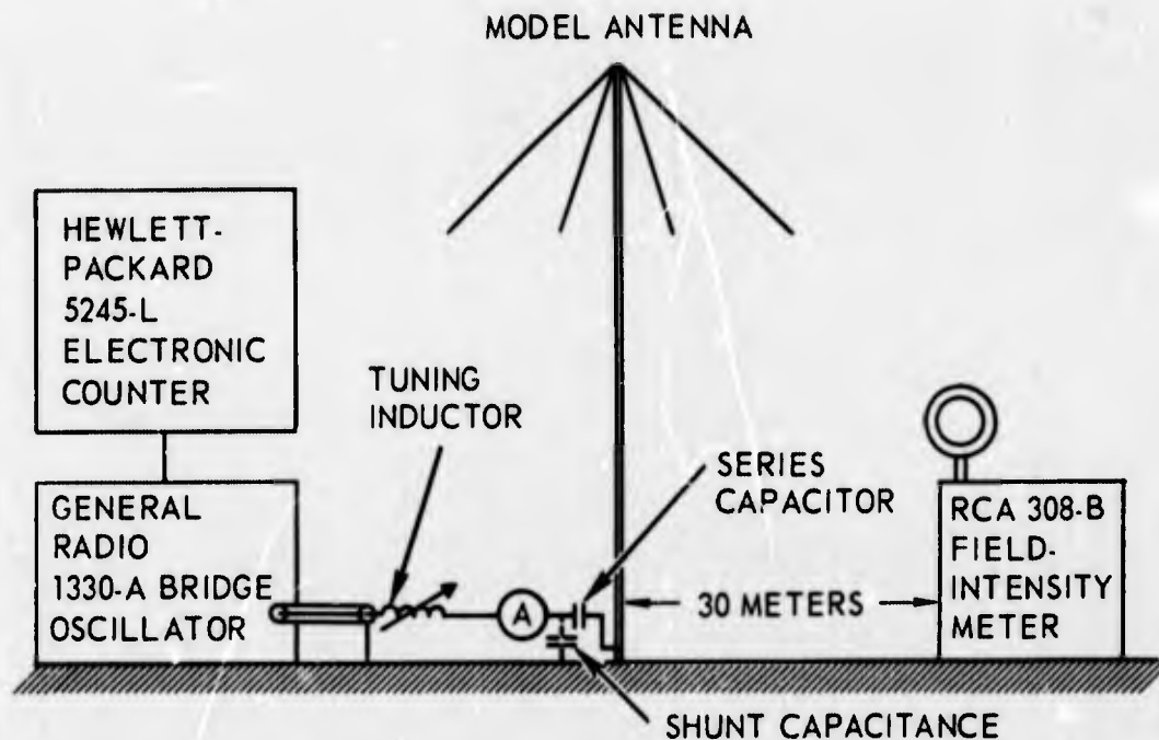
Figure 2. Test equipment for determining antenna characteristics.
