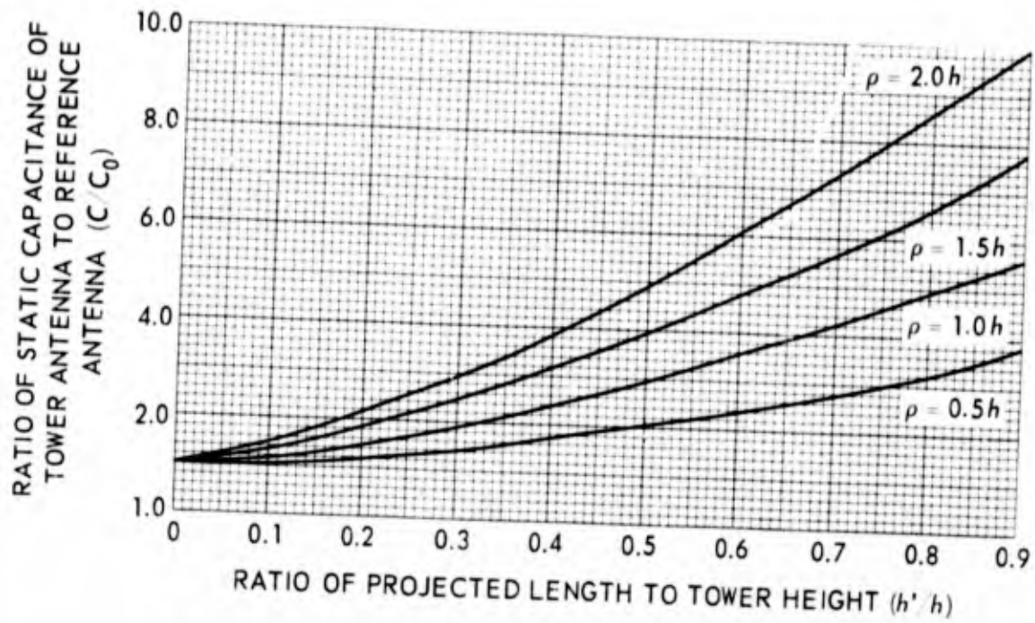
Figure 17. Normalized static capacitance of top-loaded antenna, N = 12
