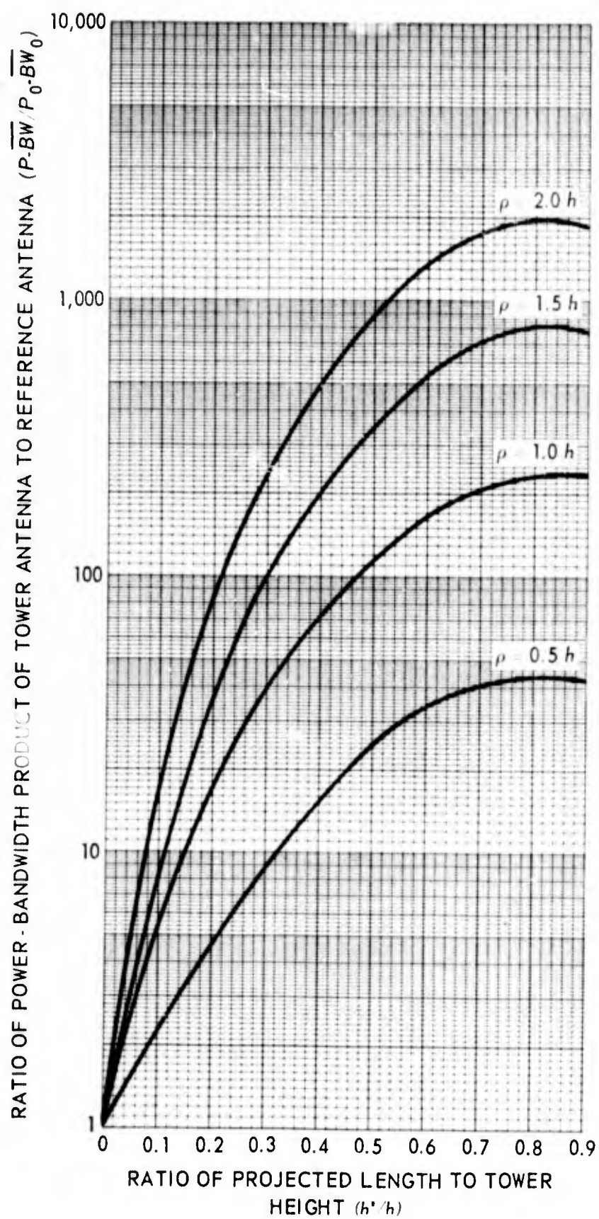
Figure 30. Normalized power-bandwidth product of top-loaded antenna, N = 24 .
