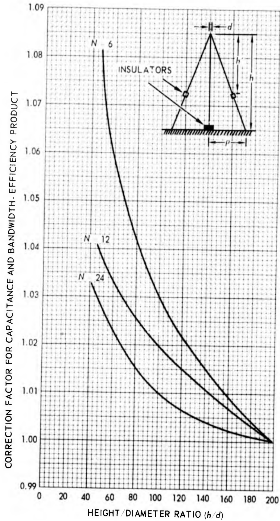
Figure 34. Correction factor for capacitance and bandwidth-efficiency product, \rho = h .
