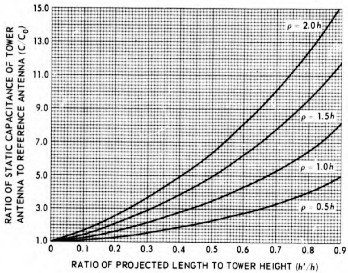
Figure 24. Normalized static capacitance of top-loaded antenna, N=24 .
