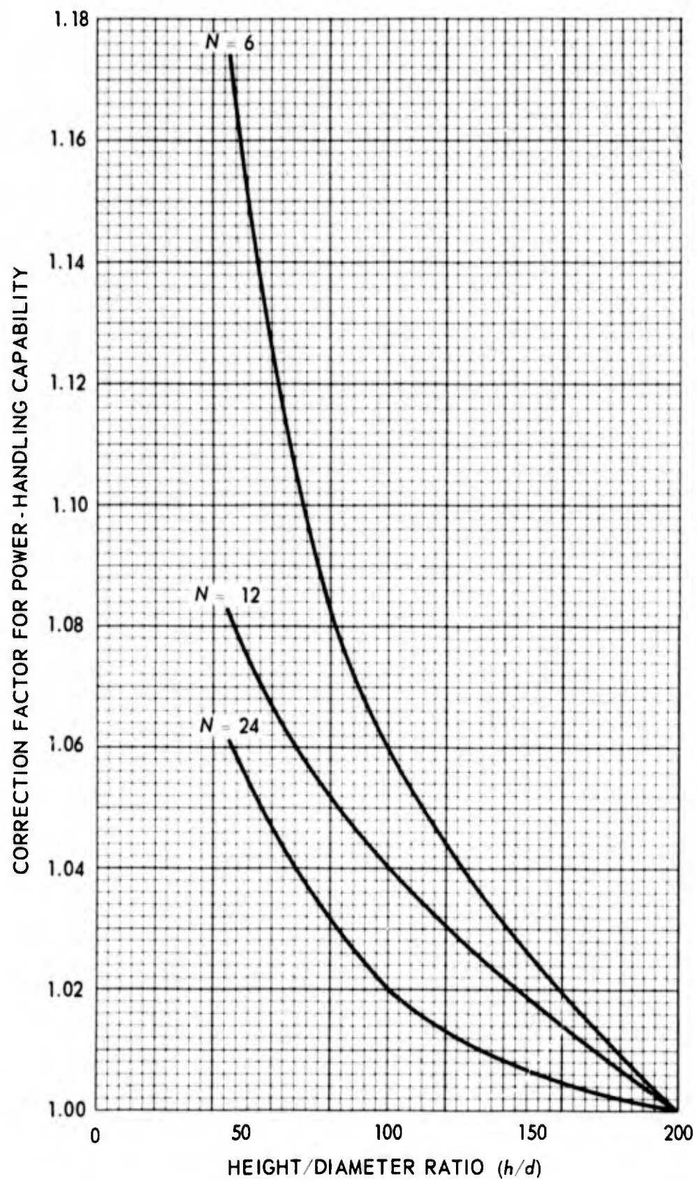
Figure 35. Correction factor for power-handling capability, \rho = h .
