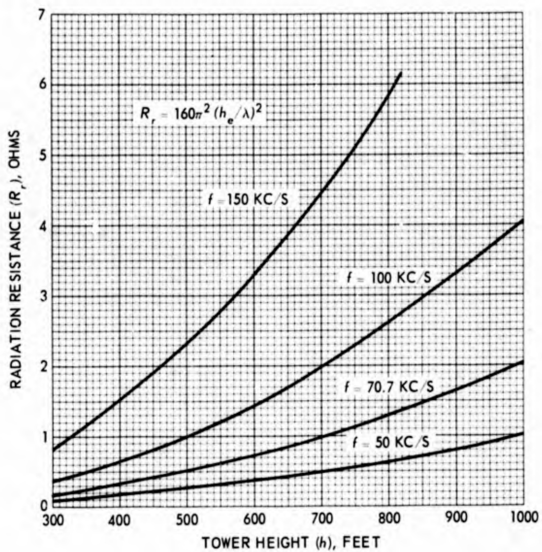
Figure 6. Variation of radiation resistance of reference antenna with tower height ( h/d=200 ).
