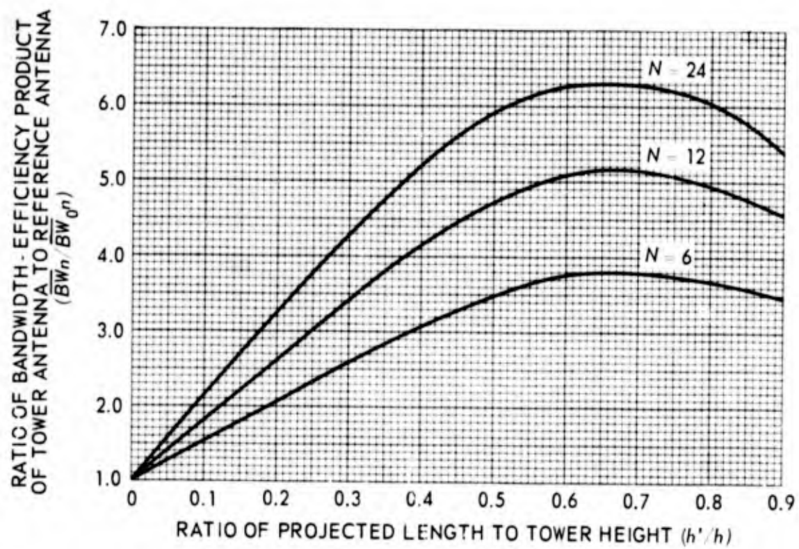
Figure 32. Normalized bandwidth-efficiency product of three top-loaded antennas, \rho=h .
