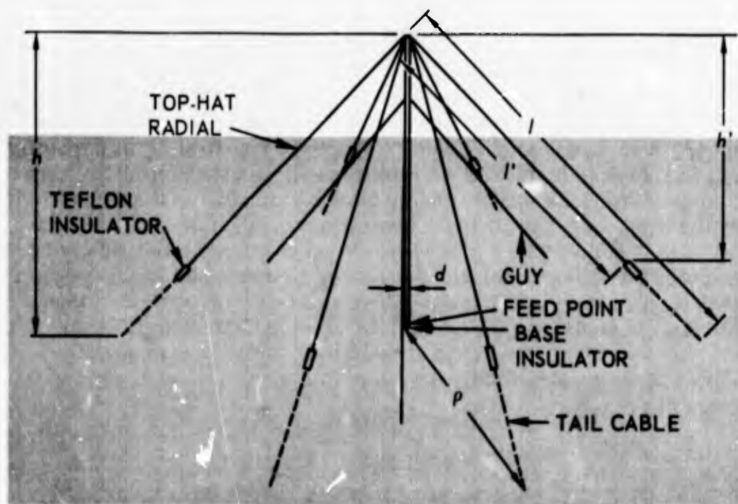
Figure 1. Top-loaded antenna, overall view.
