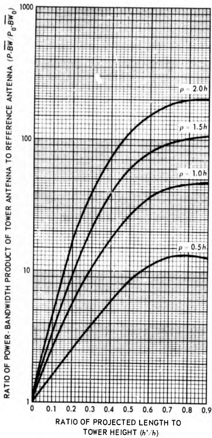
Figure 16. Normalized power-bandwidth product of top-loaded antenna, N=6 .
