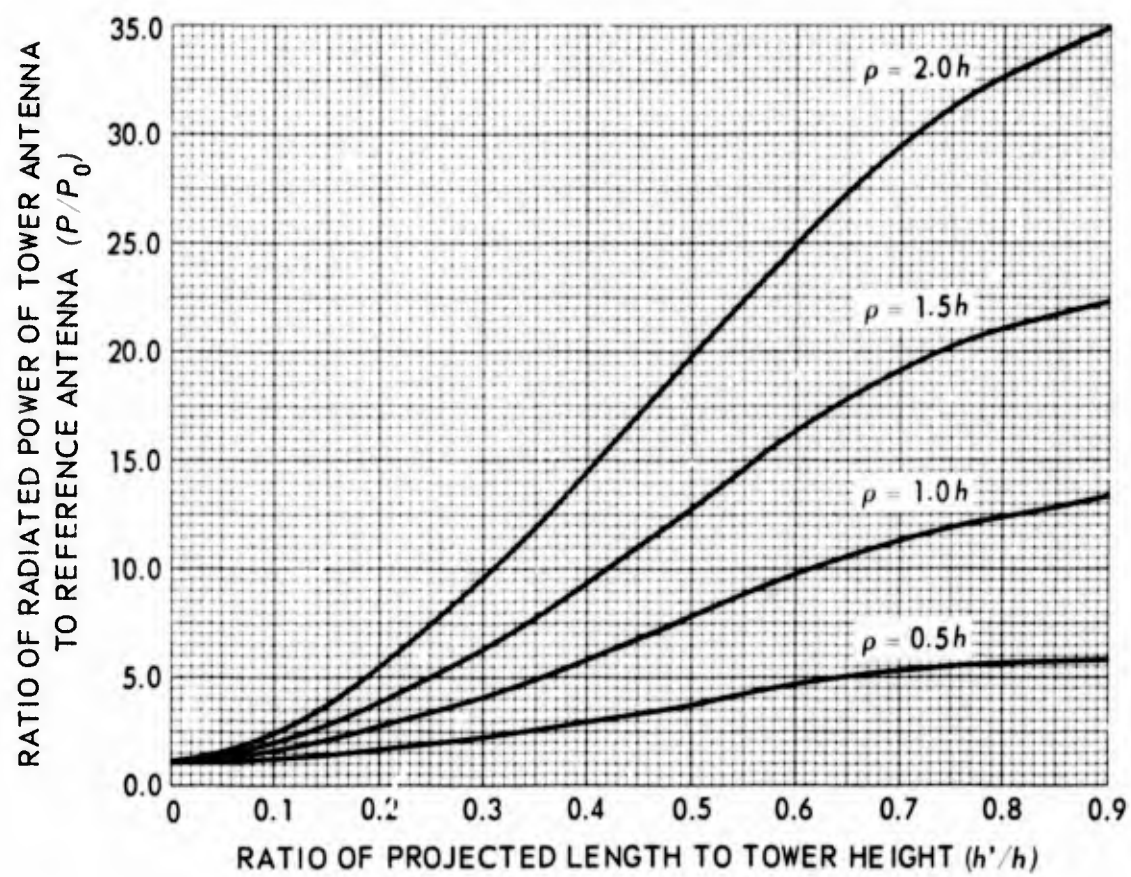
Figure 15. Normalized radiated power of top-loaded antenna, N=6 .
