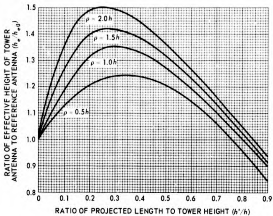
Figure 19. Normalized effective height of top-loaded antenna, N=12 .
