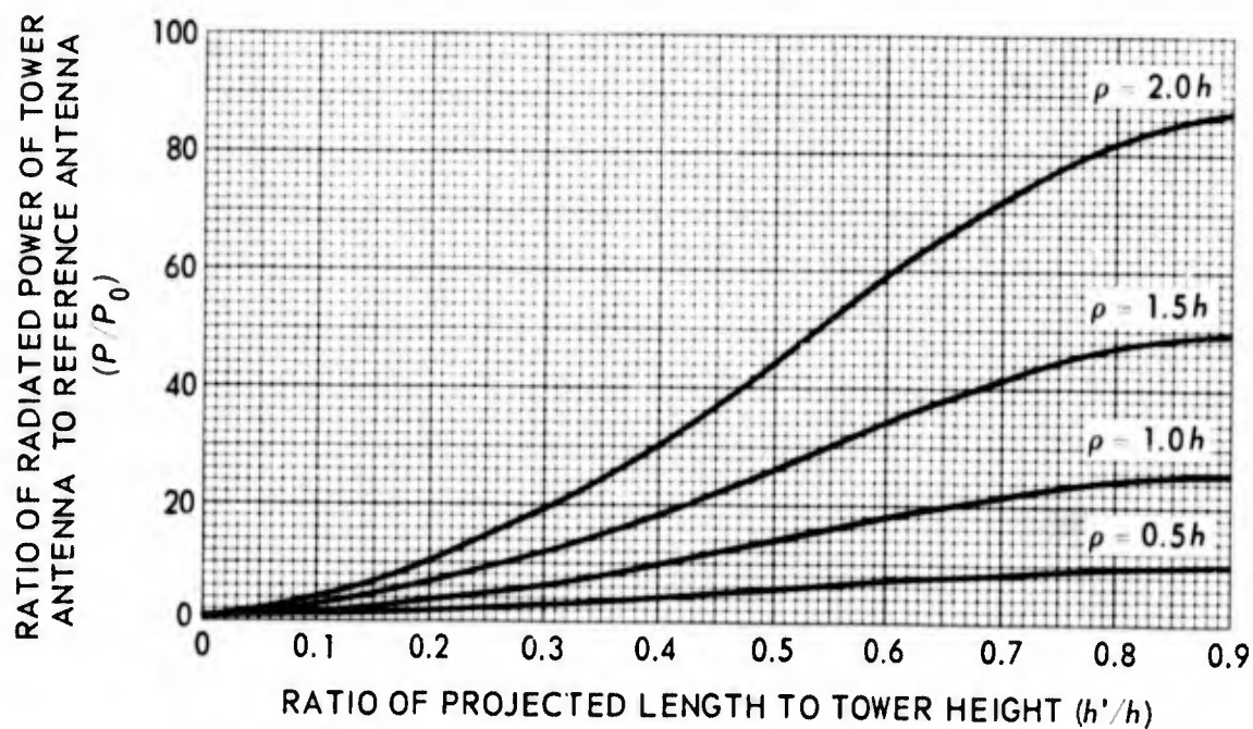
Figure 22. Normalized radiated power of top-loaded antenna, N=12 .
