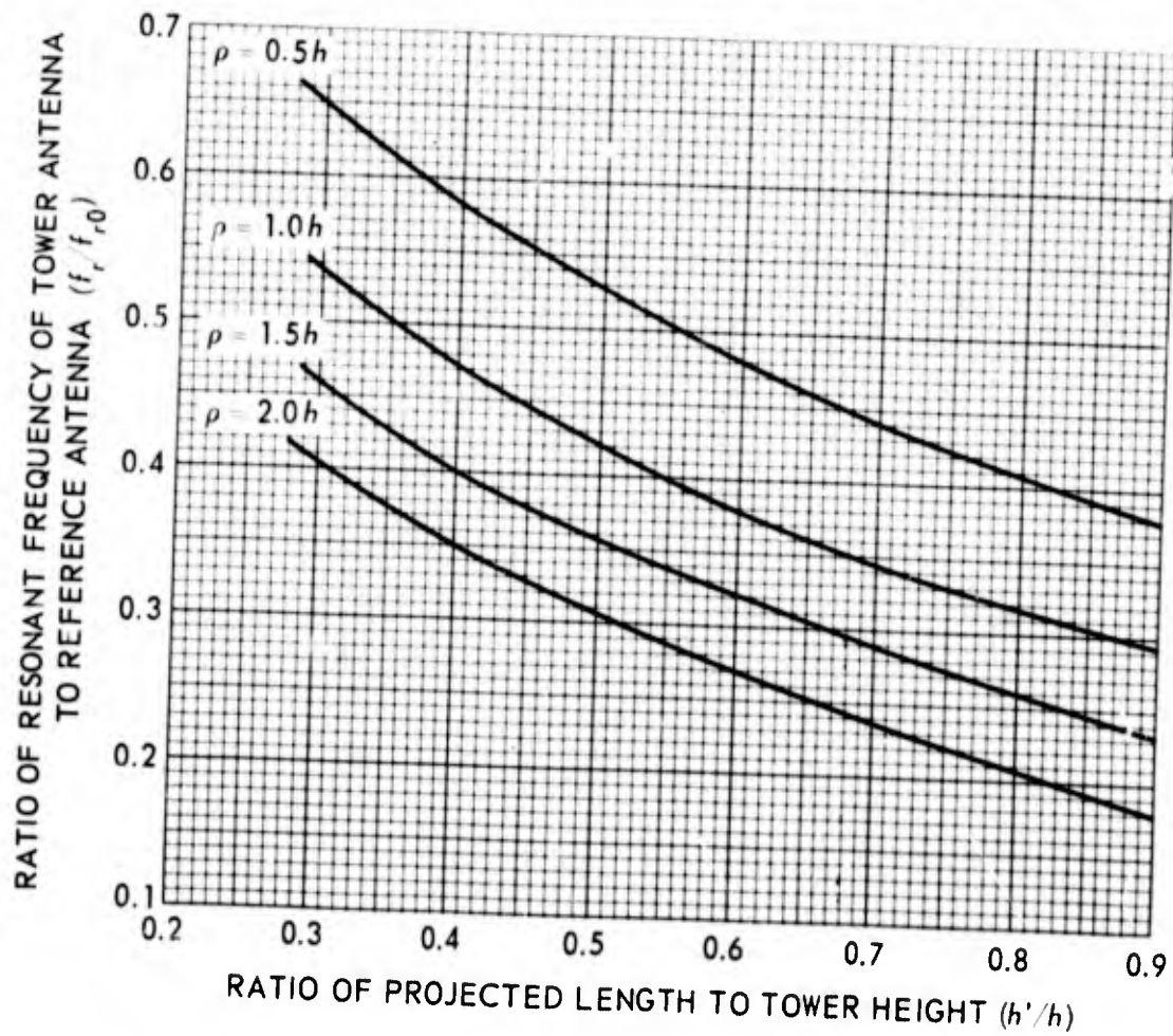
Figure 18. Normalized resonant frequency of top-loaded antenna, N = 12 .
