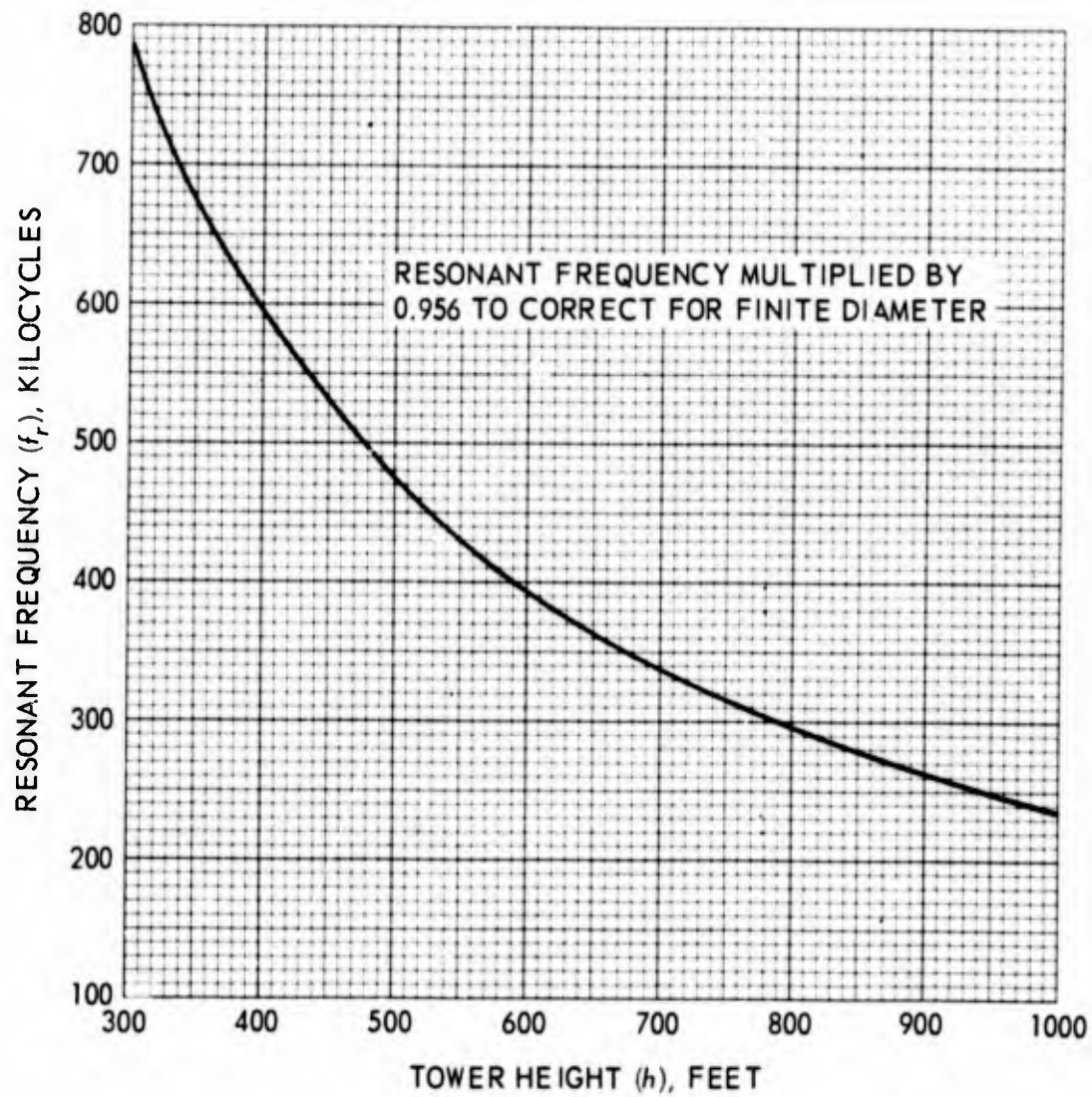
Figure 4. Computed resonant frequency of reference antenna as a function of tower height ( h/d = 200 ).
