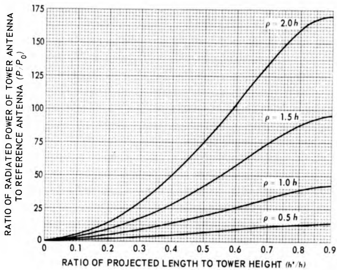
Figure 29. Normalized radiated power of top-loaded antenna, N = 24 .
