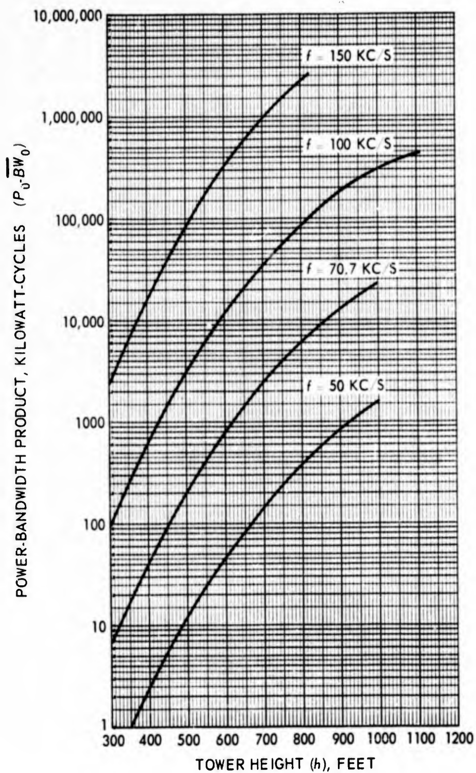
Figure 9. Variation of reference antenna power-bandwidth product with tower height ( h/d = 200 ).
