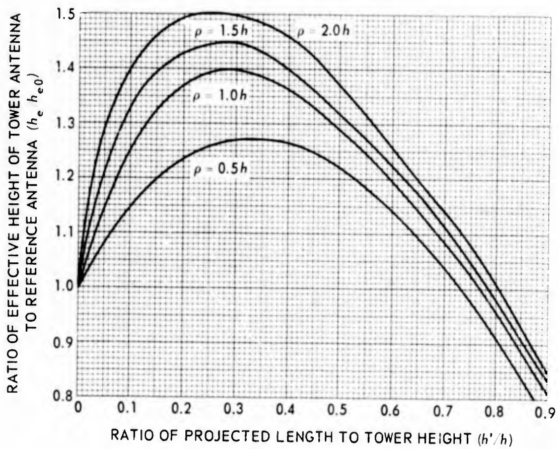
Figure 26. Normalized effective height of top-loaded antenna, N=24 .
