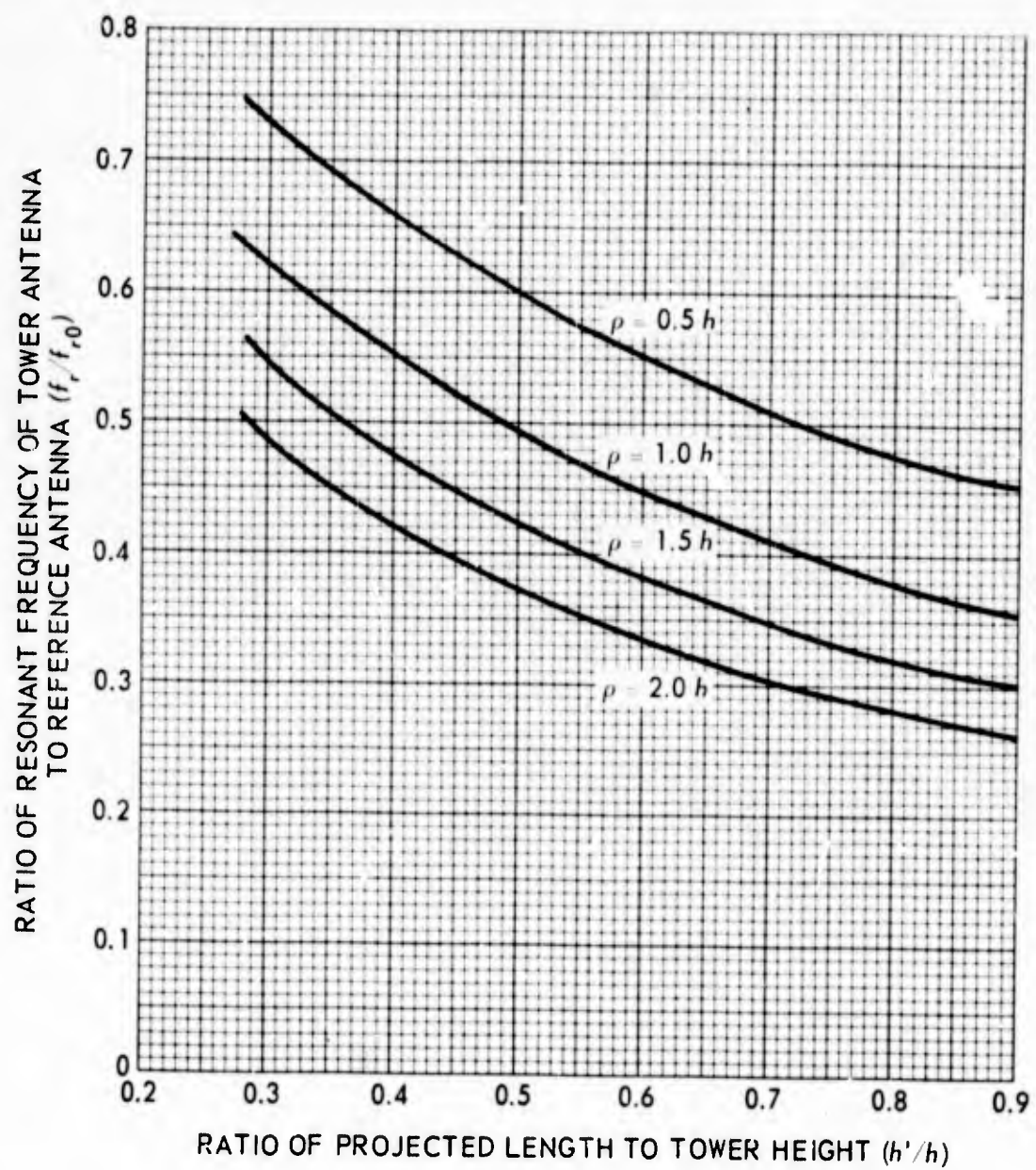
Figure 11. Normalized resonant frequency of top-loaded antenna, N=6 .
