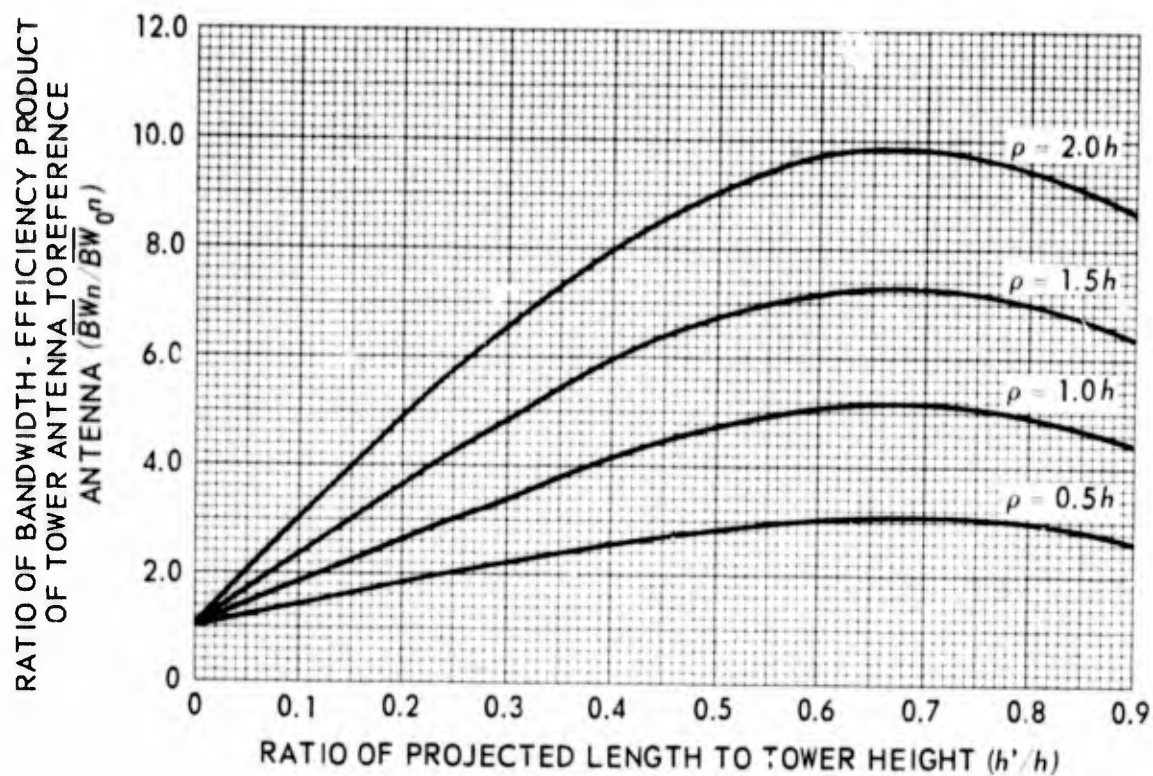
Figure 21. Normalized bandwidth-efficiency product of top-loaded antenna, N=12 .
