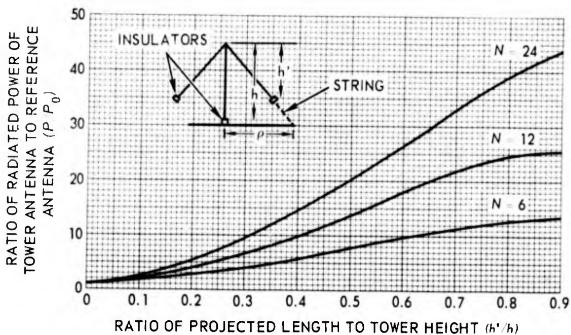
Figure 31. Normalized radiated power of three top-loaded antennas, \rho = h .
