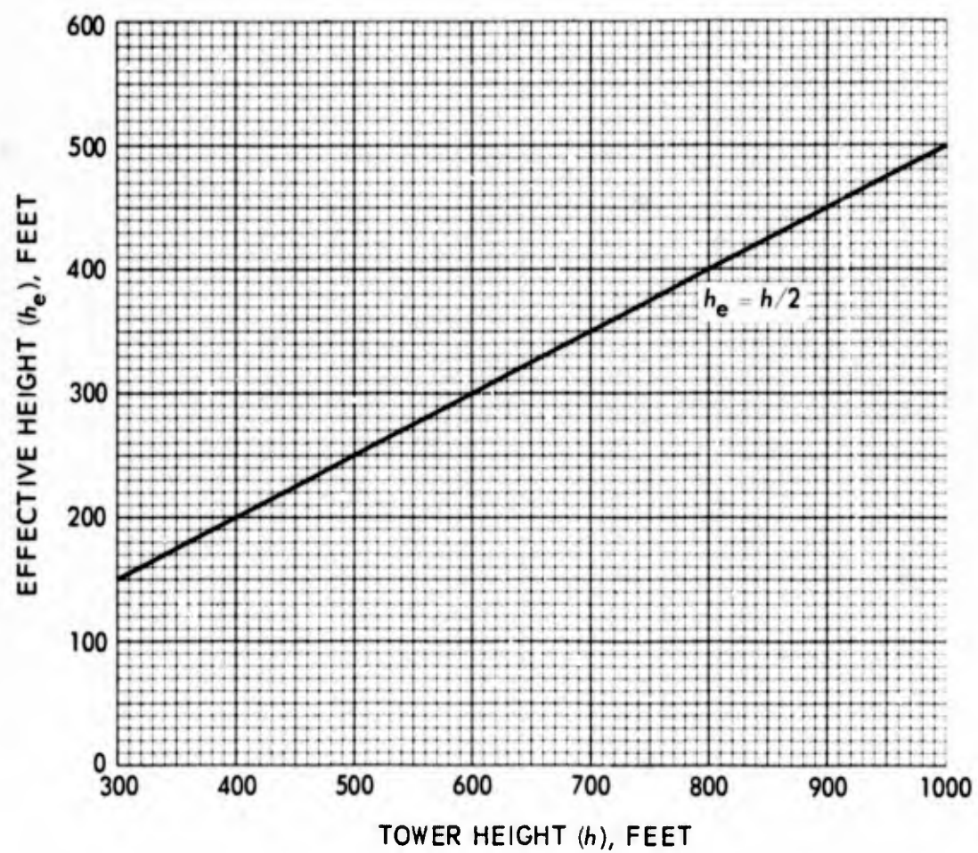
Figure 5. Variation of effective height of reference antenna with tower height ( h/d=200 ).
