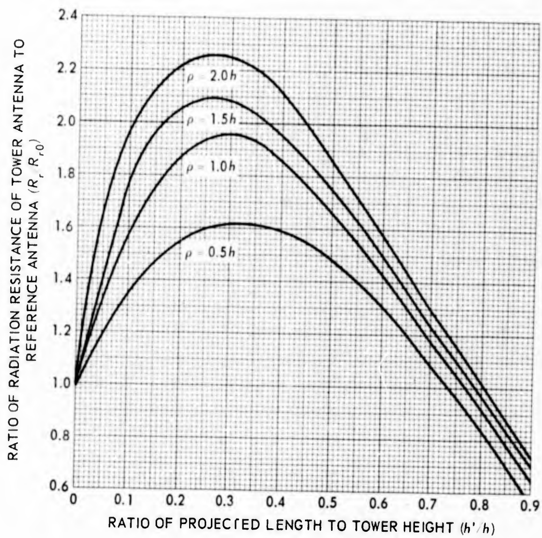
Figure 27. Normalized radiation resistance of top-loaded antenna, N=24 .
