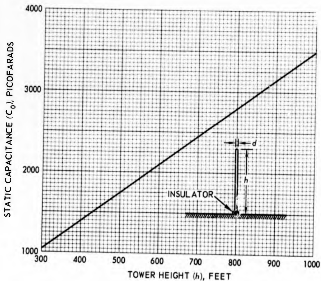
Figure 3. Variation of static capacitance of reference antenna with tower height ( h/d=200 ).
