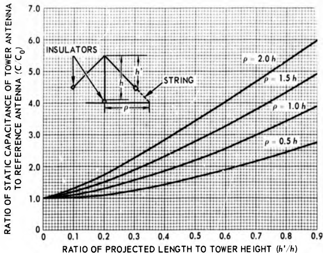
Figure 10. Normalized static capacitance of top-loaded antenna, N=6 .
