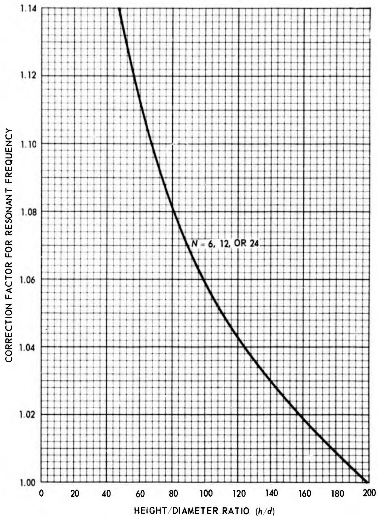
Figure 36. Correction factor for resonant frequency \rho = h .
