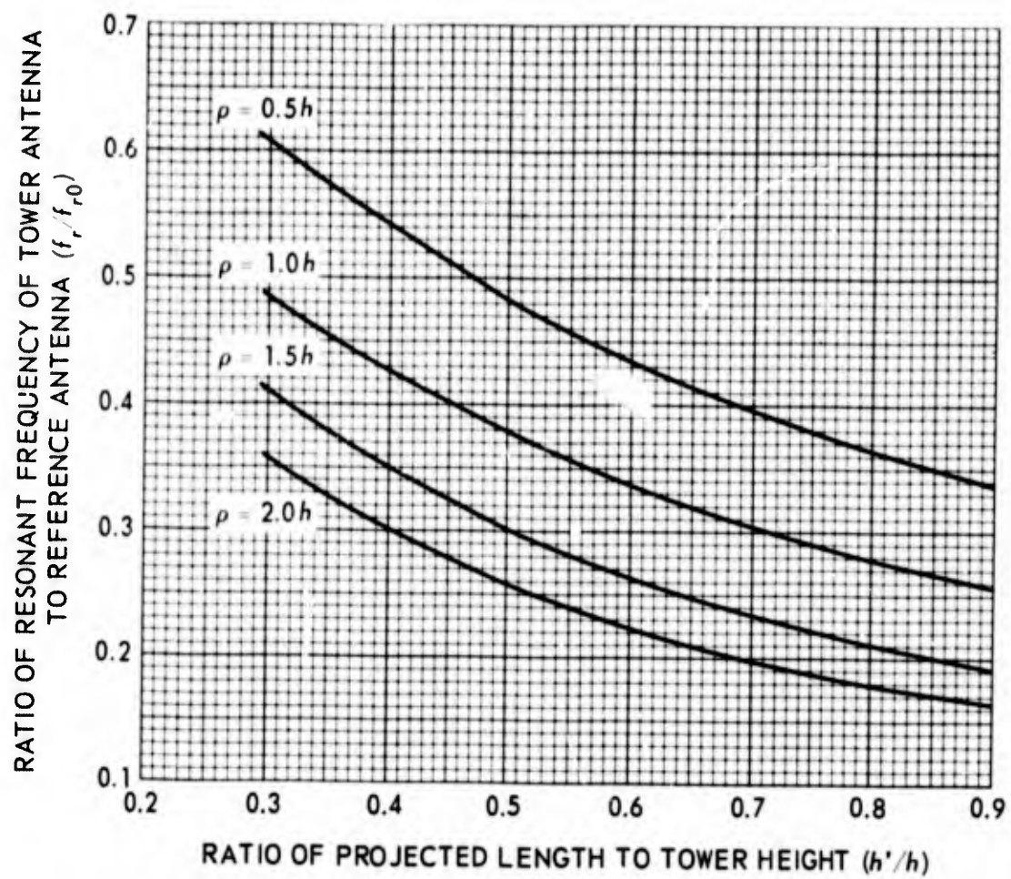
Figure 25. Normalized resonant frequency of top-loaded antenna, N=24 .
