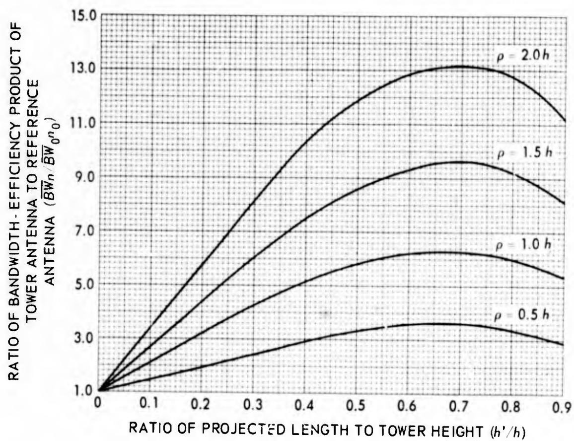
Figure 28. Normalized bandwidth-efficiency product of top-loaded antenna, N=24 .
