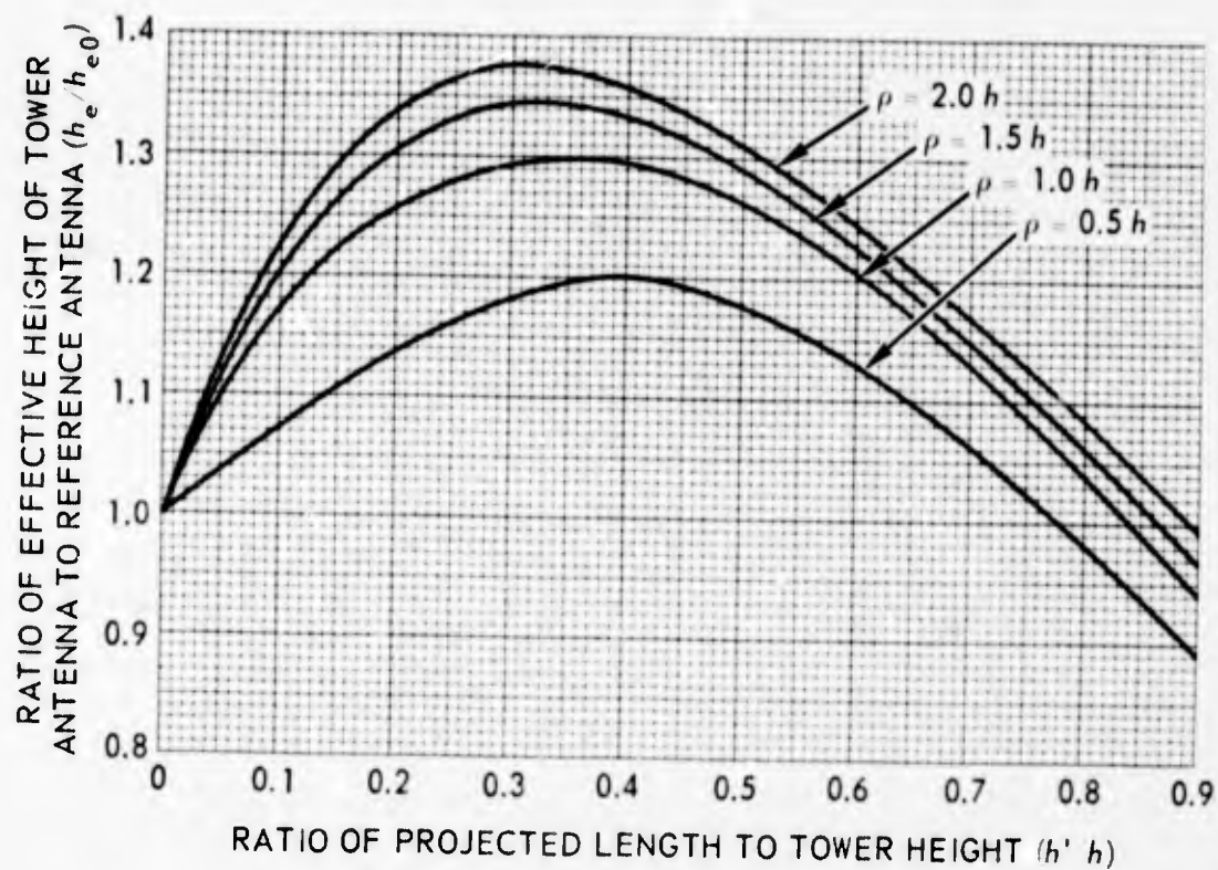
Figure 12. Normalized effective height of top-loaded antenna, N = 6 .
