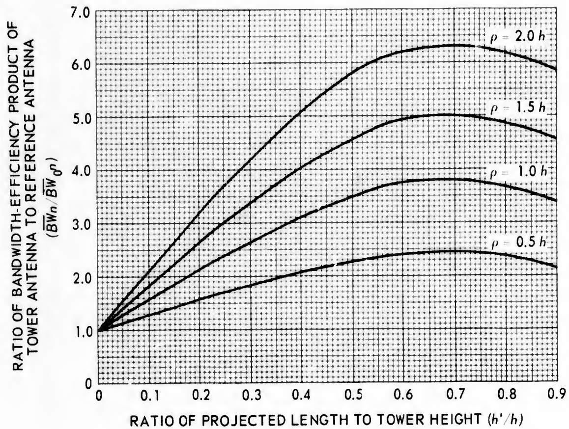
Figure 14. Normalized bandwidth-efficiency product of top-loaded antenna, N=6 .
