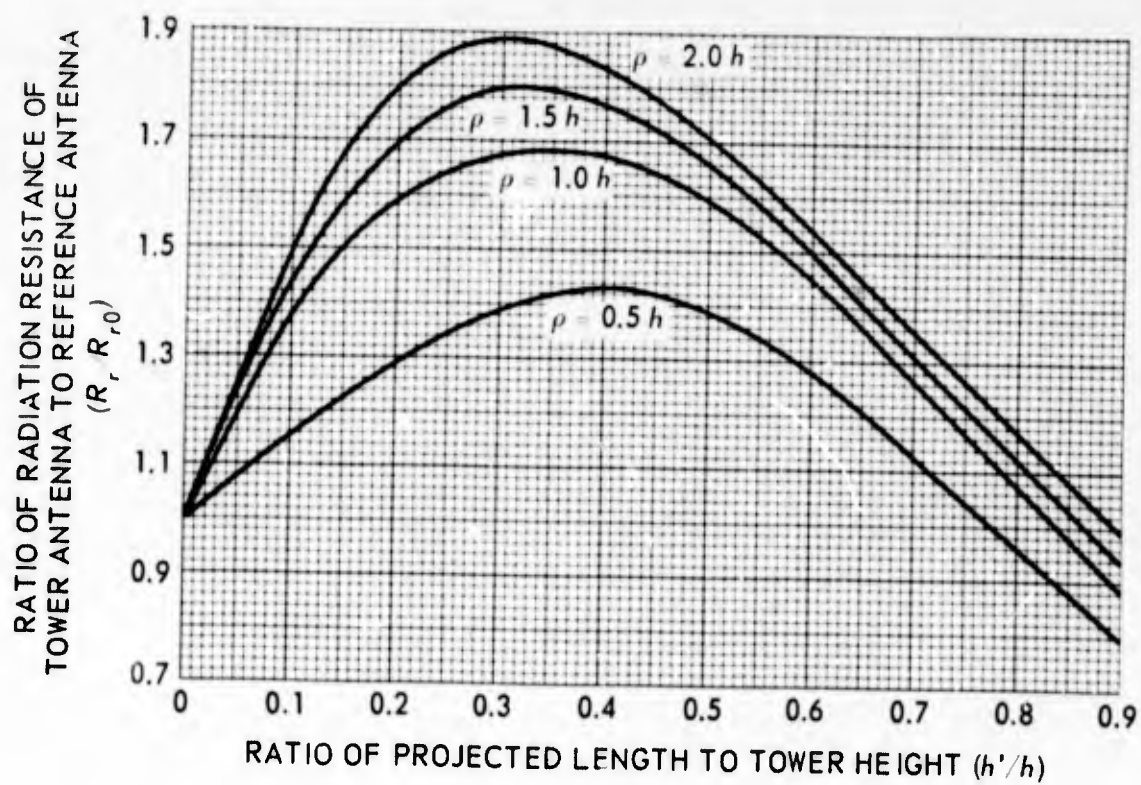
Figure 13. Normalized radiation resistance of top-loaded antenna, N = 6 .
