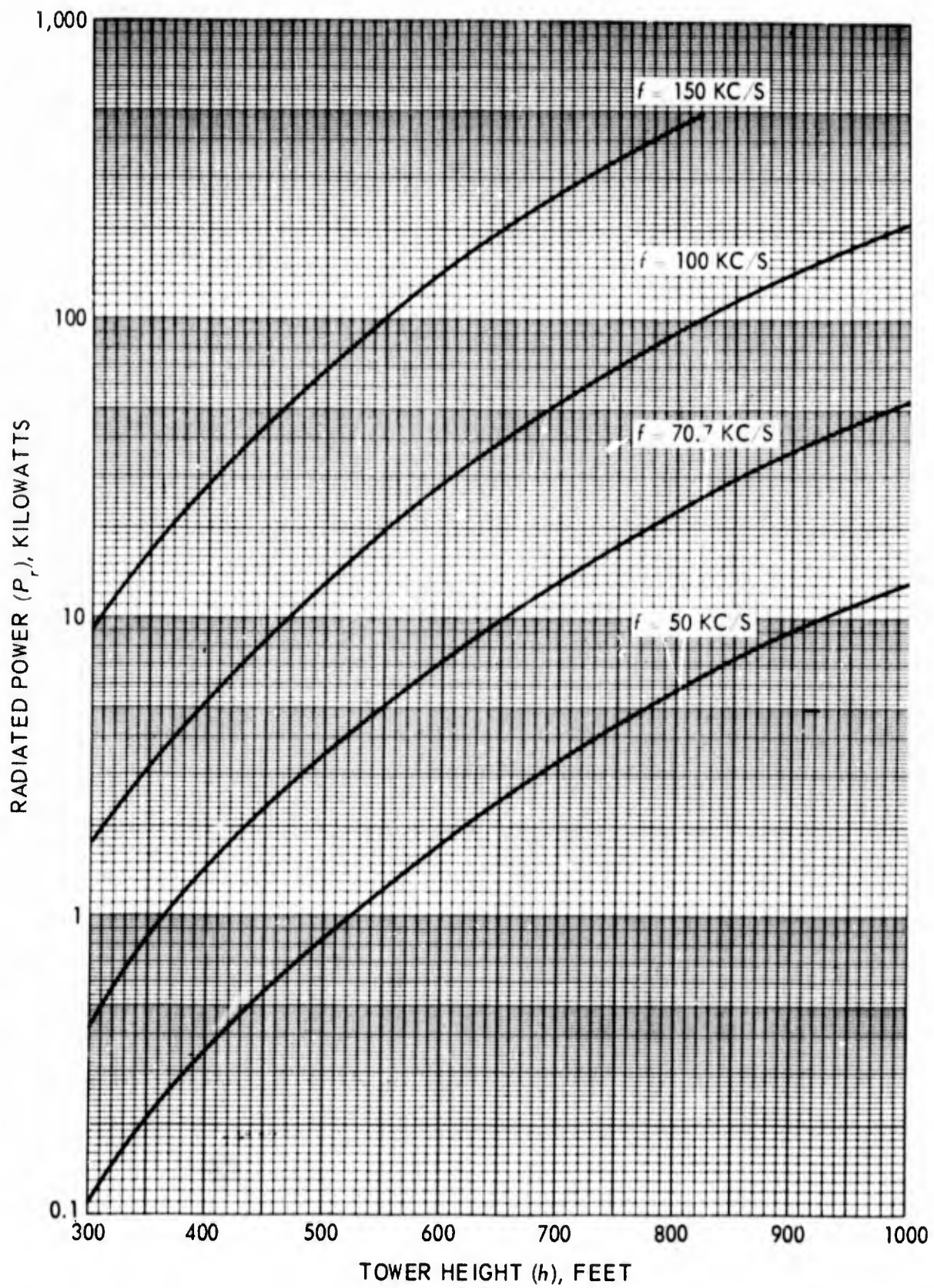
Figure 8. Variation of reference tower maximum radiated-power capability with tower height ( h/d = 200 ).
