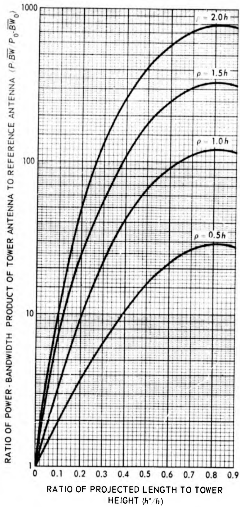
Figure 23. Normalized power-bandwidth product of top-loaded antenna, N = 12 .
