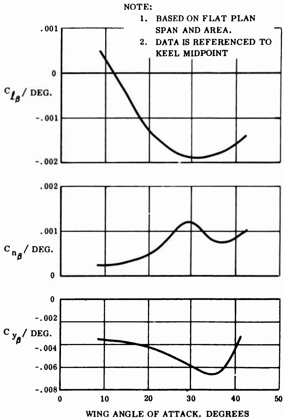
Figure 42. Lateral-Directional Static Stability, Wing Only
