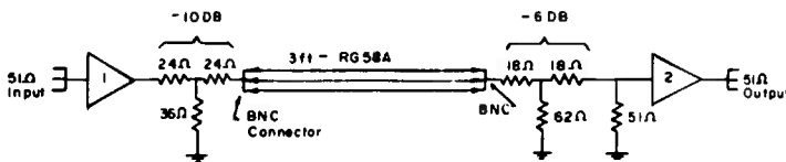
Figure 20. Attenuator and Amplifier Configuration
