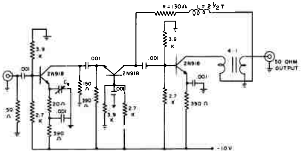
Figure 17. Circuit of Wideband Transistor Amplifier Referred to as the BABB (Basic Amplifier Building Block)
