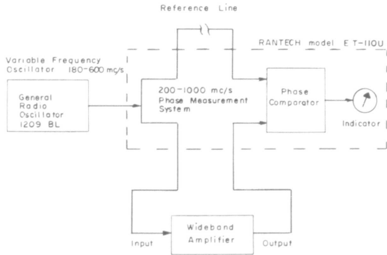
Figure 36. Phase Measurement Technique
