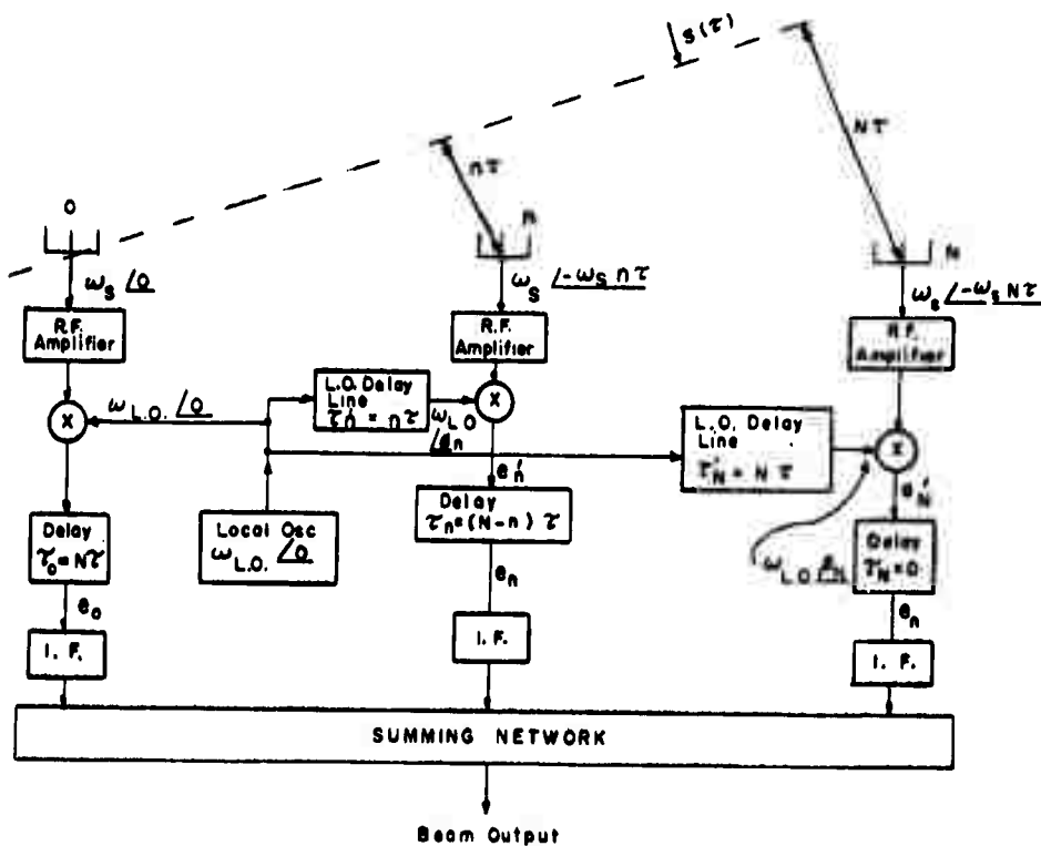
Figure 6. Wideband I-F Time Delay Beam Steering
