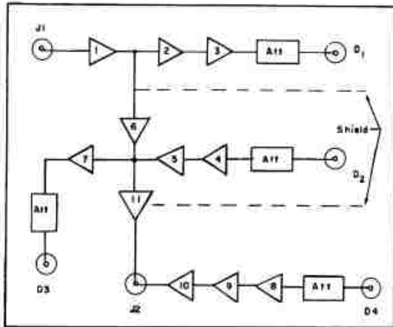
Figure 25. Physical Layout of Two-Bit Digital Delay Line
