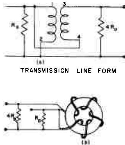
Figure 38. Wiring Diagram for 4:1 Impedance Transformer
