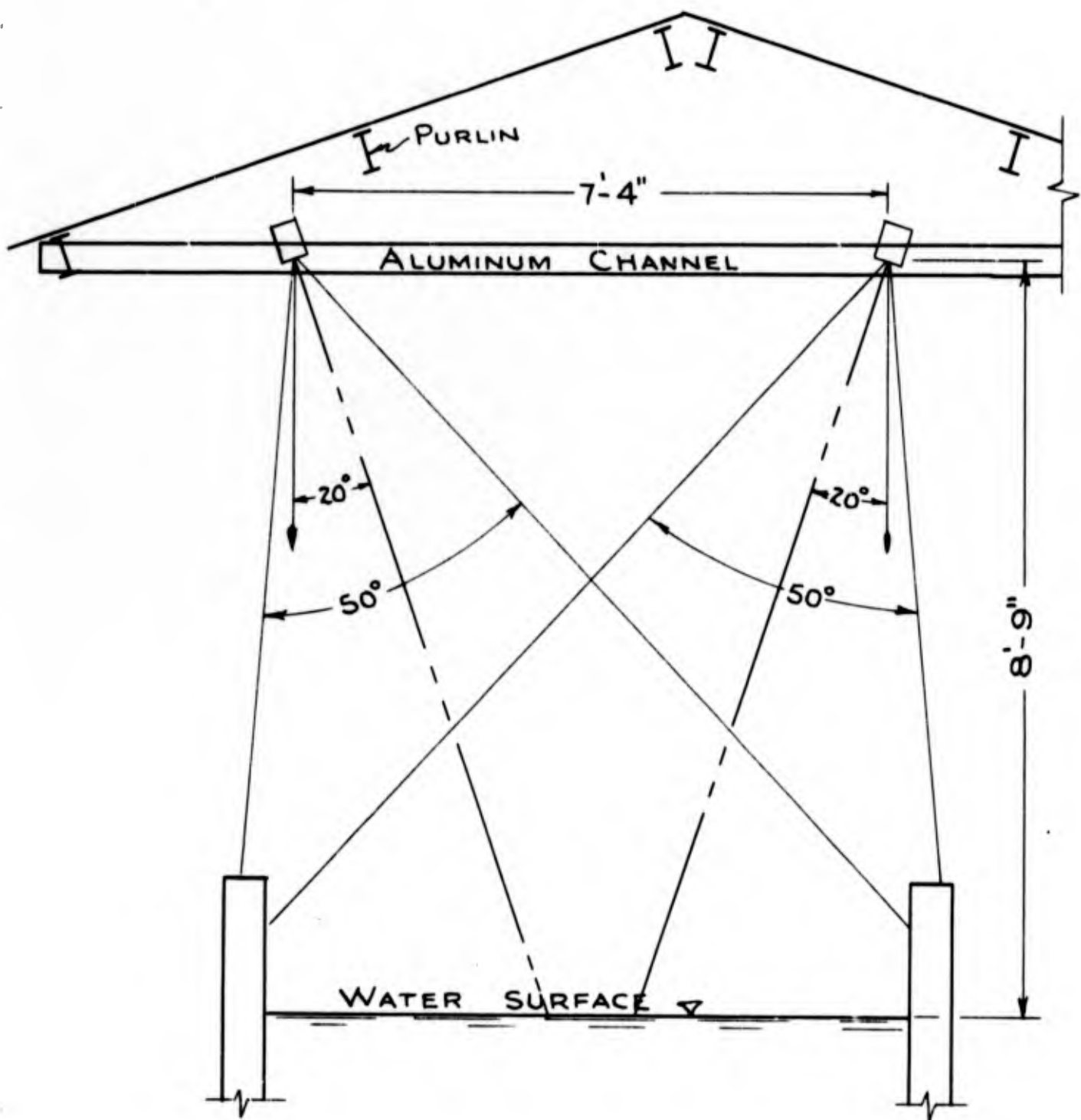
Fig. 4. Camera arrangement in towing tank.
