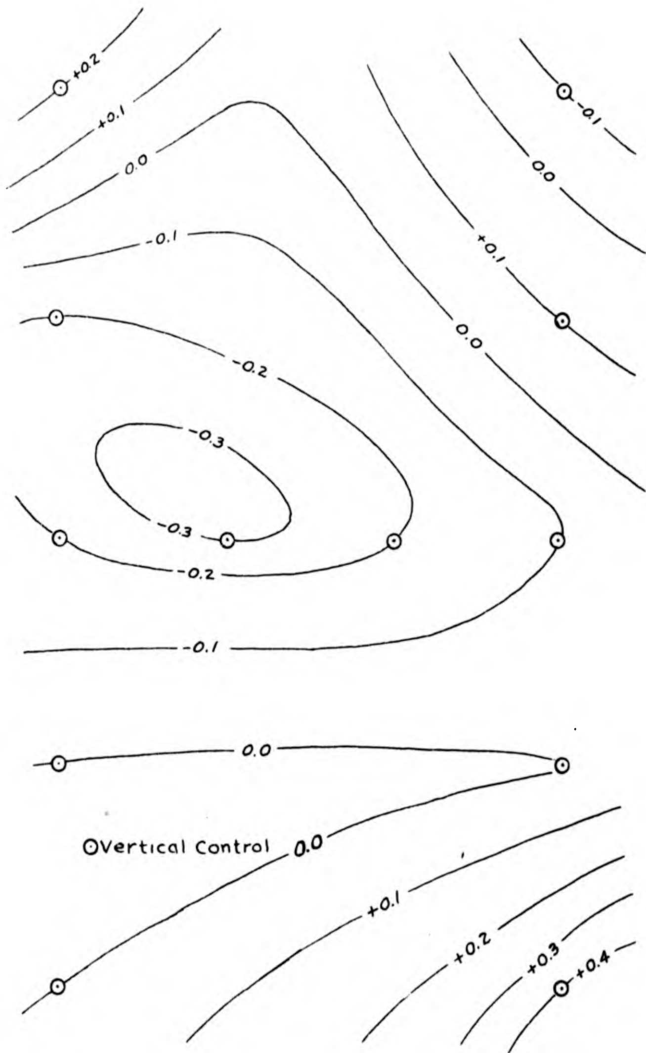
Fig. 13. Correction diagram-Second high-speed run.
