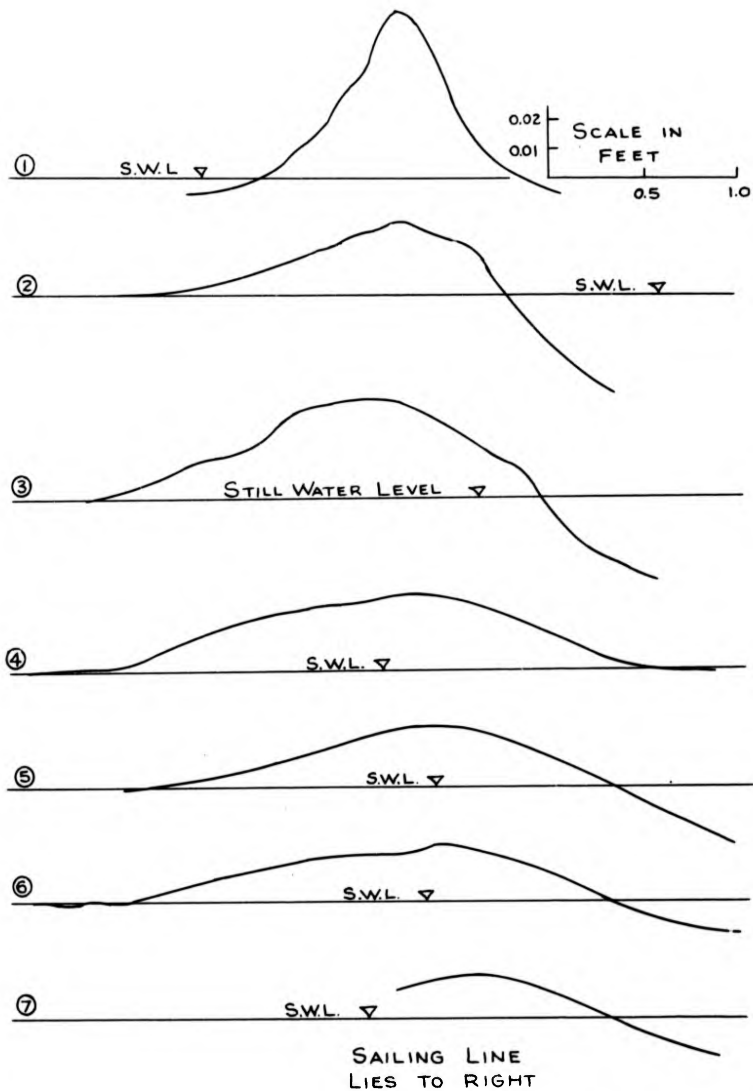
Fig. 17. Crest profiles - Ship model speed = 3.20 ft./sec.
