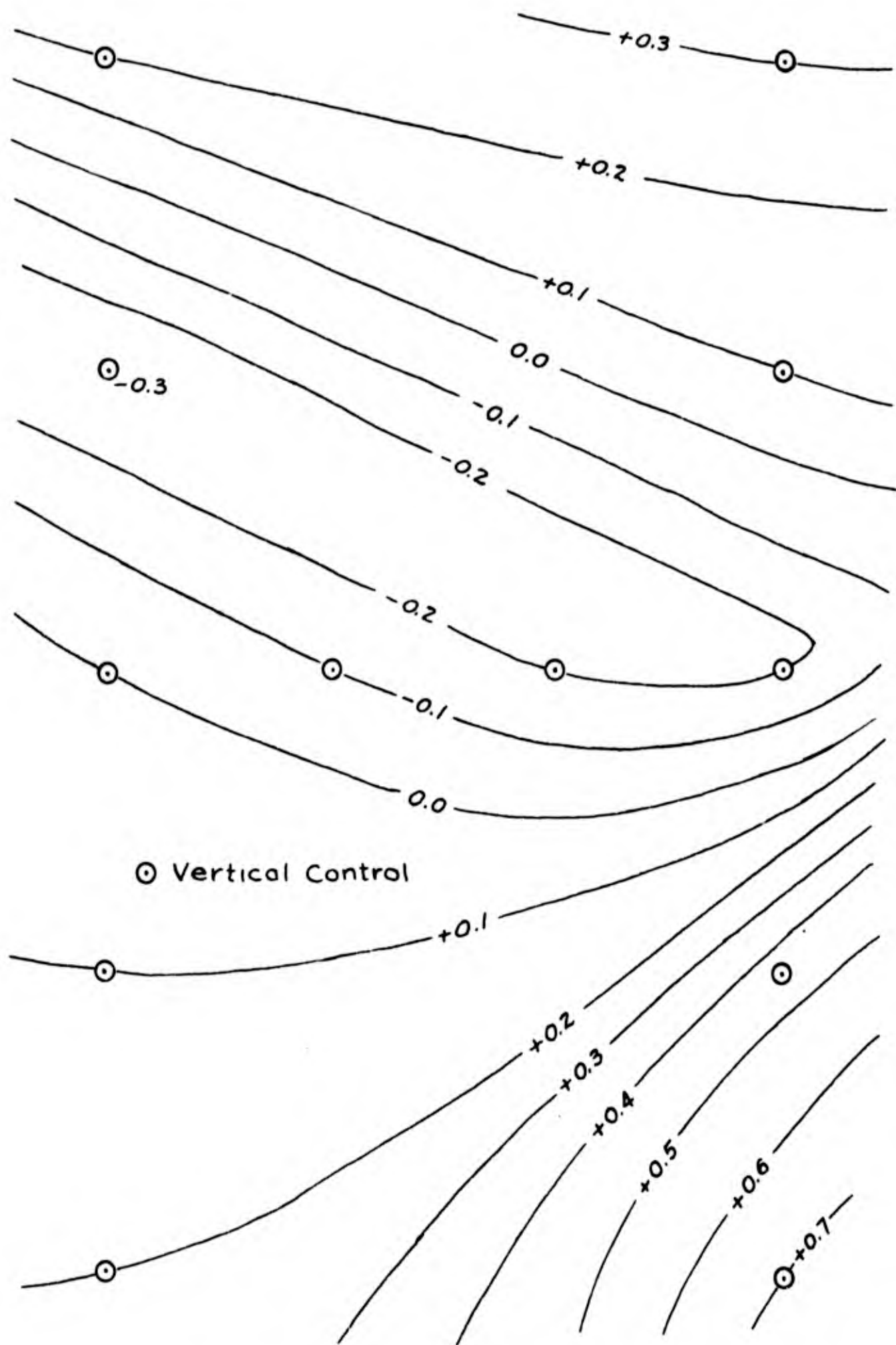
Fig. 12. Correction diagram - Second low-speed run.
