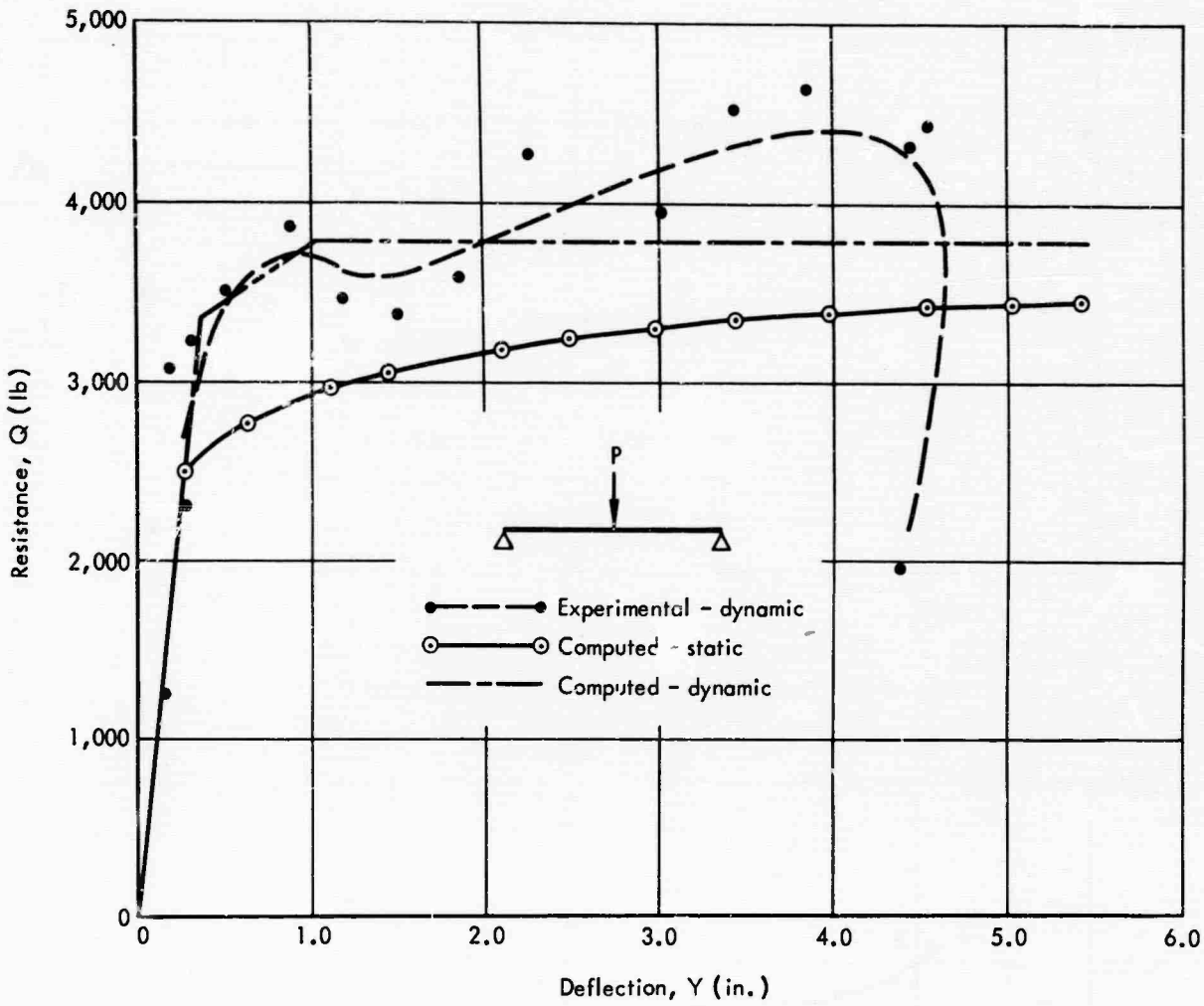
Figure 46. Resistance versus deflection - Beam C-9.
