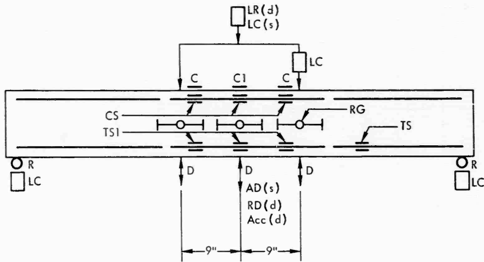
(b) Beams with a = 18''
