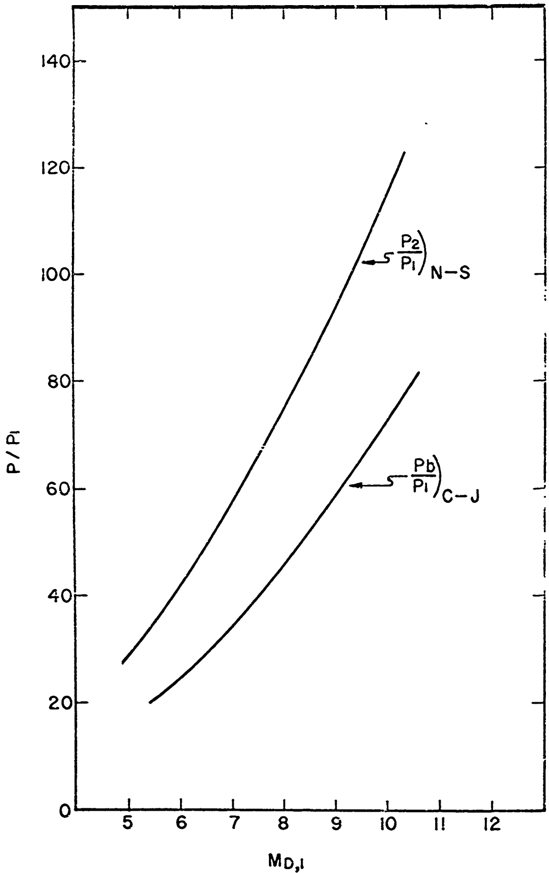
Figure 35 The Theoretical Variation of the Pressure Ratio of a Detonation Wave Versus Mach Number for Flows Against a Supersonic Stream
