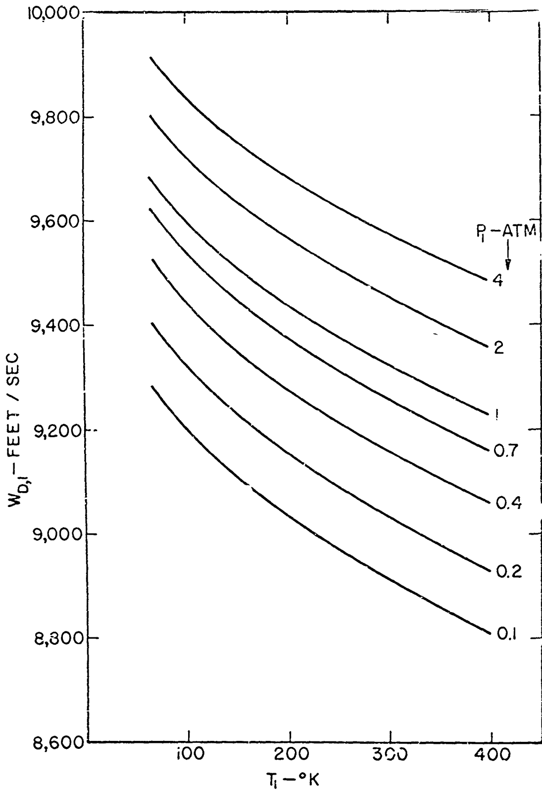
Figure 19 The Theoretical Variations of the Absolute Chapman-Jouguet Detonation Wave Velocity with Initial Temperatures at Constant Initial Pressures for a Stoichiometric Mixture of Hydrogen-Oxygen
