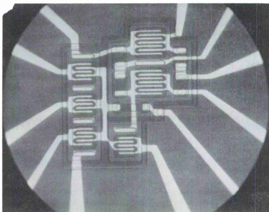
b. Photomicrograph (M = 300X).
