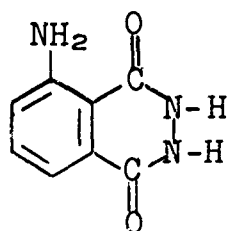
Luminol
