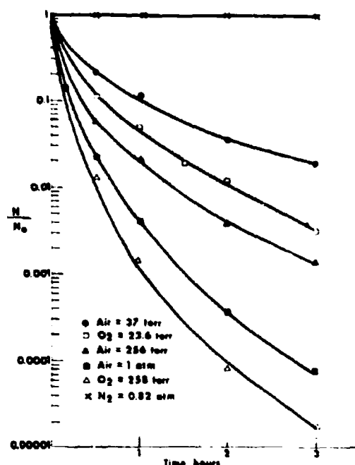
FIG. 4. Semi-log plot of survival versus time after exposure of lyophilized Serratia marcescens to various pressures of oxygen, dry air, or purified nitrogen. N_0 and N are the number of viable organisms before and after the exposure, respectively.
