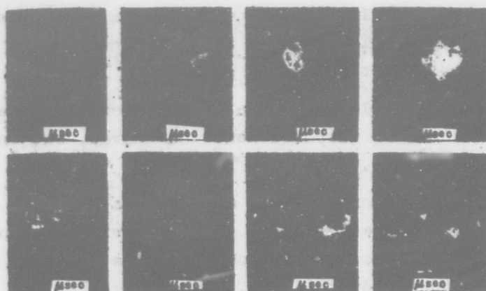
Fig. 4.49. Sample of photographs of detonation, obtained with the help of SFR-2 in a variant of time beams. The charge is in the form of a parallelepiped 30 \times 76 \times 120 mm. The lens is turned to the side 30 \times 76 . Photographs were produced in two microseconds. Imprints are given for the moments 8, 16, 24, 32, 48, 64, 80, 96 microseconds from the beginning of the explosion. Initiation is from above (in the middle). Below is a scale rule. The big division (light section of the biggest length) is 150 mm.
