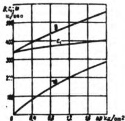
Fig. 6.5. Parameters of shock waves in air with values of \Delta p up to 2 \text{ kg/cm}^2 .
