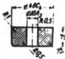
Fig. 4. Directing bushing.
