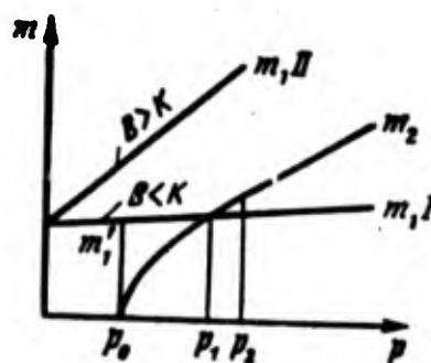
Fig. 4.28. Dependence of gas influx m_1 during burning and gas bleeder m_2 on the pressure.
