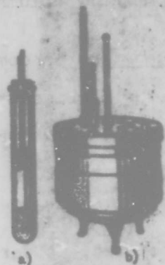
Fig. 3.11. Test tube (a) and bath (b) for test of explosive for stability by iodized starch sample.
