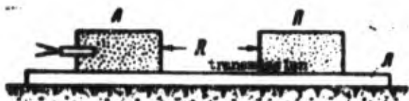
Fig. 6.11. Diagram of experimental determination of distance for the transmission of a detonation. A) active charge; B) passive charge; C) lining - "witness."
