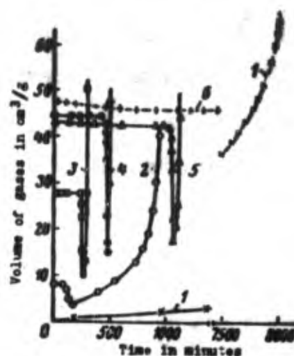
Fig. 2.20. Change in time of volume of gaseous products of disintegration of liquid nitroglycerine at 100°C in the presence of water vapors ( \delta \sim 6 \cdot 10^{-3} ). Pressure of water vapors in mm: 1 - 0; 2 - 116; 3 - 328; 4 - 447; 5 - 467; 6 - 471.
