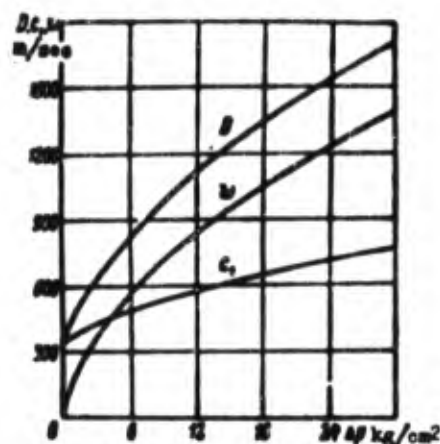
Fig. 6.6. Parameters of shock waves in air with values of \Delta p from 2 to 30 \text{ kg/cm}^2 .
