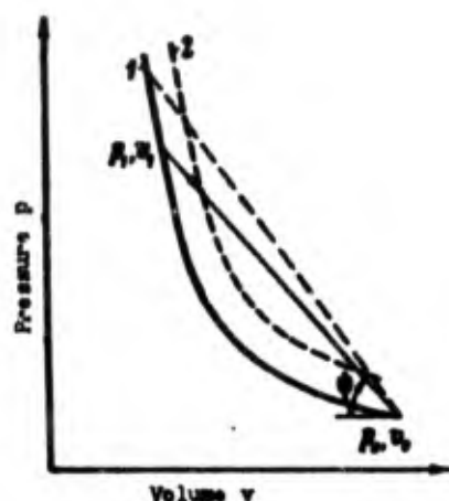
Fig. 4.57. Measurement of the state on the diagram p - v by means of passage of the reaction. 1) shock adiabat for initial explosive; 2) the same, for the condition, when part of the explosive has already reacted.
