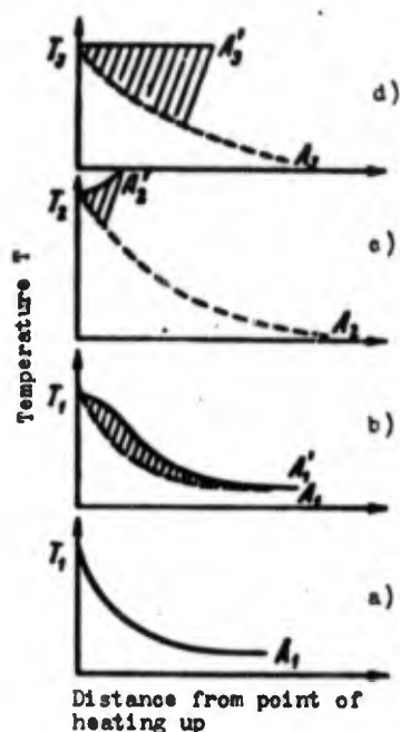
Fig. 2.6. Diagram of thermal ignition according to Vant-Hoff.
