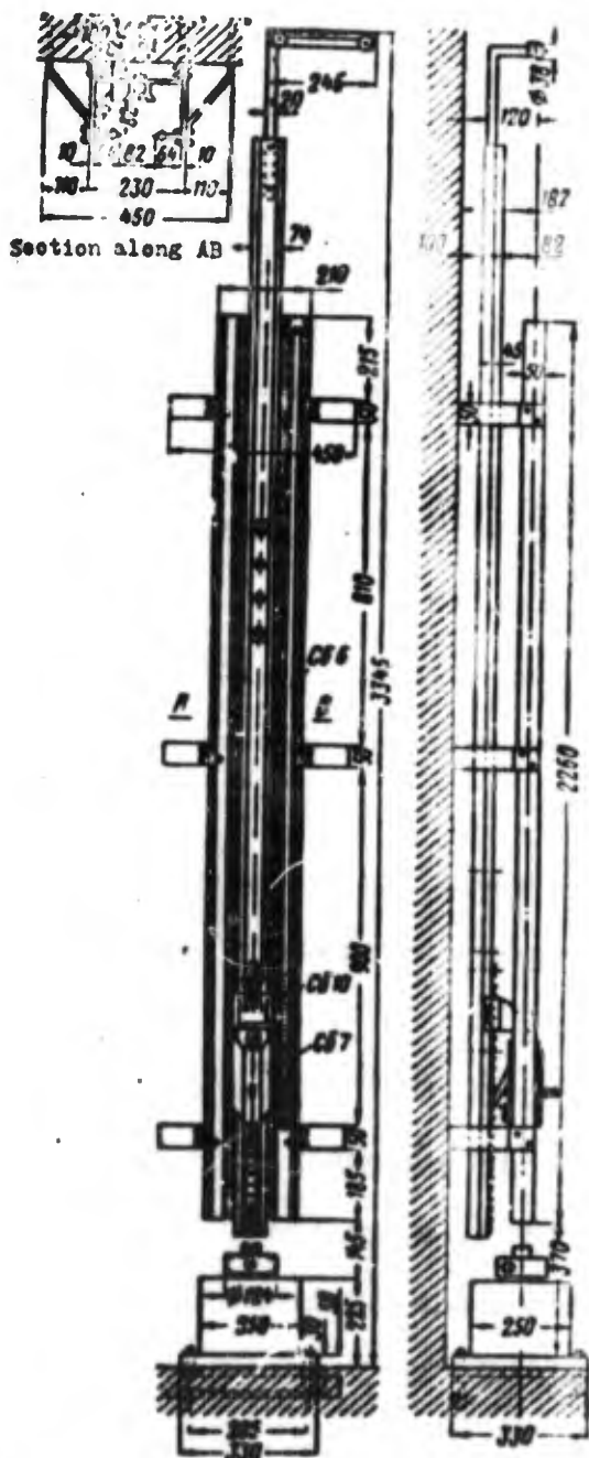
Fig. 1. Kast drop hammer. [C6 = Sb (unidentified)]
