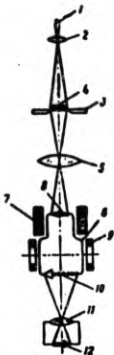
Fig. 4.53. Diagram of determination of the speed of detonation with the help of an electron-optical converter. 1 - charge; 2 - lens; 3 - slot; 4 - intermediate image in plane of the slot; 5 - second lense; 6 - tube of electron-optical converter; 7 - magnetic lens; 8 - second image on light sensitive cathode; 9 - deflecting coverings, giving unfolding in time; 10 - electron image on screen of converter; 11 - lense of camera; 12 - image on photographic film.
