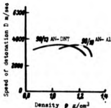
Fig. 4.42. Dependence of the speed of detonation of mixtures of ammonium nitrate (90%) with dinitrotoluene (10%) or aluminum (10%) on the density with a small (10 cm) diameter of charge.
