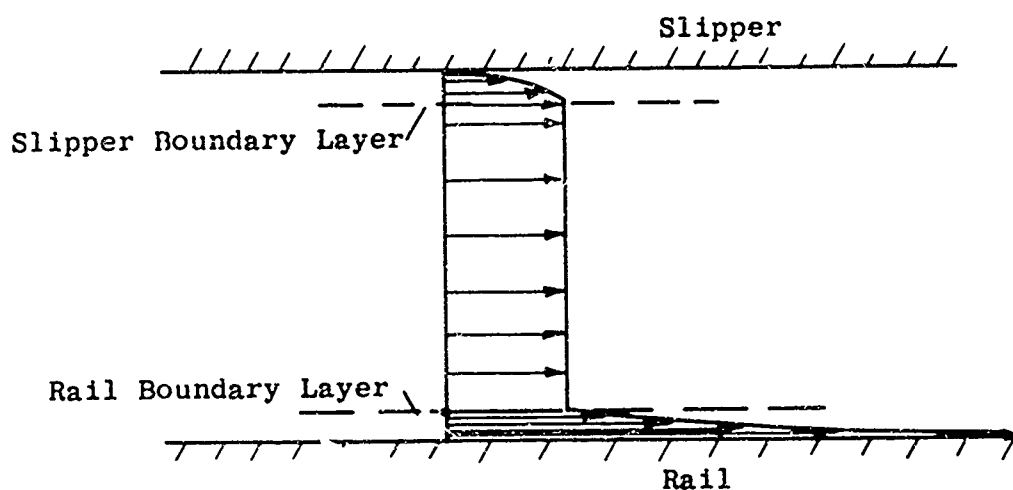
(a) Near Transition From Laminar to Turbulent Flow
