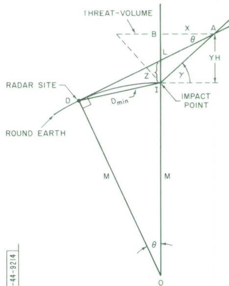
Fig. E-1. Limiting coverage geometry for point impact zone.
