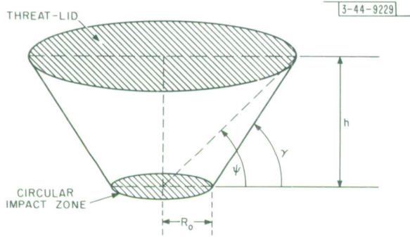
Fig. 11(b). Threat-volume geometry showing angular variation for Eq. (17).
