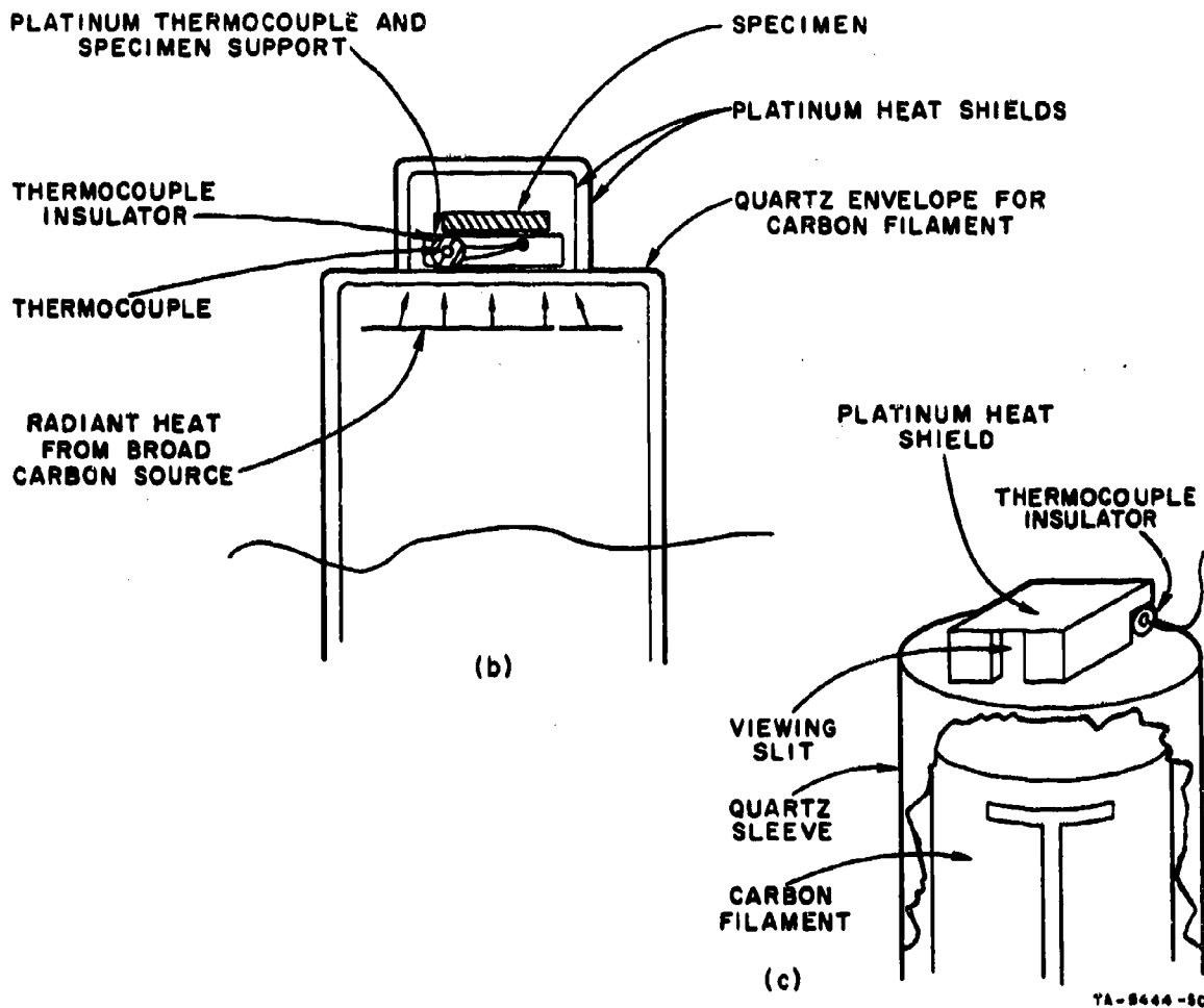
FIG. 1 VACUUM STATION
