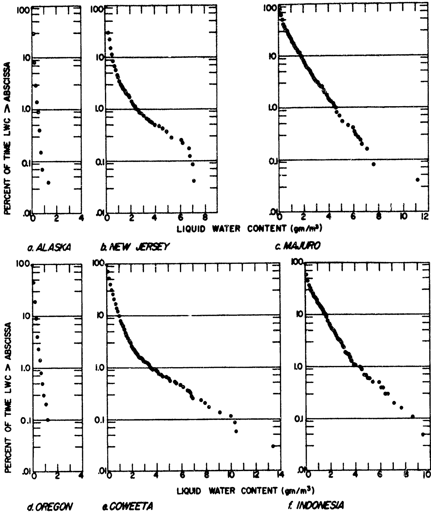
FIG.26 LIQUID WATER CONTENT FREQUENCY DISTRIBUTIONS
