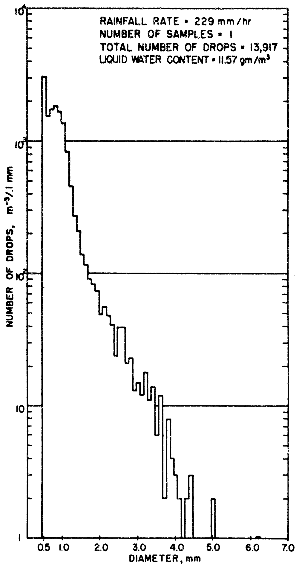
Fig. 8 ONE-MINUTE SAMPLE OF LARGEST TOTAL NUMBER OF DROPS AT MIAMI, 1105 EST, JUNE 21, 1958
