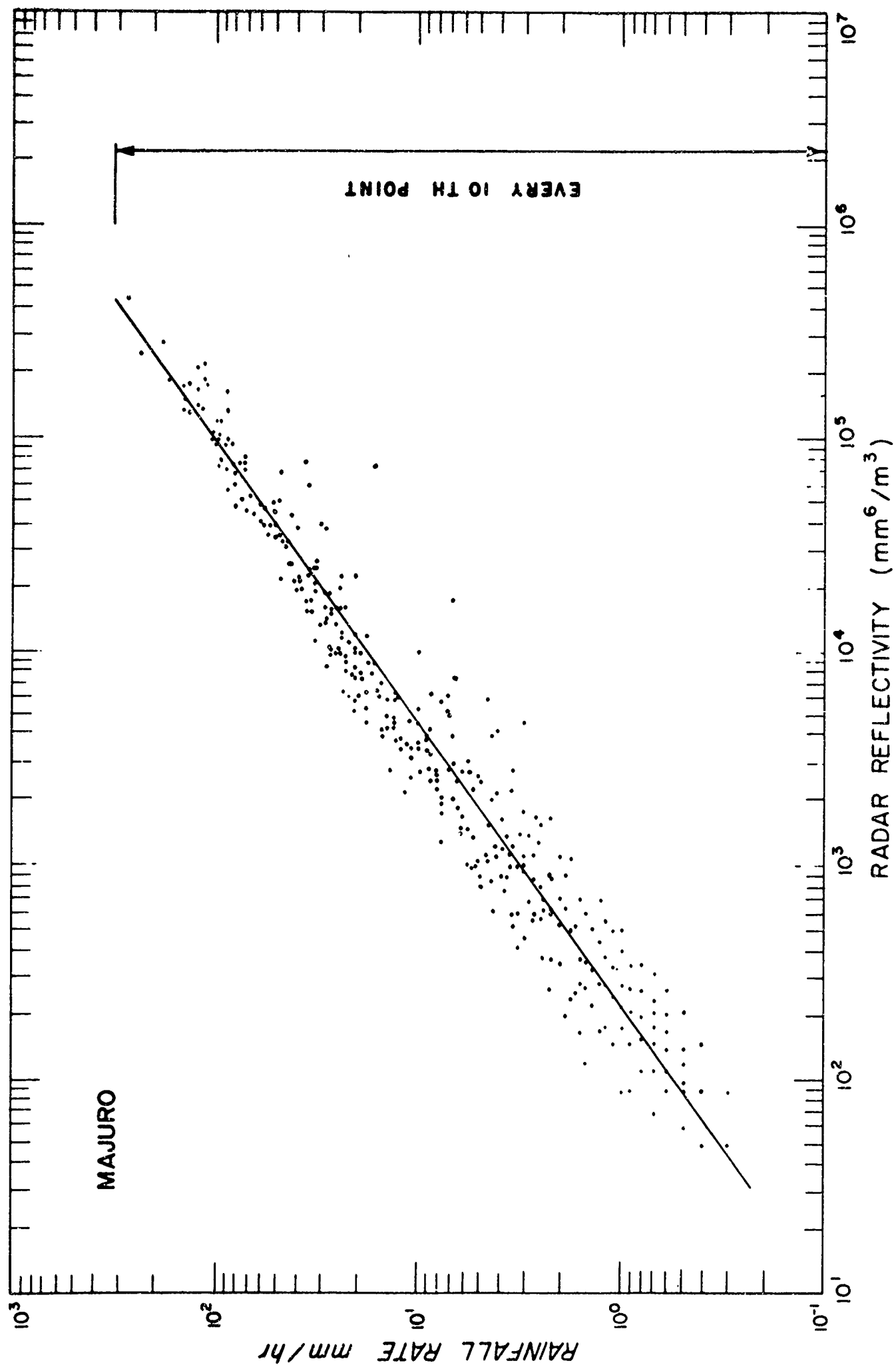
FIG. 20 RAINFALL RATE - RADAR REFLECTIVITY SCATTERGRAM FOR MAJURO DATA
