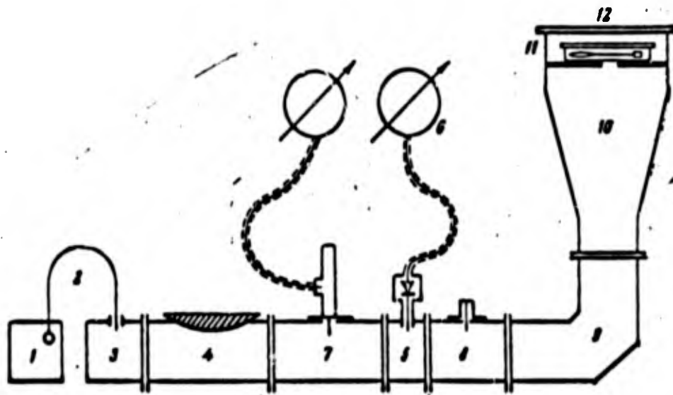
Fig. 2. Device for irradiating neuromuscular preparations with measured doses of microwave power
