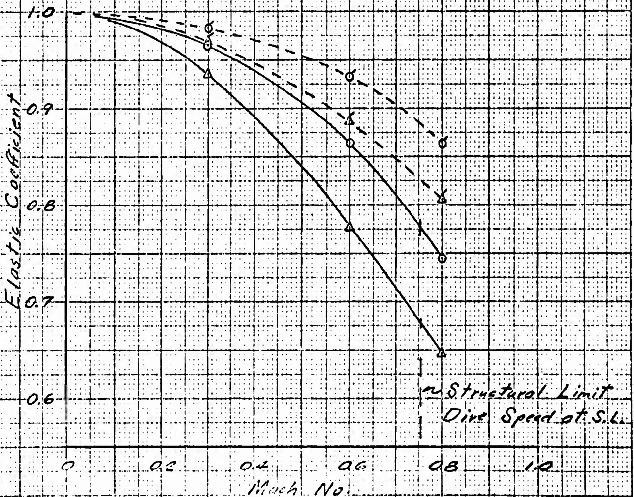
Figure 4.77 Empennage Elastic Coefficients, Pitching Mode
