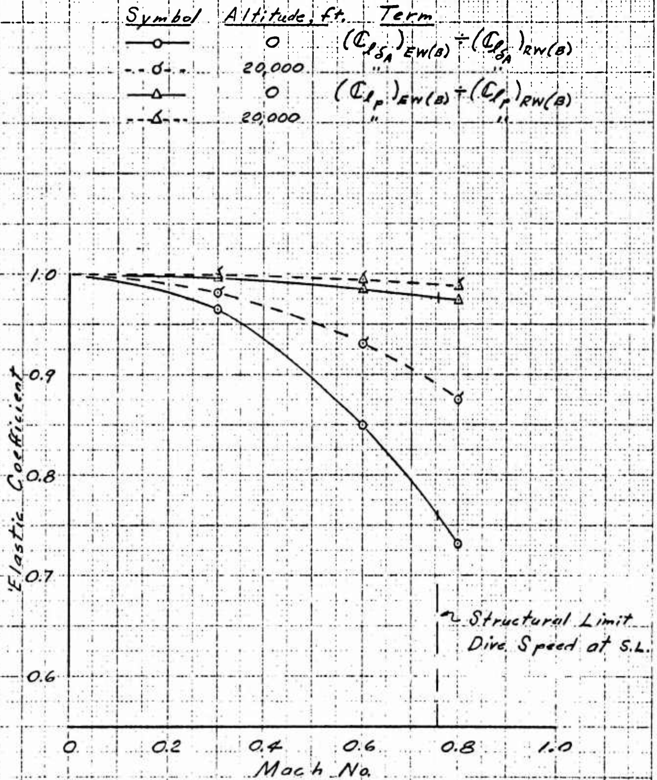
Figure 4.76 Wing - Body Elastic Coefficients, Rolling Mode
