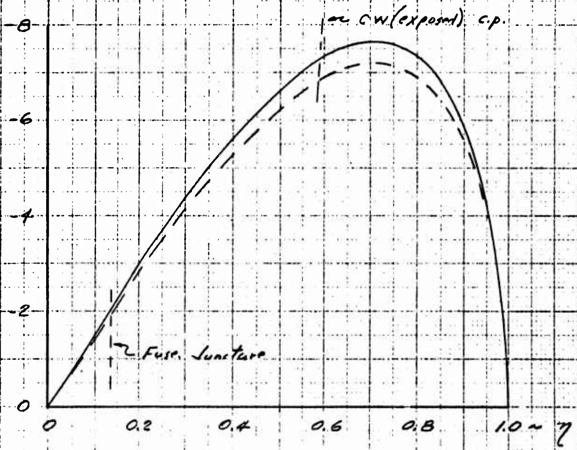
Figure 3.27 Loading Distribution Due to Rolling Velocity
