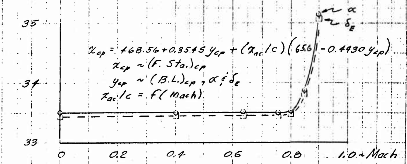
Figure 3.53 Horizontal Tail Loading Characteristics Due to \alpha \delta_E & \phi - Types of Loading
