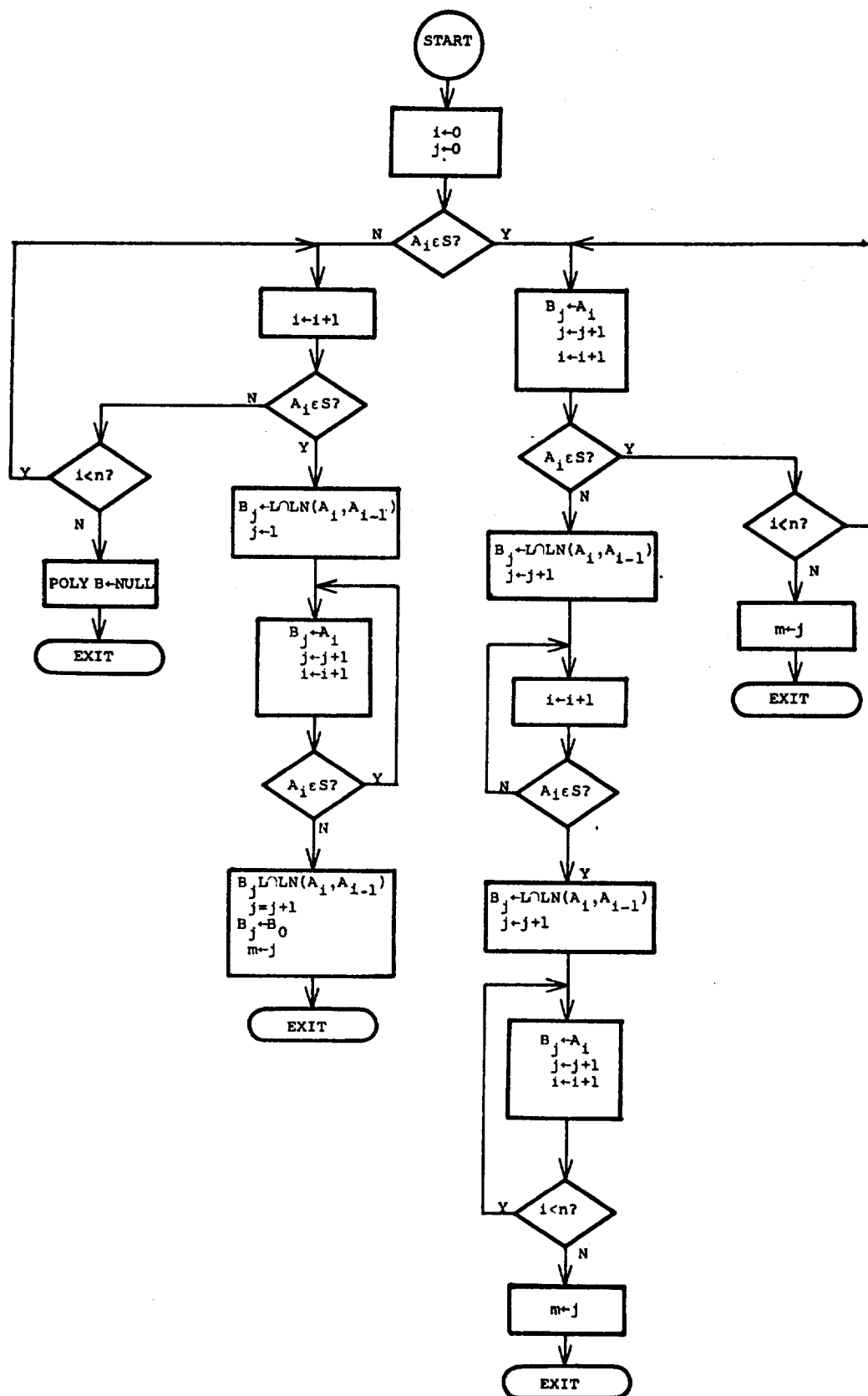
FIGURE 5 - FLOW DIAGRAM OF POLYGON INTERSECTION ALGORITHM
