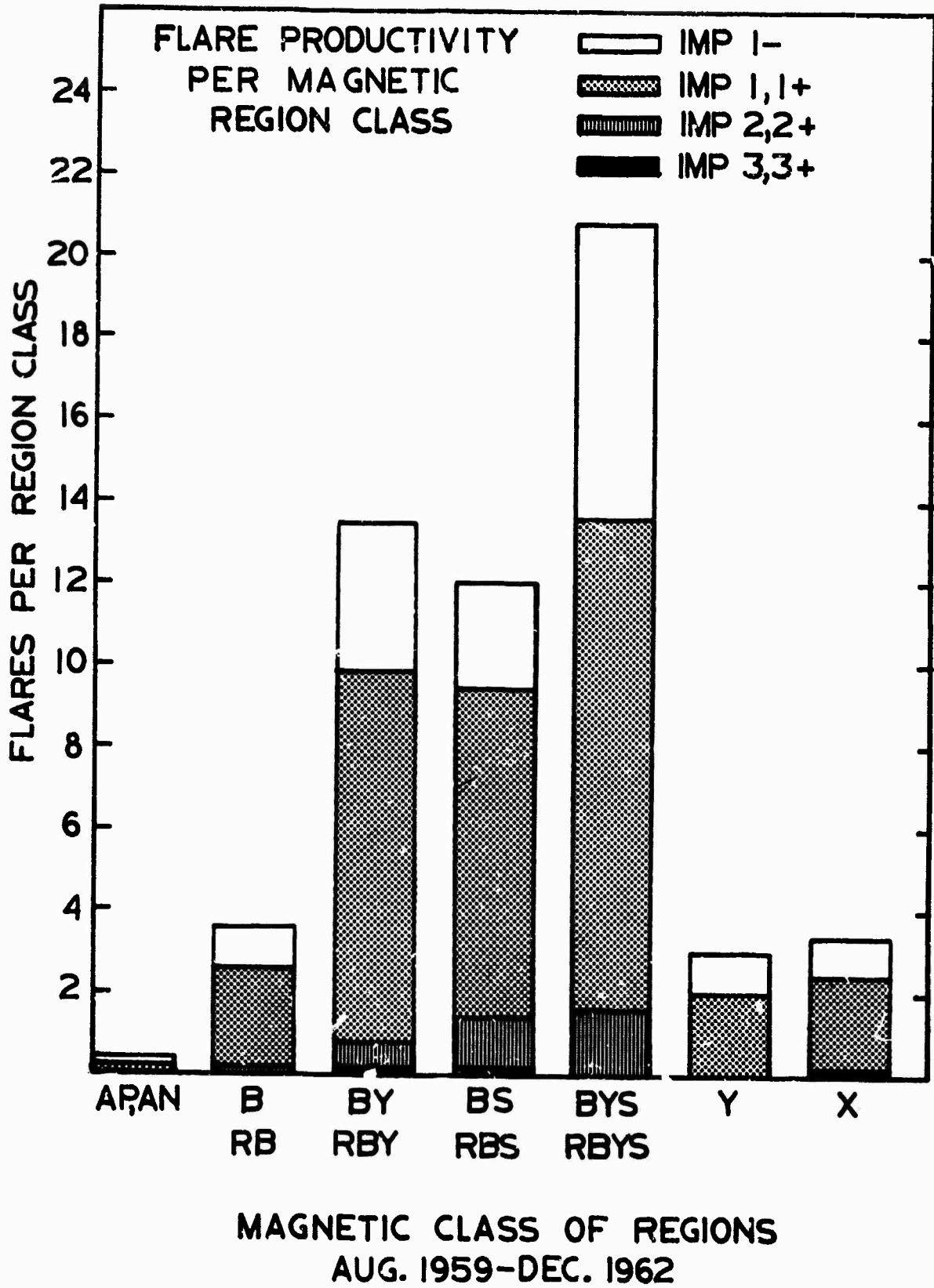
Figure 9. The Most Flare-productive Classes are Also the Most Complex Bipolar Magnetic Regions. The Most Complex Class, Y, However, A pears to be no More Flare-productive than the Simple Bipolar Regions.
