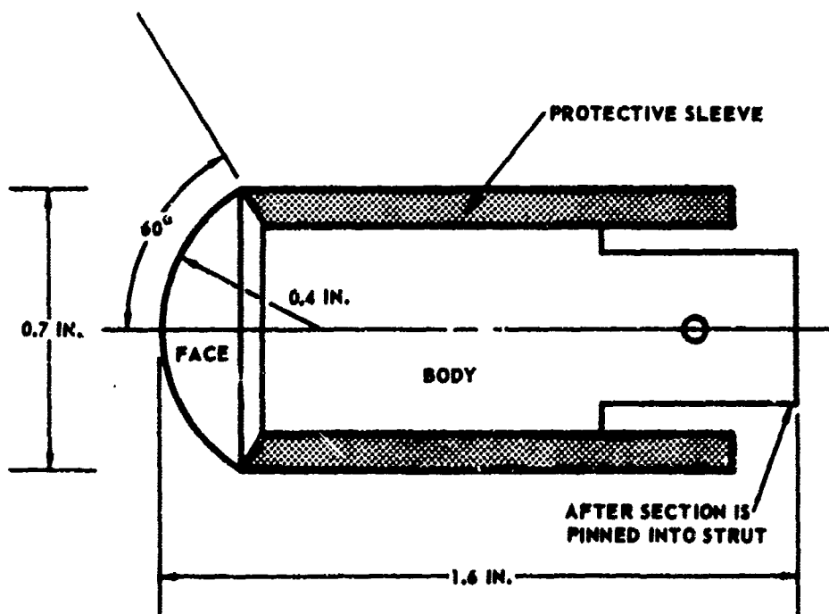
Fig. 2 TYPICAL TEST MODEL
