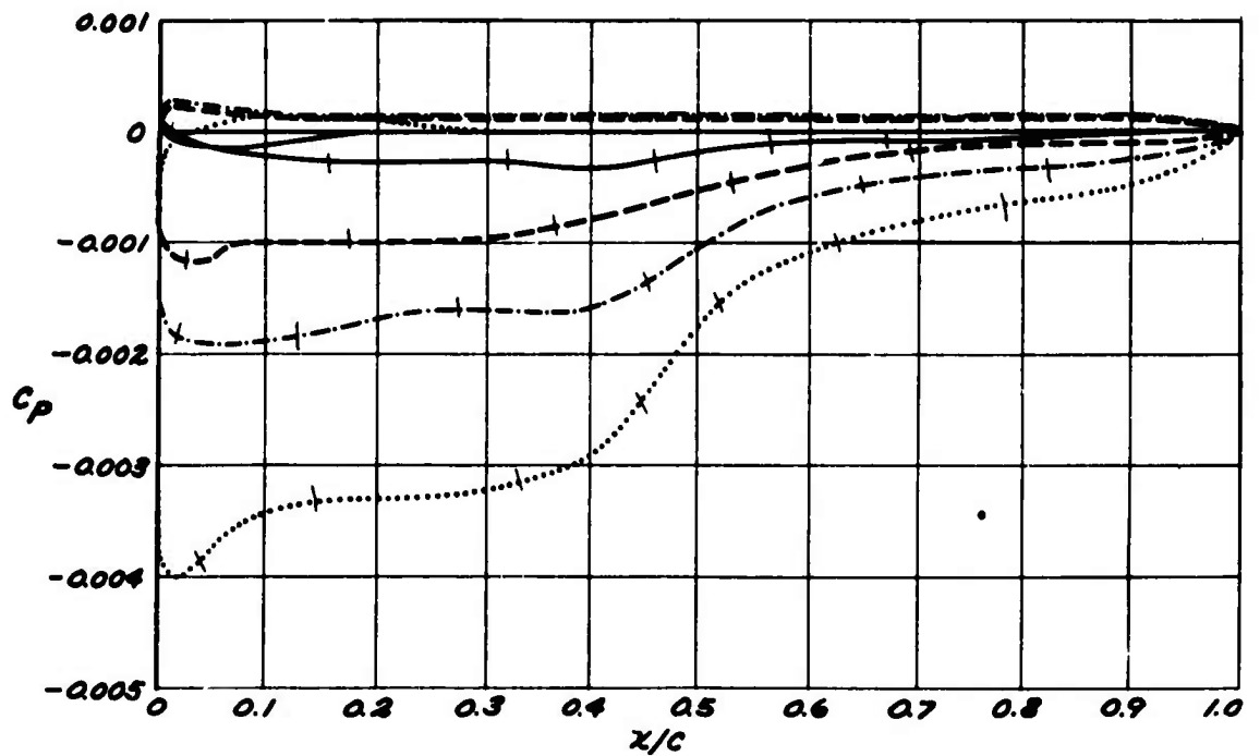
Figure 19-b. Shroud Pressure Distribution - Forward Motion, 4000 RPM, 10 MPH.
