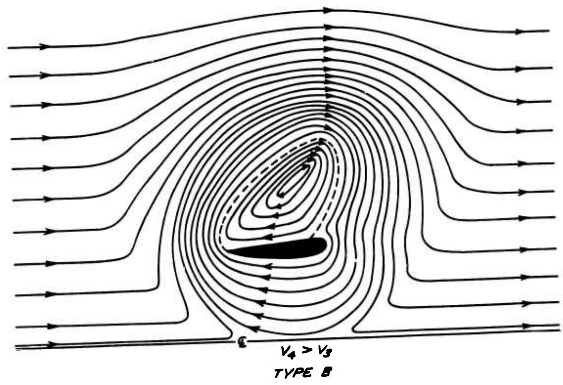
Figure 15-b. Flow Patterns - Rearward Motion.
