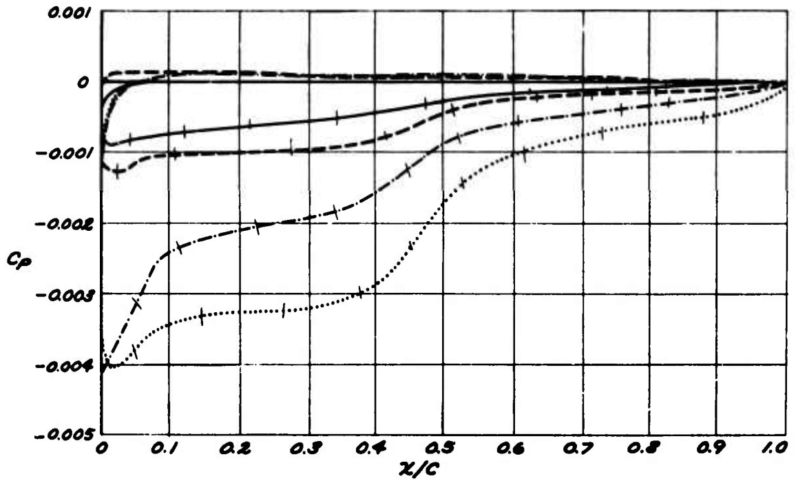
Figure 19-a. Shroud Pressure Distribution - Forward Motion, 4000 RPM, 5 MPH.
