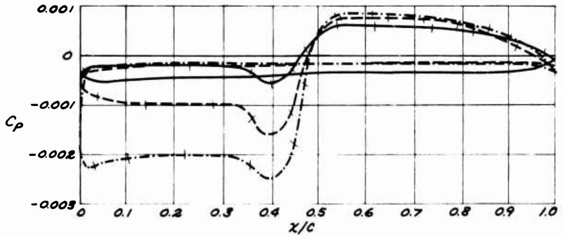
Figure 12-k. Shroud Pressure Distribution - Rearward Motion, 4500 RPM, 25 MPH.
