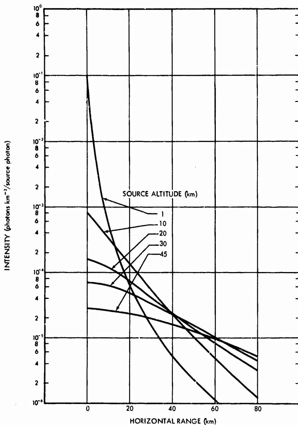
Fig. 32. Total Intensity vs Horizontal Range for Several Source Altitudes: 0.45\mu Light, Receiver Altitude = 0.1Km, Ground Albedo = 0.0
