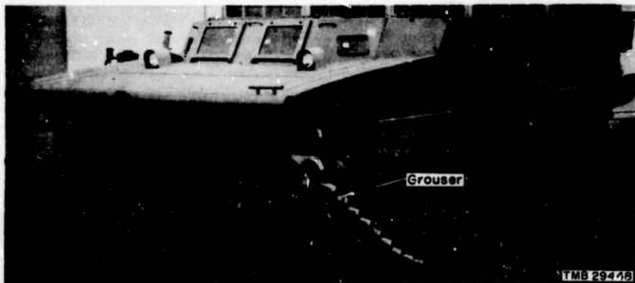
Figure 1 - Photograph of Amphibian Tractor Showing Grousers
