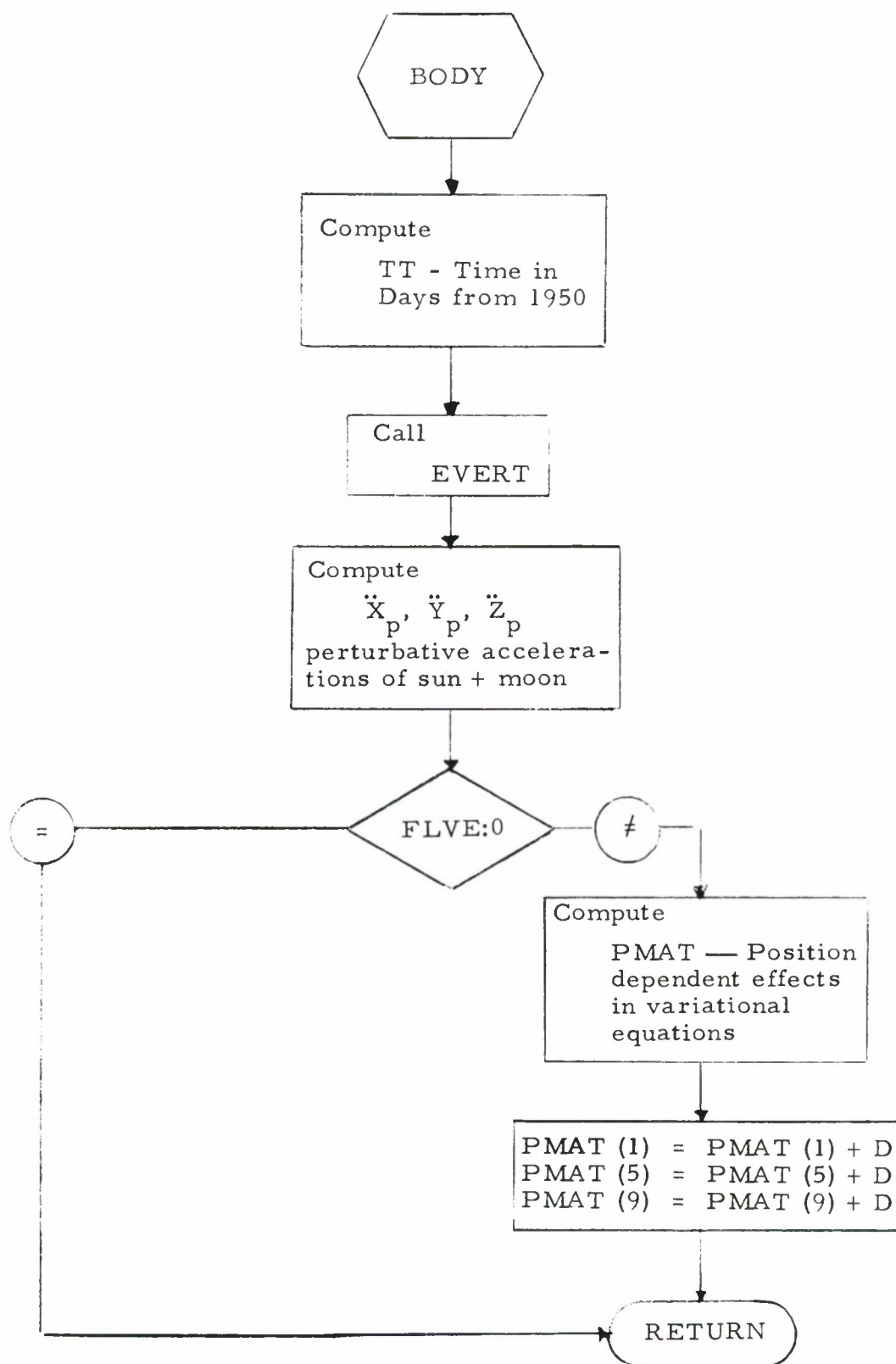
Figure 5-2. BODY Flow Diagram
