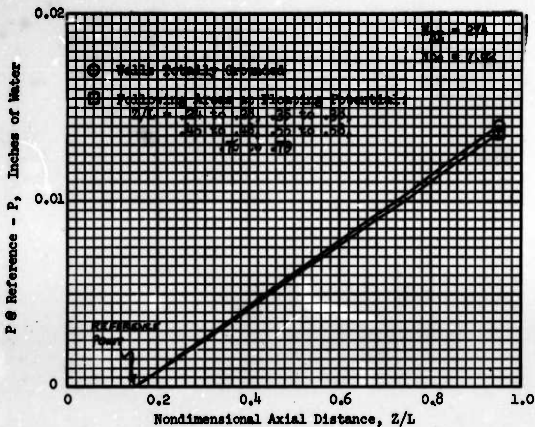
Fig. 33 - Static pressure on upper wall versus axial distance Z/L showing effect of discontinuous electric field along the duct
