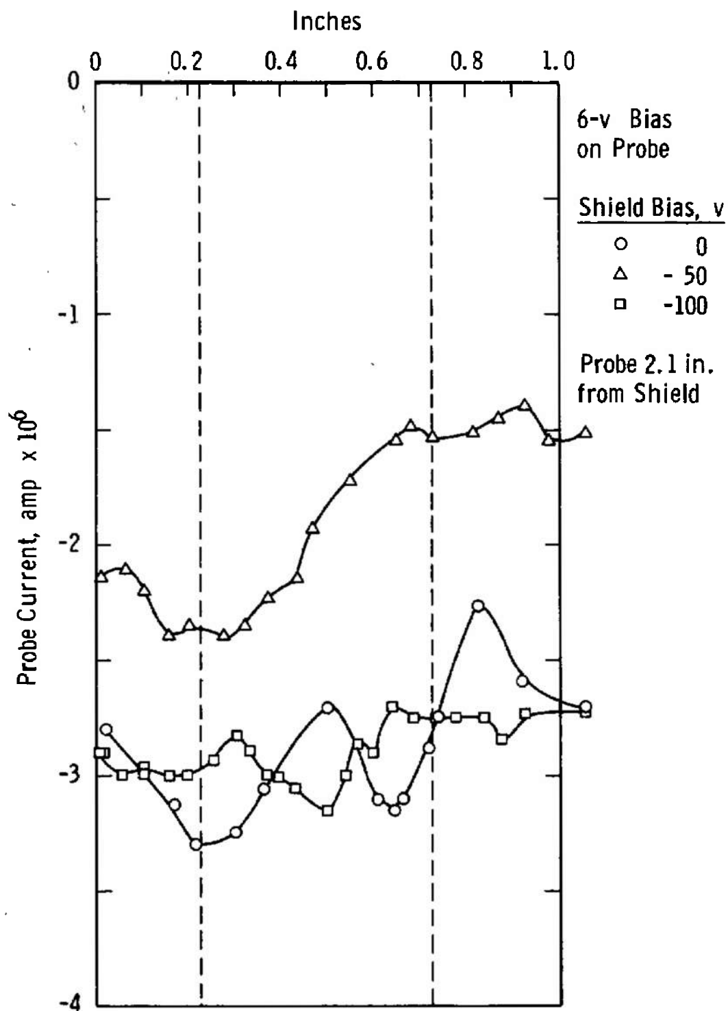
Fig. 48 Current Distribution Collected by Probe Biased 6.0 v (Shield 2.1 in. from Probe)
