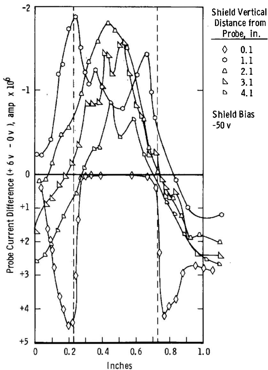
Fig. 52 Probe Current Difference ( -50\text{ v} on Shield)
