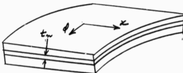
Fig. 13 Layered Shell
