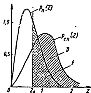
Fig. 6.3. Curves of the conditional probability densities p_p(Z) and p_{sp}(Z) corresponding to the detection of a signal with random initial phase.
