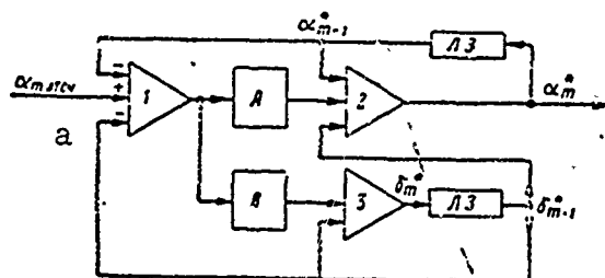
Fig. 8.5. Circuit scheme of the device for obtaining consecutive optimum estimates in the smooth regime in presence of independent and stationary second increments of the measured value \alpha . a) отсч.
