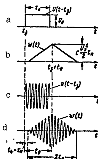
Fig. 4.9. Diagrams showing the envelopes and instantaneous values of a useful signal at the input and output ends of an optimum filter for a rectangular radio pulse with constant carrier frequency.
