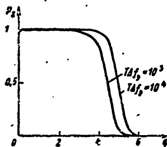
Fig. 6.15. Curves of the unreliability coefficient P_2 = P_2(q) for two values of the produce T\Delta f_e .
