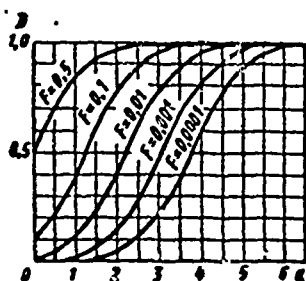
Fig. 6.2. Detection curves for a signal with completely known parameters.
