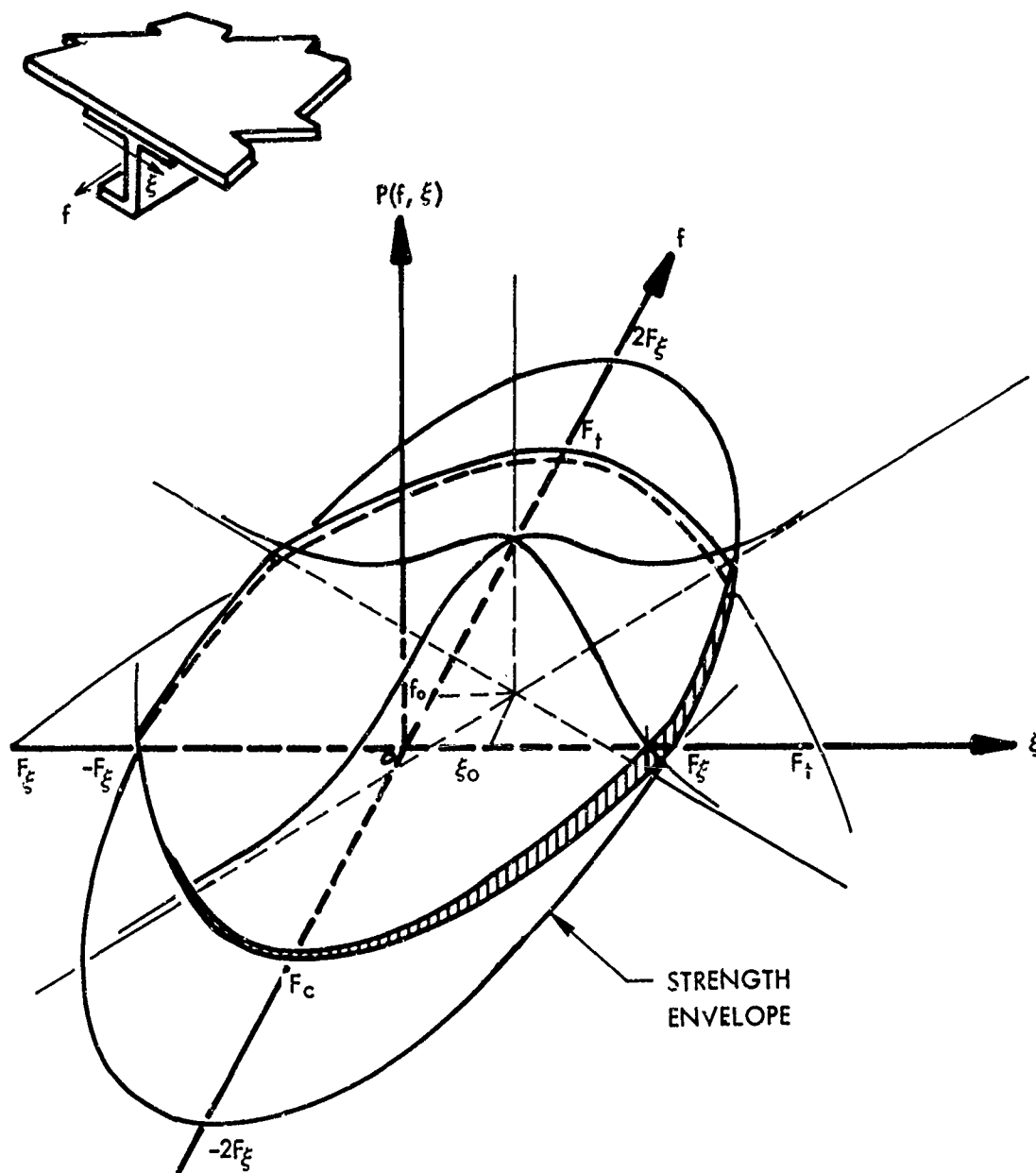
FIGURE 14. JOINT GAUSSIAN PROBABILITY DENSITY FUNCTION
