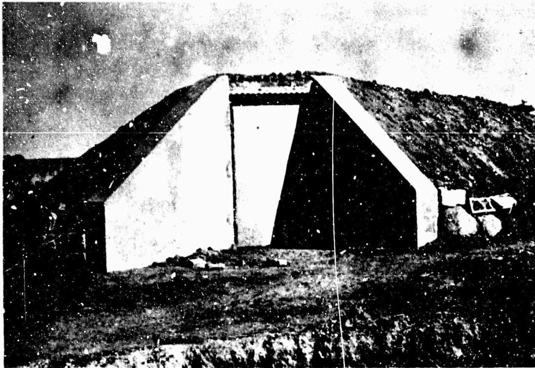
Figure 9. The exterior of the long period vault at the main station at Abéché.
